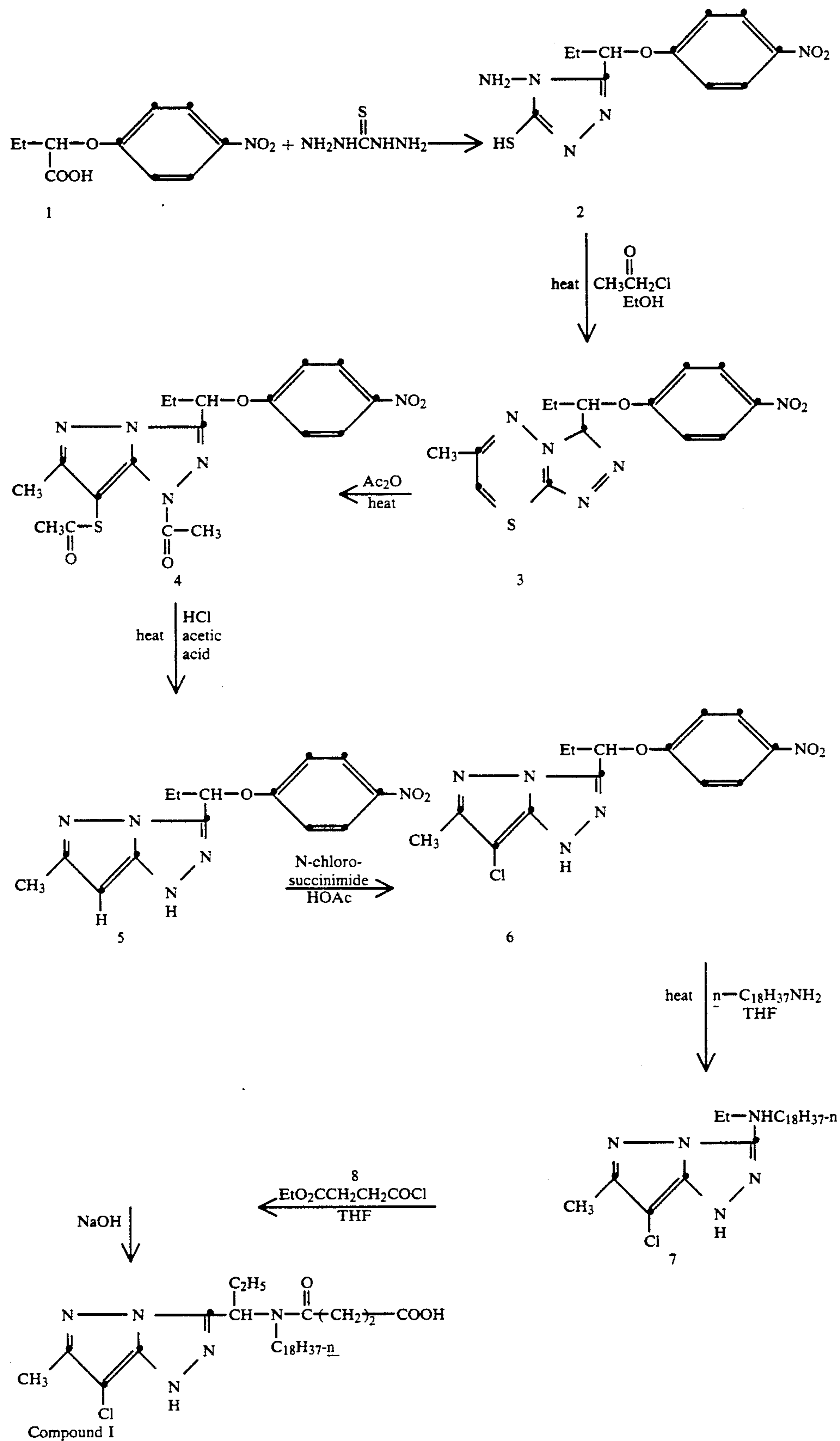
Scheme I
