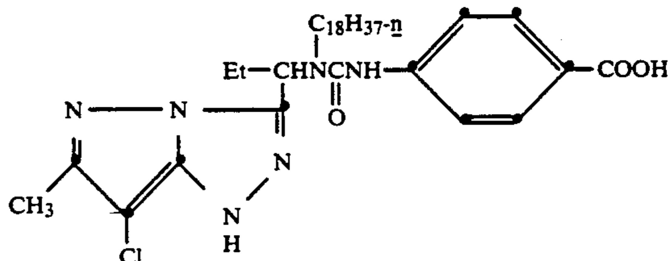
Compound III
