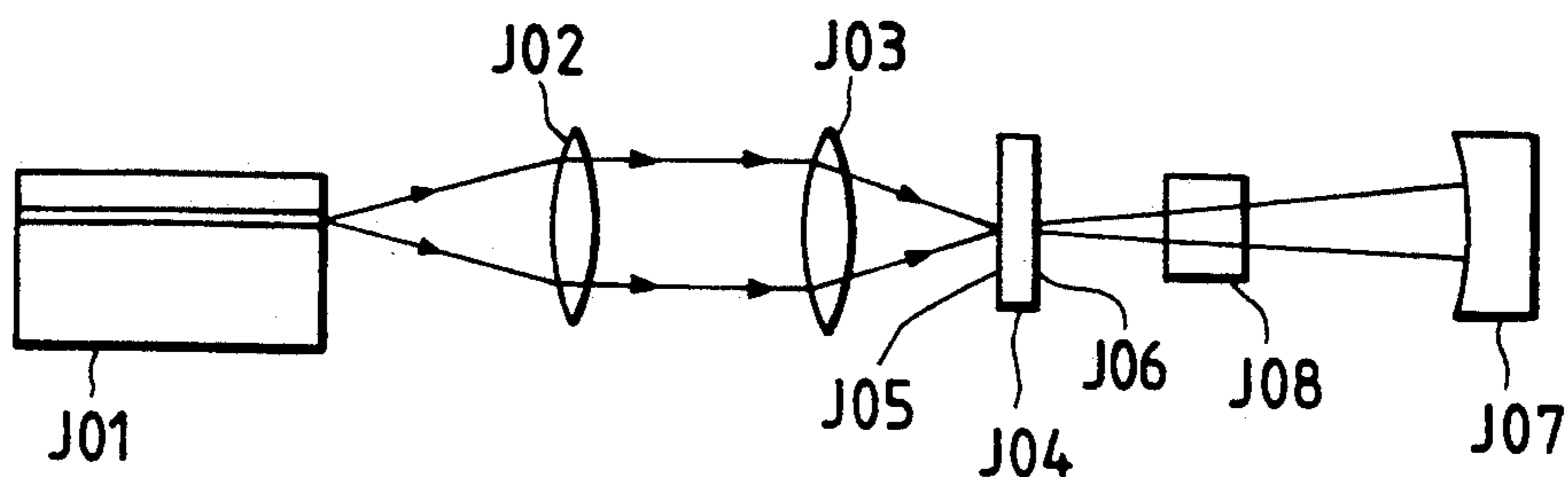
FIG. 19 PRIOR ART
