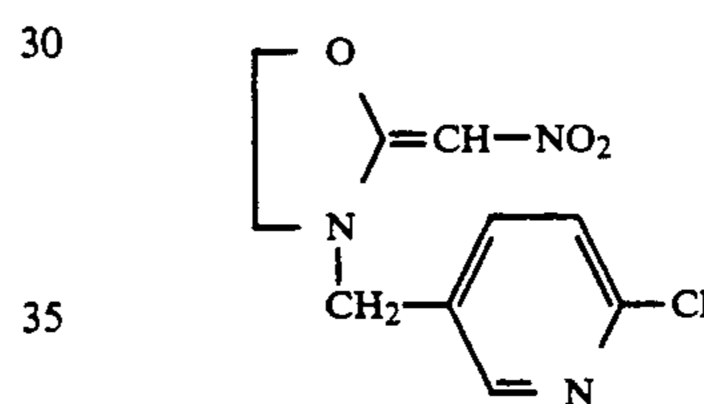
(Compound No. 14)
