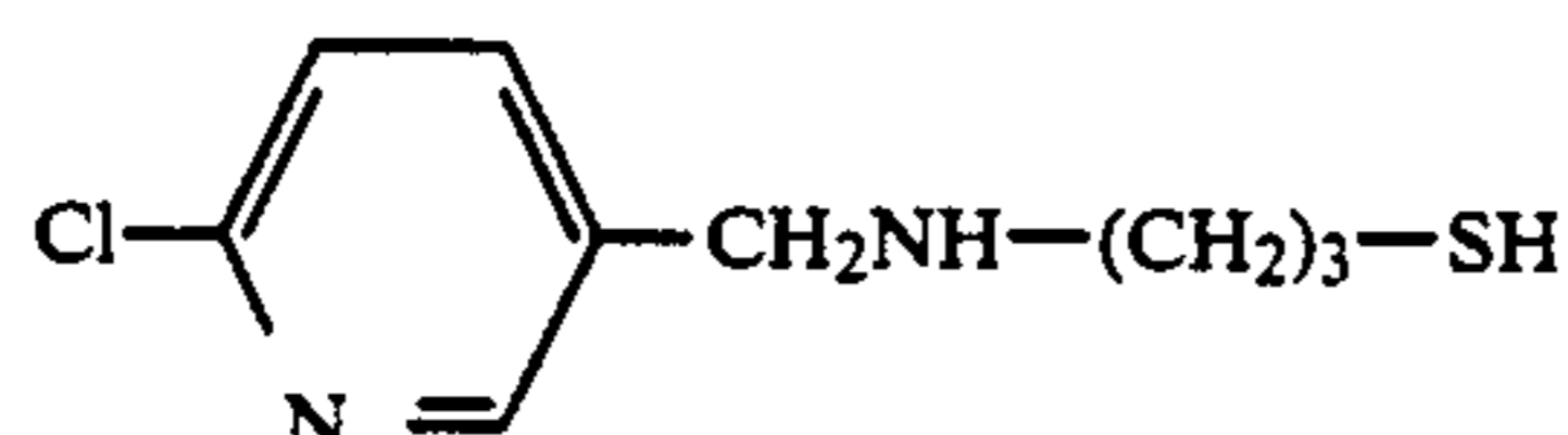
N-(2-chloro-5-pyridylmethyl)3-aminopropanethiol
