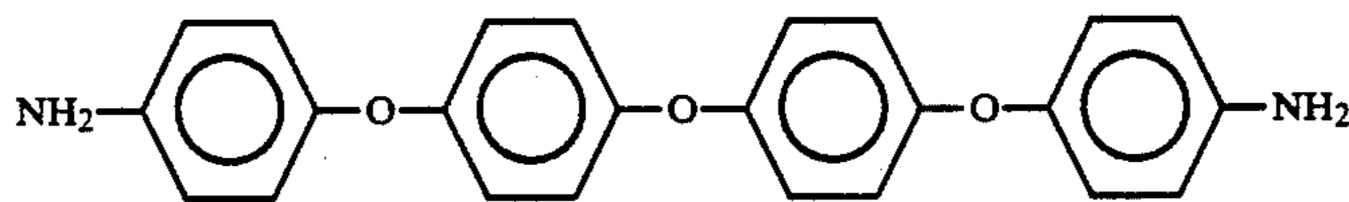
BAPE
