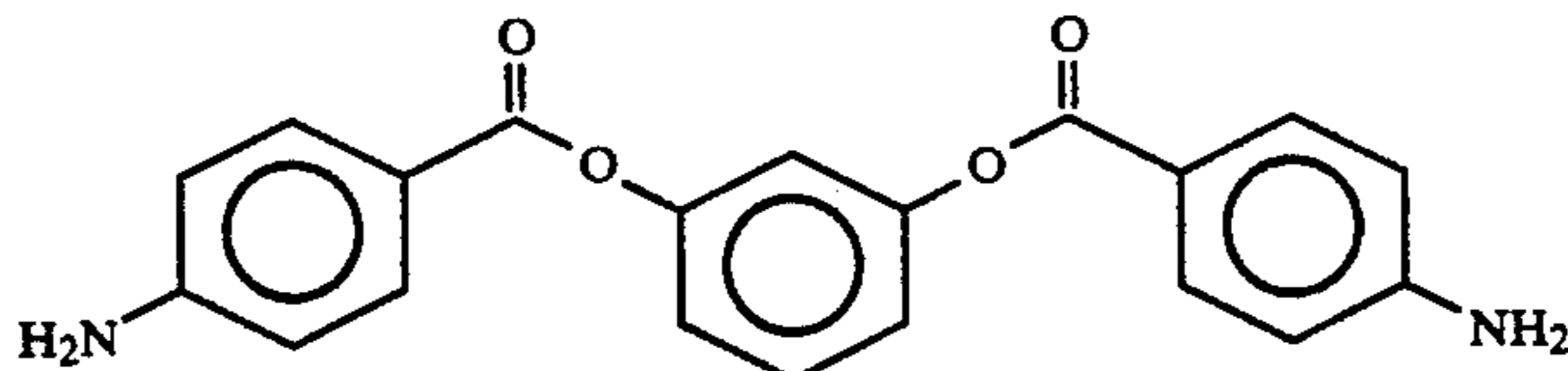
RDEDA
