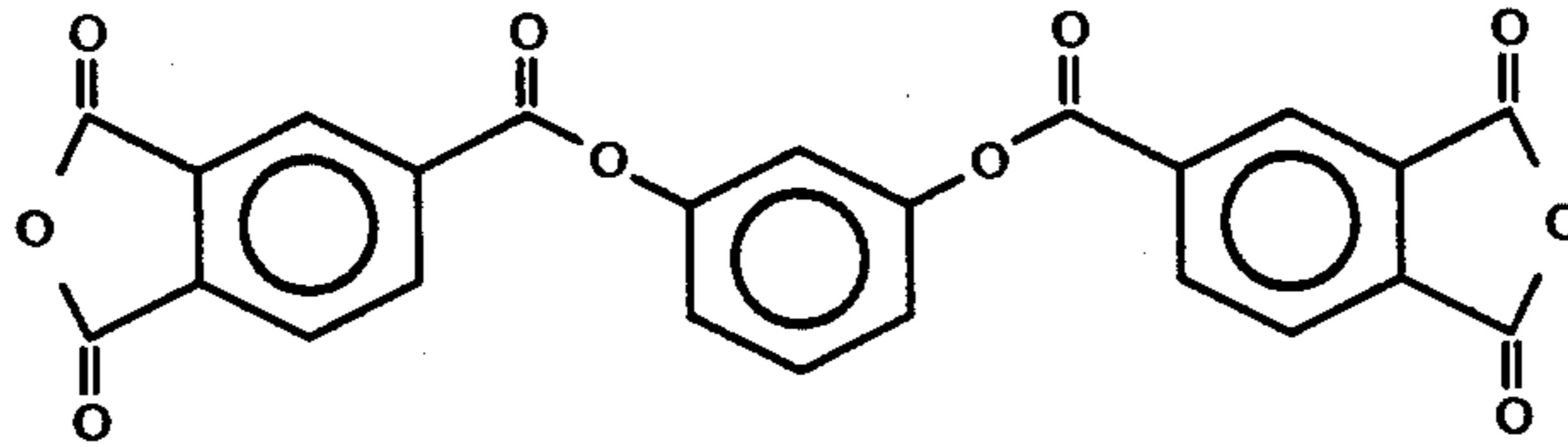
MPBTDA
