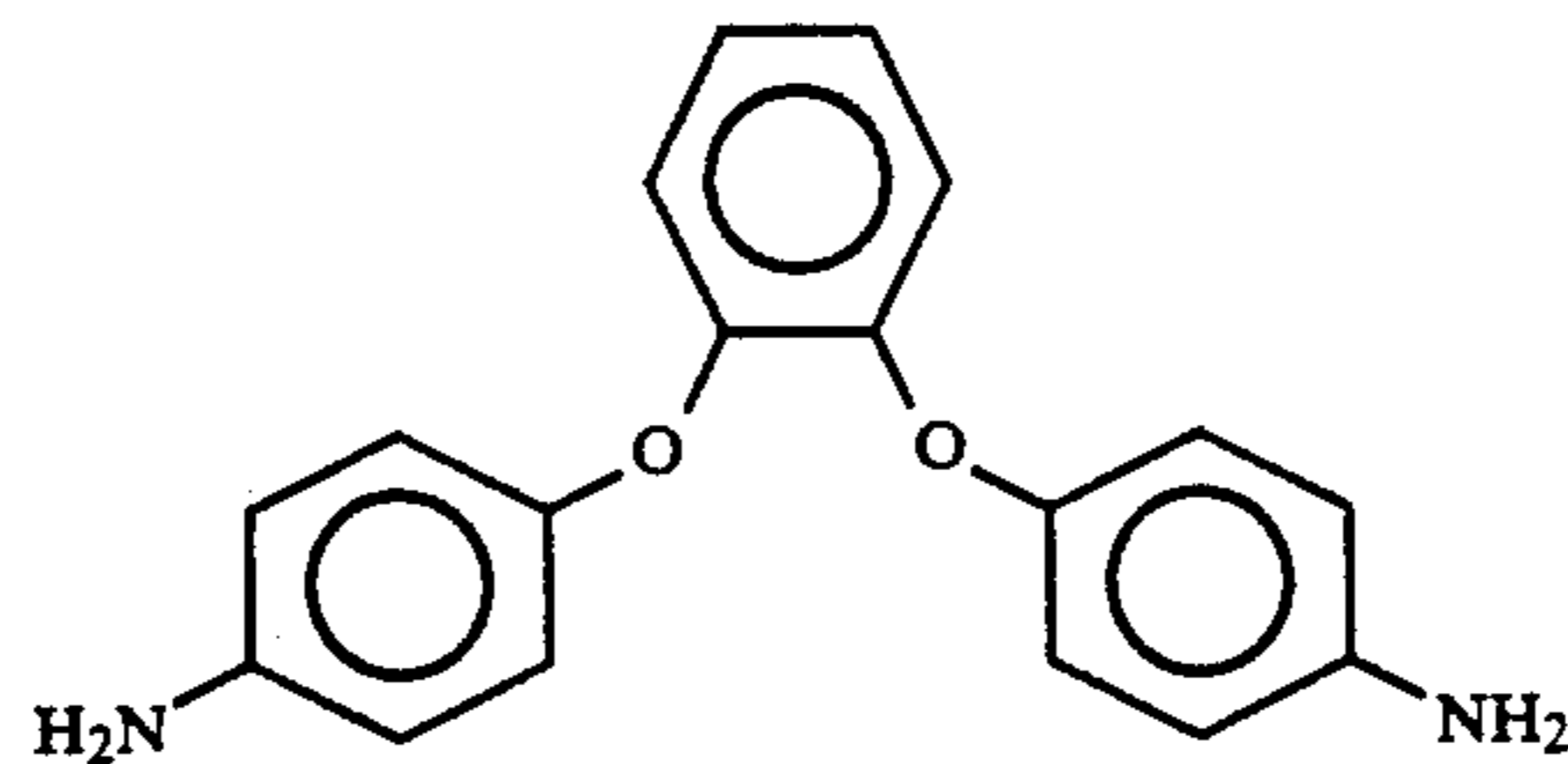
CODA
