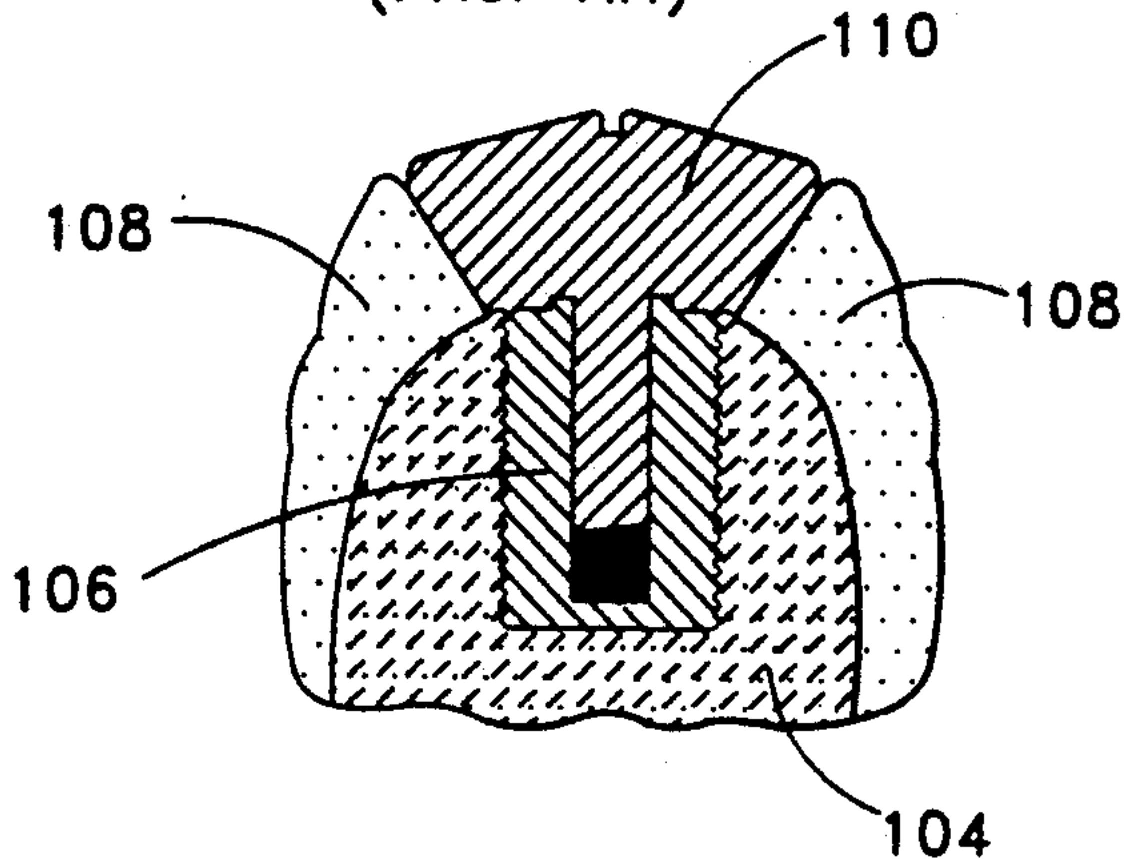
FIG. 1 (Prior Art)
