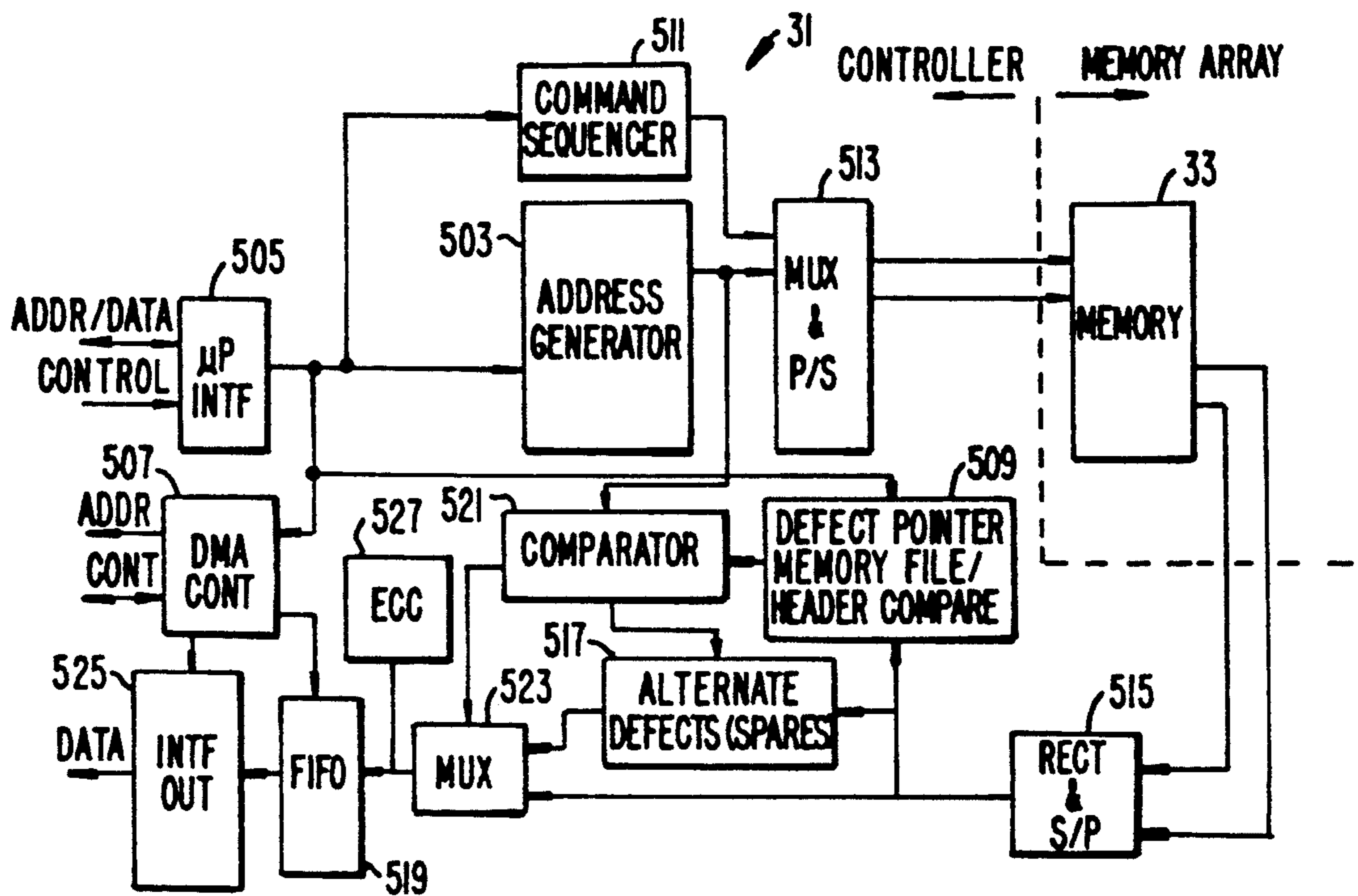
READ DATA PATH CONTROL
