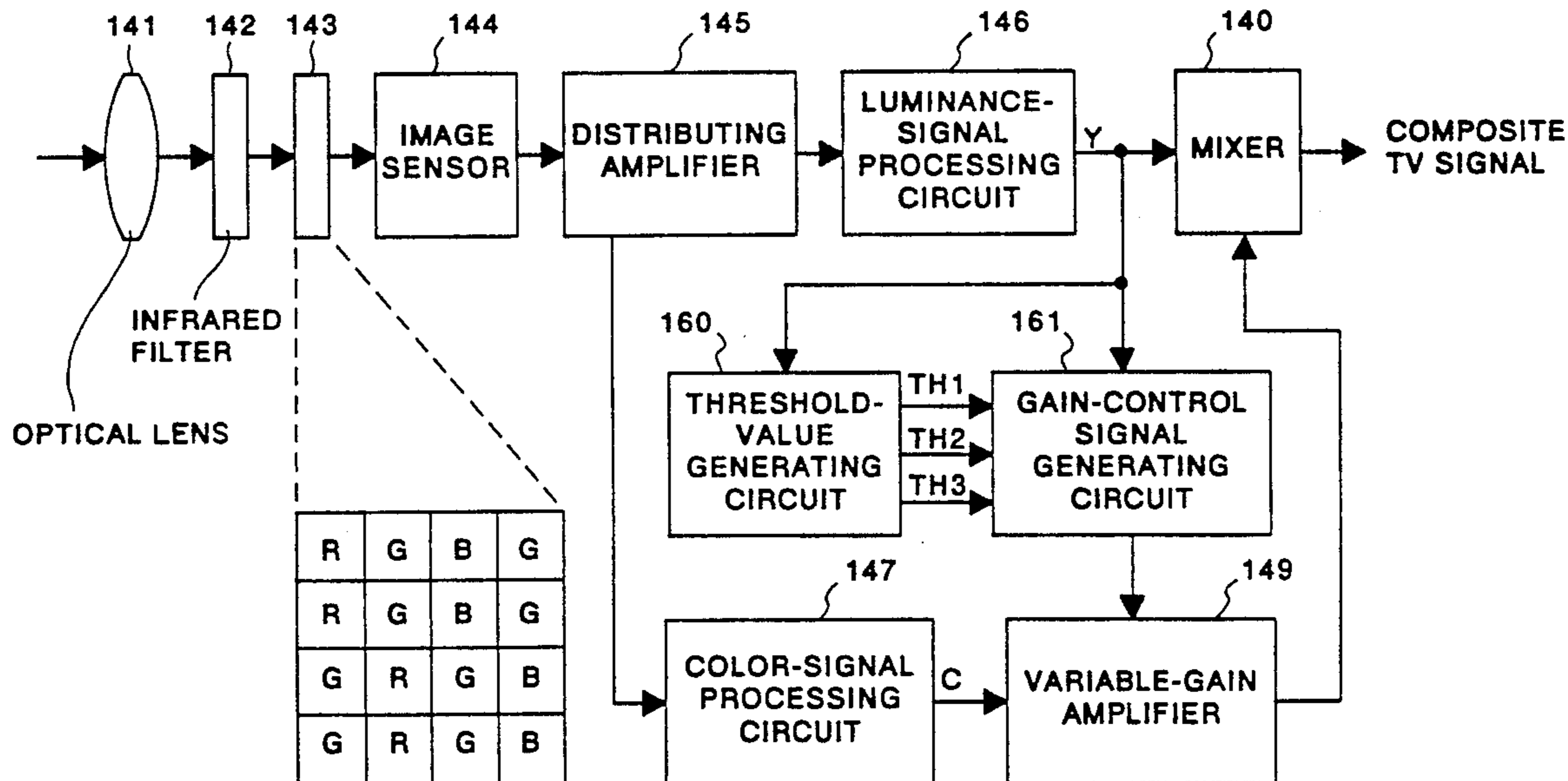
(EXAMPLE OF COLOR-FILTER ARRAY)
