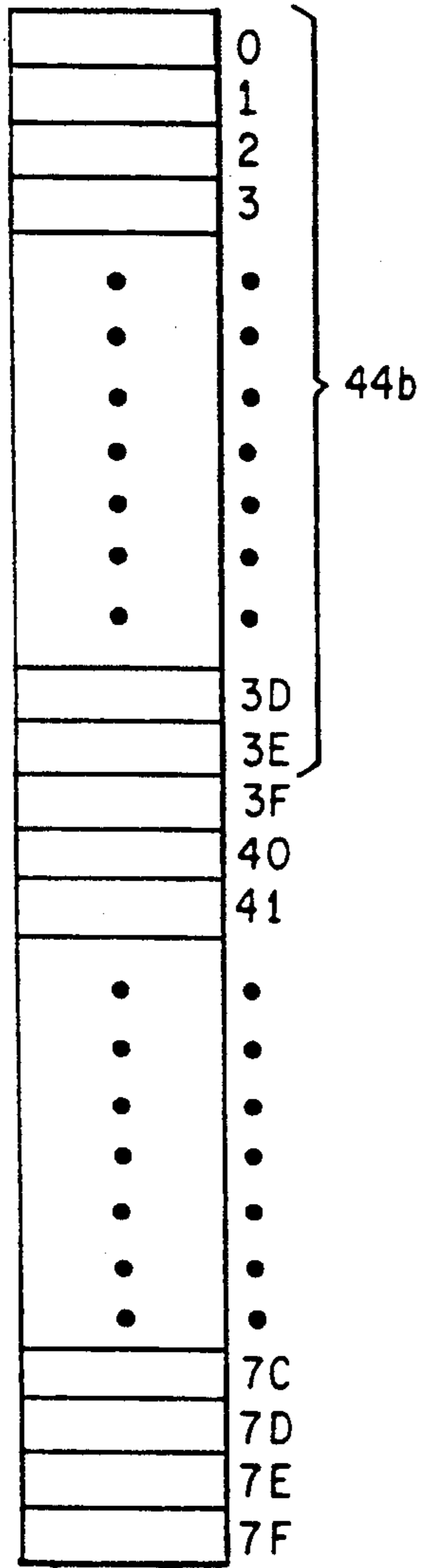
REGISTER FILE 0 OR 1 Fig. 44a
