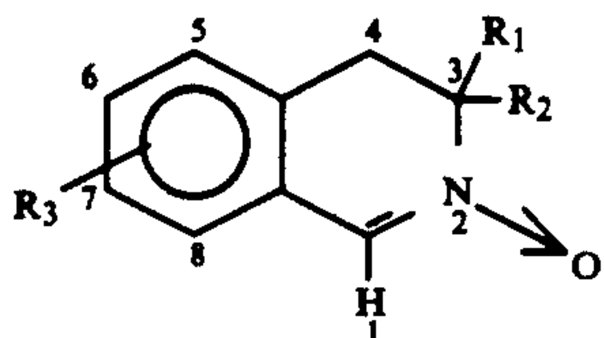
Formula I, n = 1 isoquinoline (3,4-dihydro)-N-Oxide
