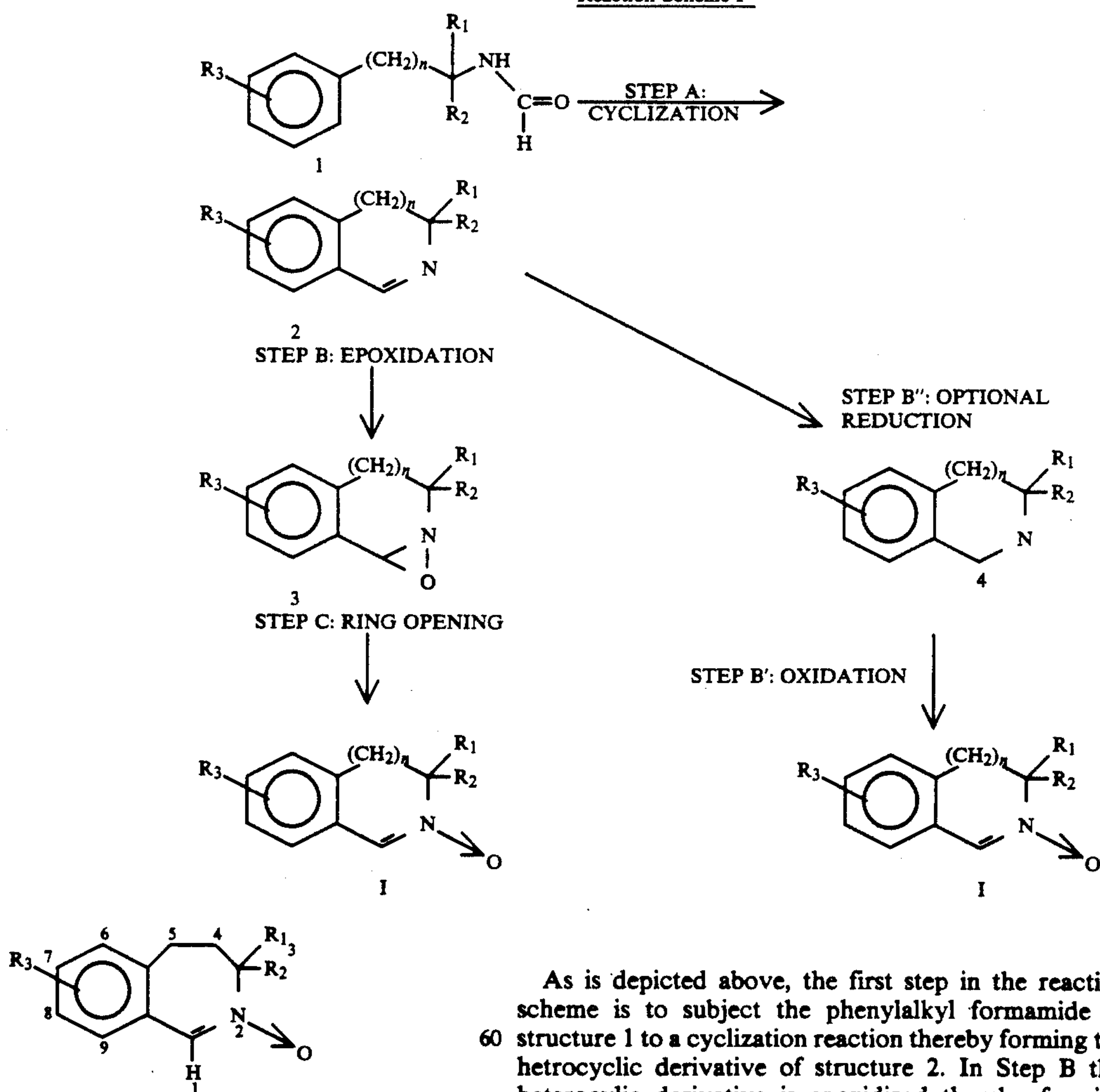
Formula I, n = 2 dihydrobenzazepine-N-oxide
