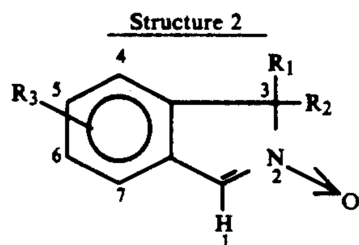
Formula I, n = 0 isoindole-N-oxide
