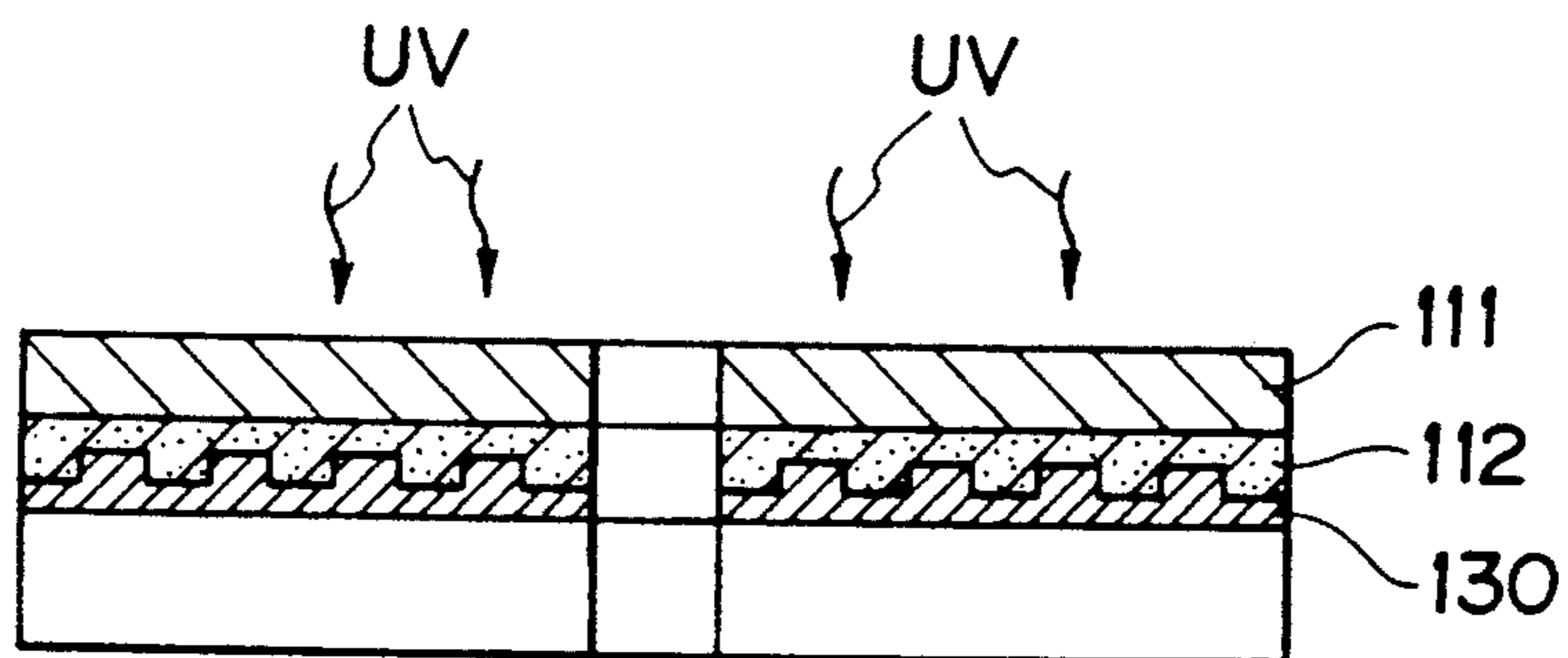
FIG. 8 PRIOR ART
