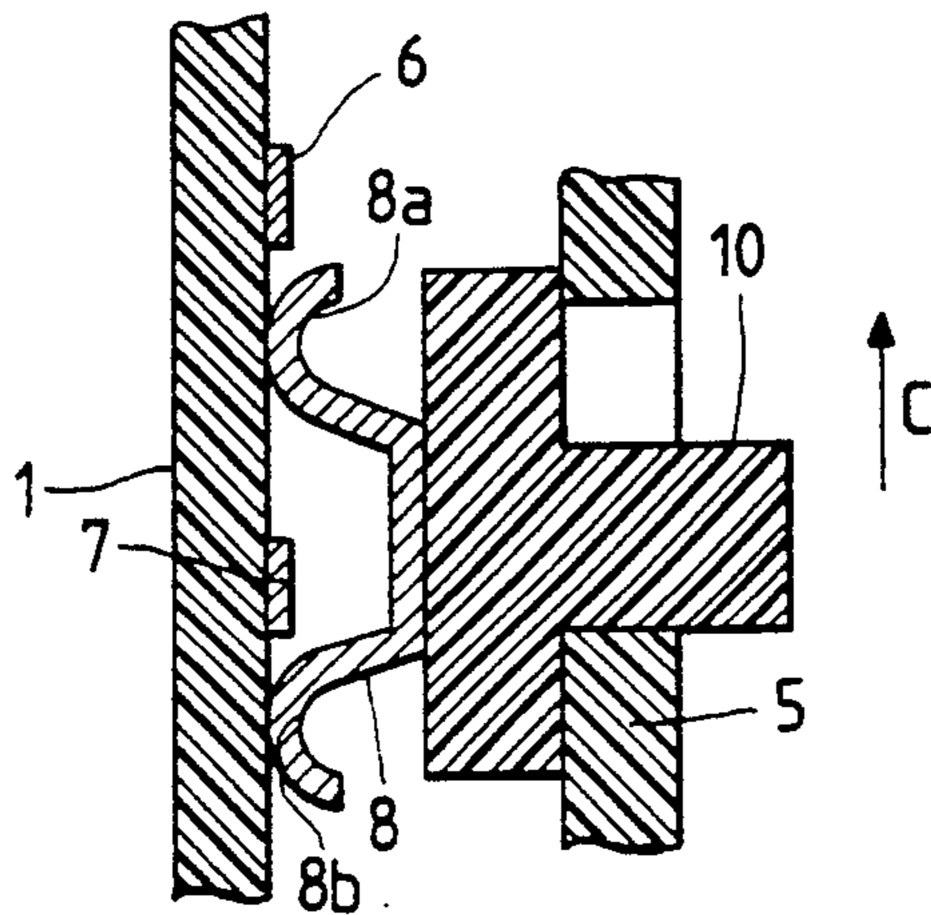
FIG. 3C PRIOR ART
