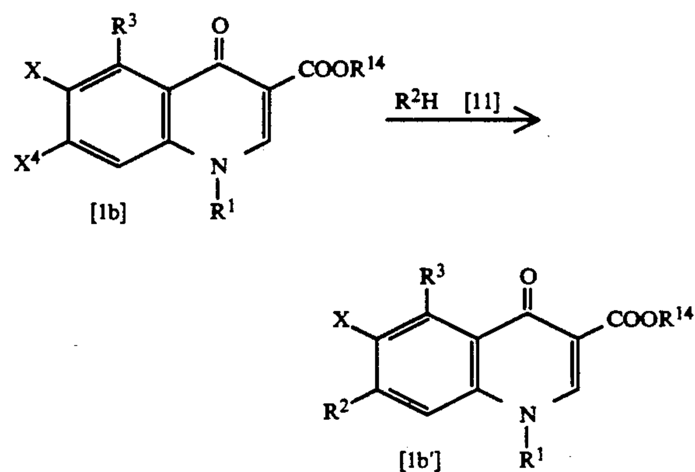
[Reaction Scheme-II]
