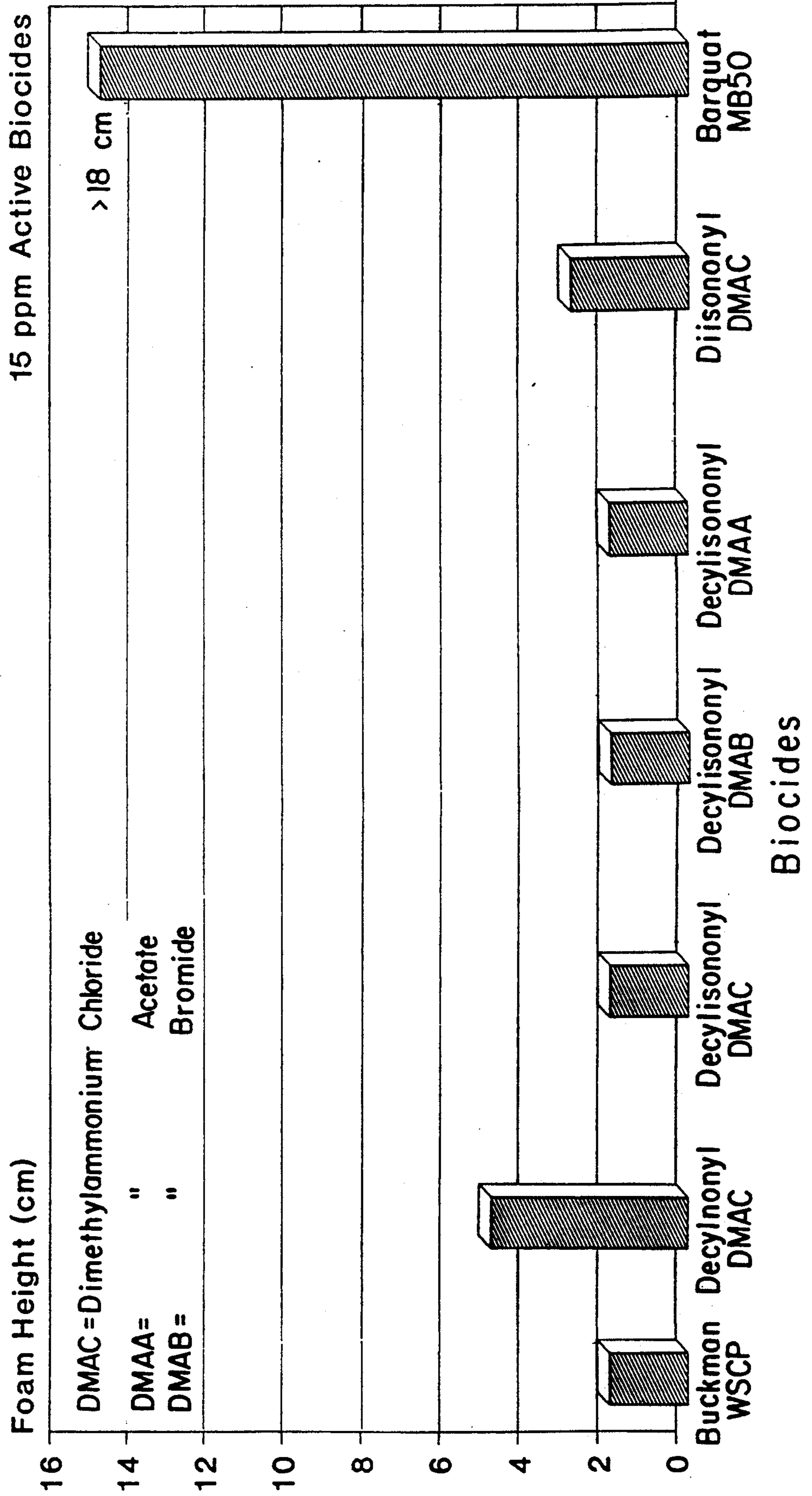
FIG. 6 - CIRCULATION FOAM TEST EQUILIBRIUM FOAM HEIGHT
