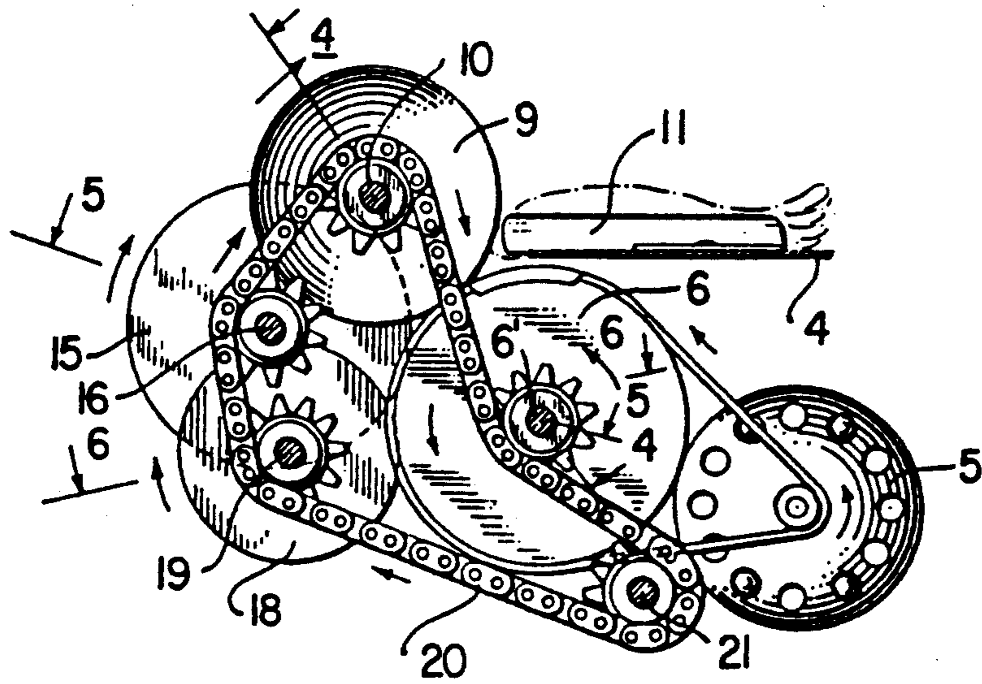
FIG. 3 (PRIOR ART)
