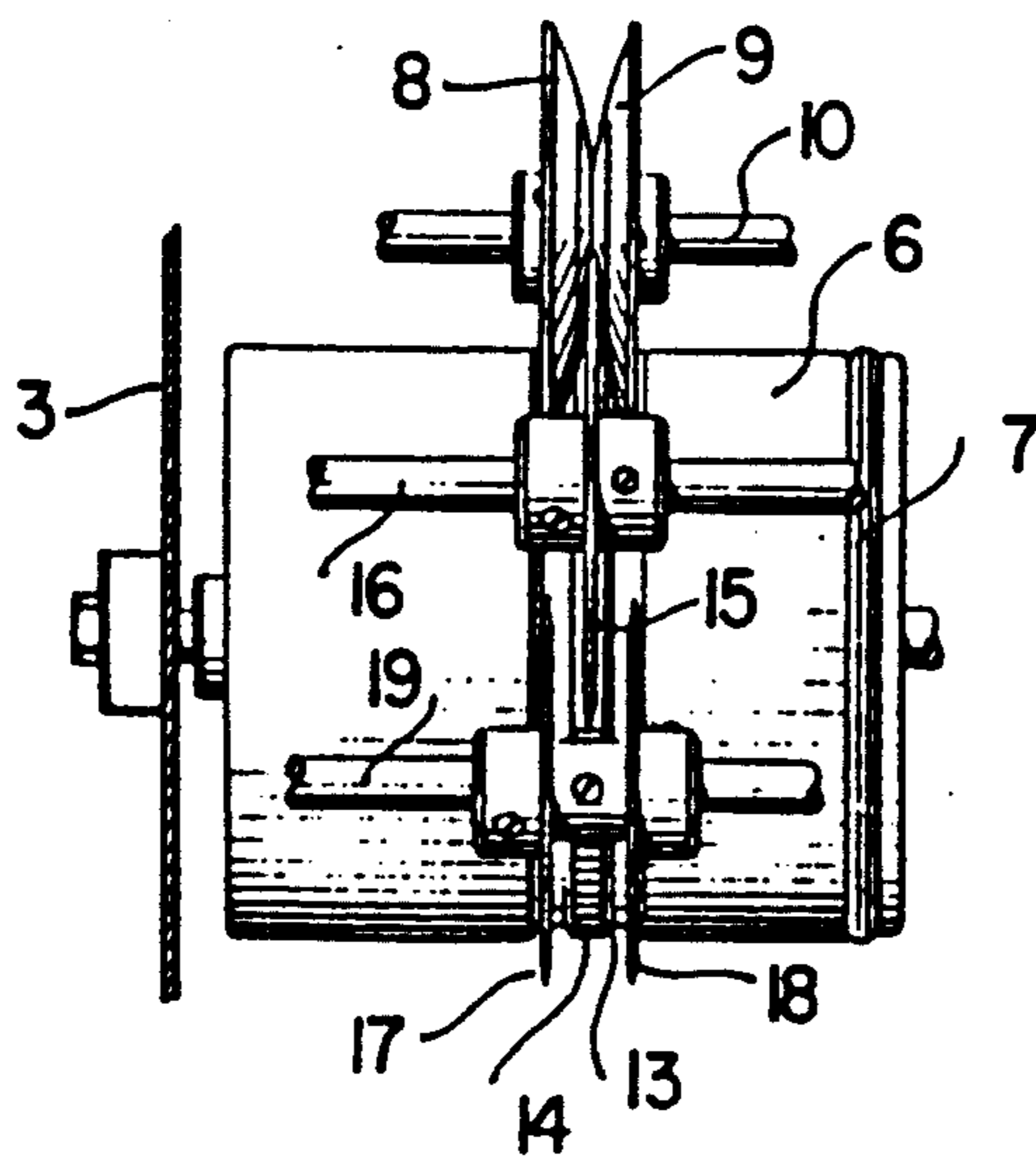
FIG. 4 (PRIOR ART)
