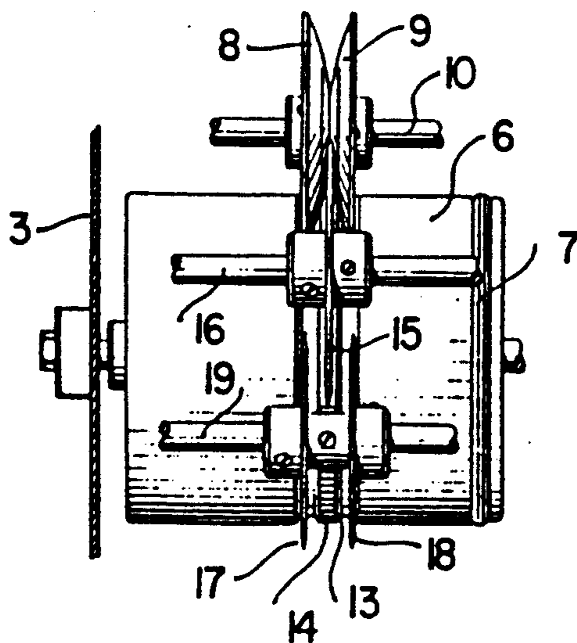
FIG. 4 (PRIOR ART)
