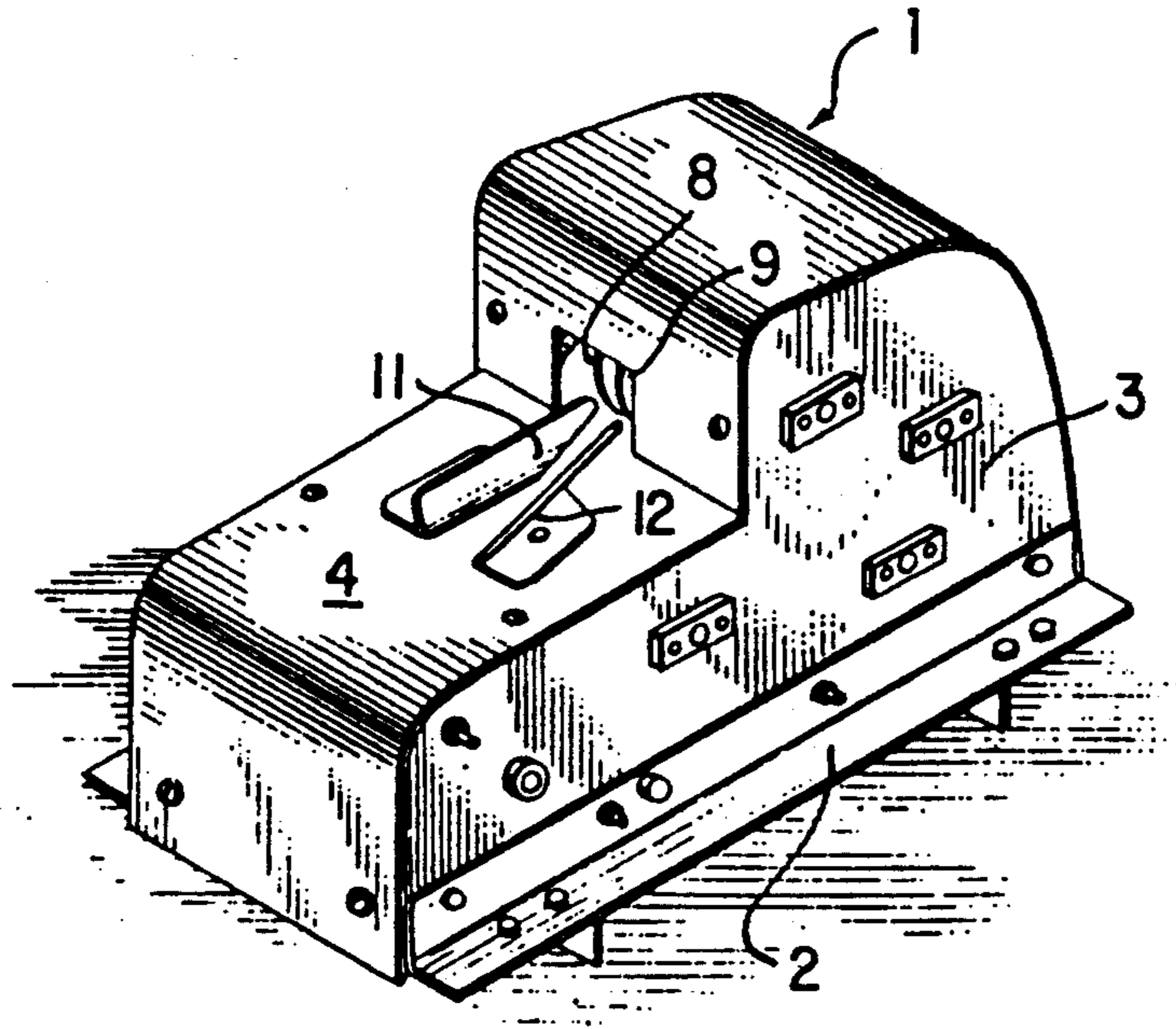
FIG. 1 (PRIOR ART)
