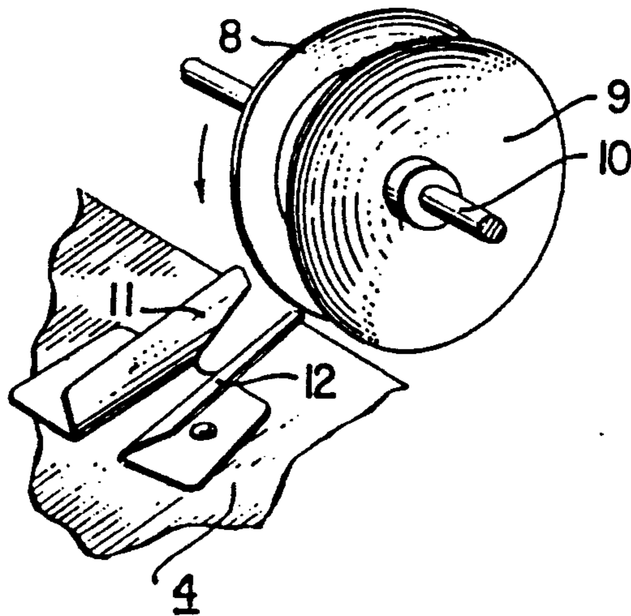
FIG. 2 (PRIOR ART)
