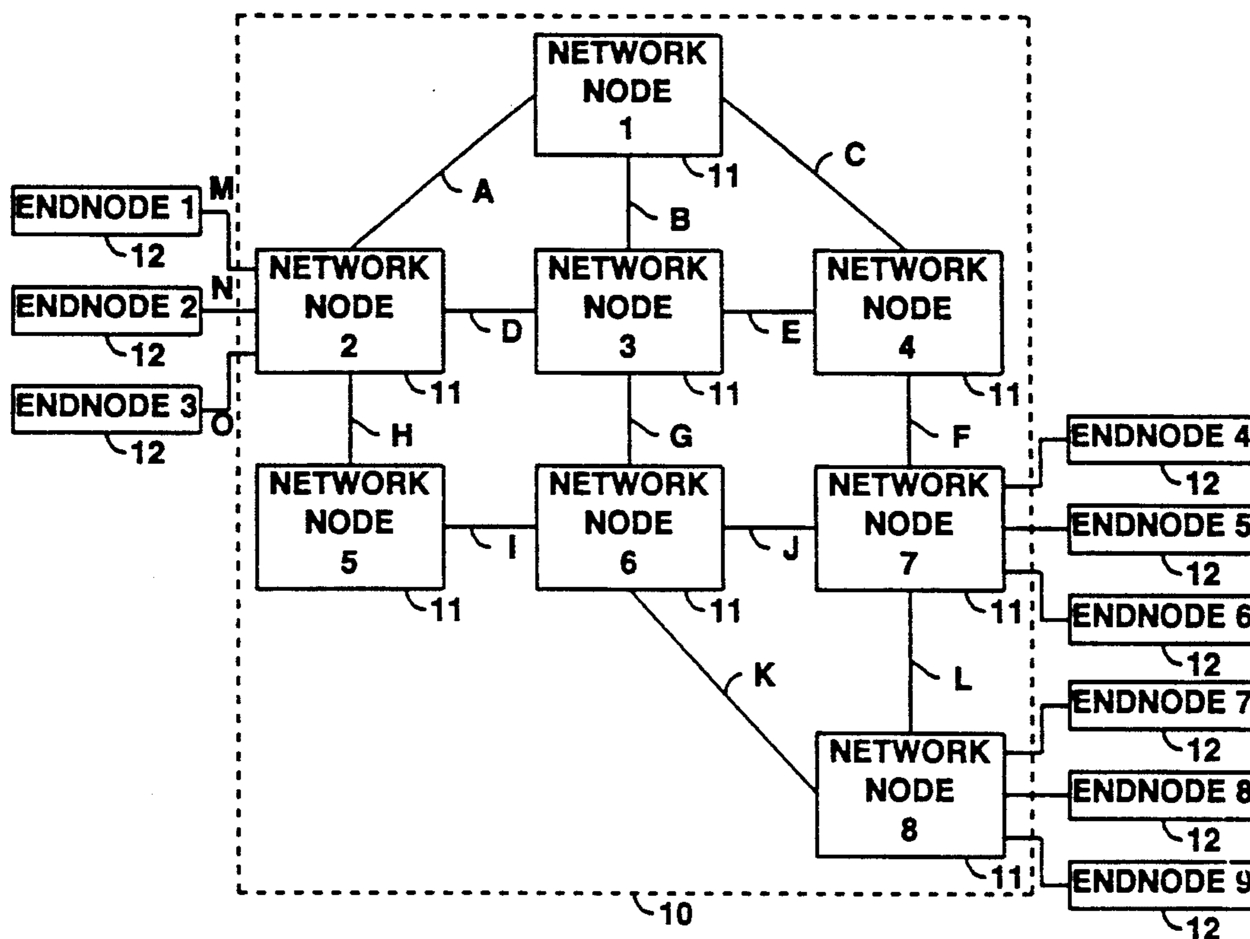
FIG. 1 COMMUNICATIONS NETWORK
