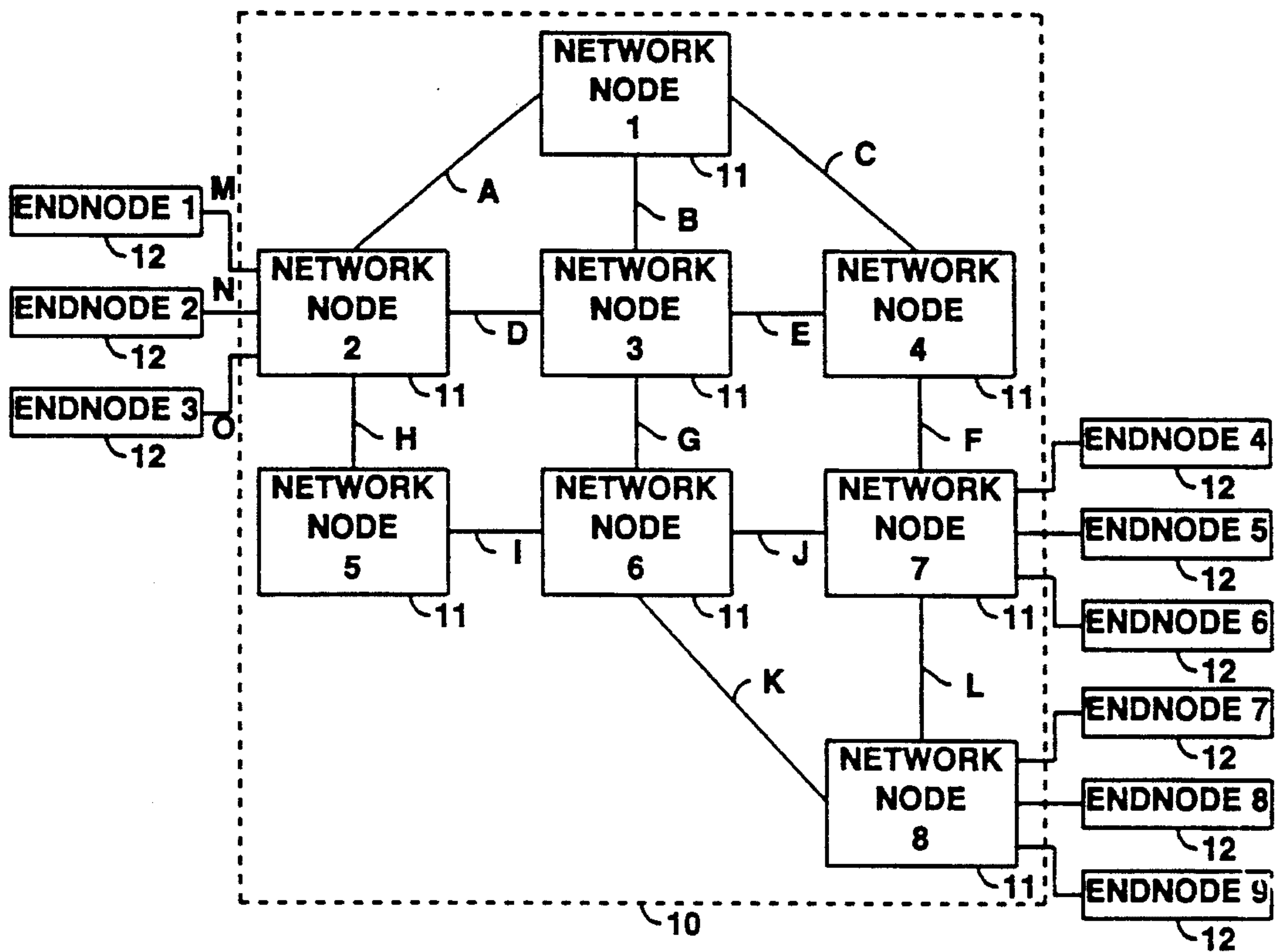
FIG. 1 COMMUNICATIONS NETWORK
