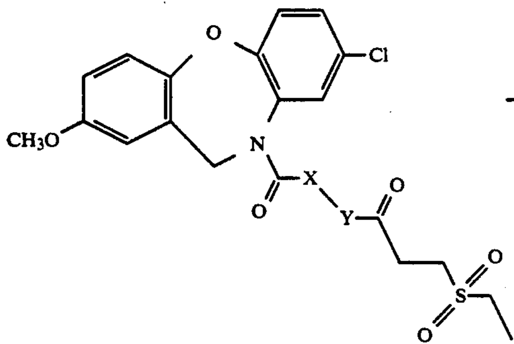
GENERAL REACTION SCHEME NO. 9)
