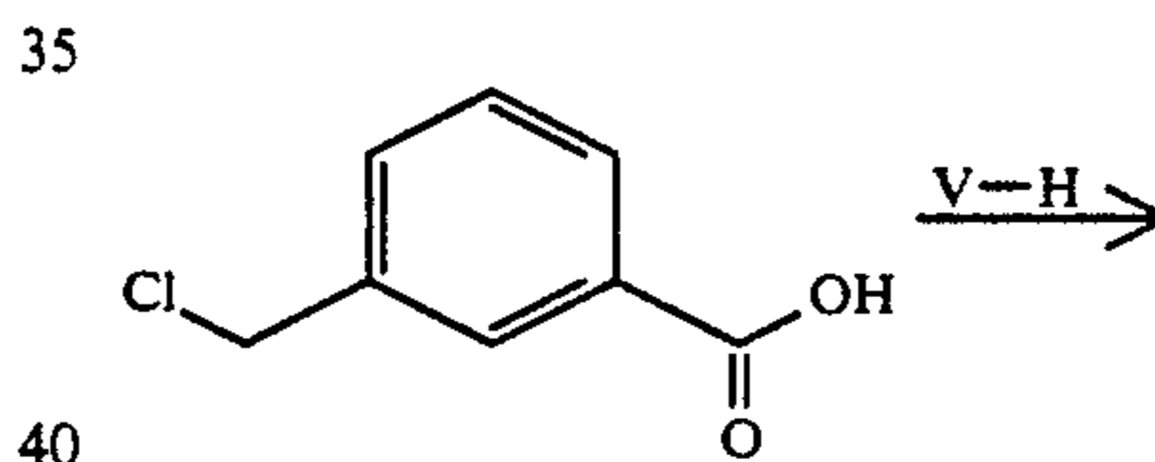
GENERAL REACTION SCHEME NO. 12
