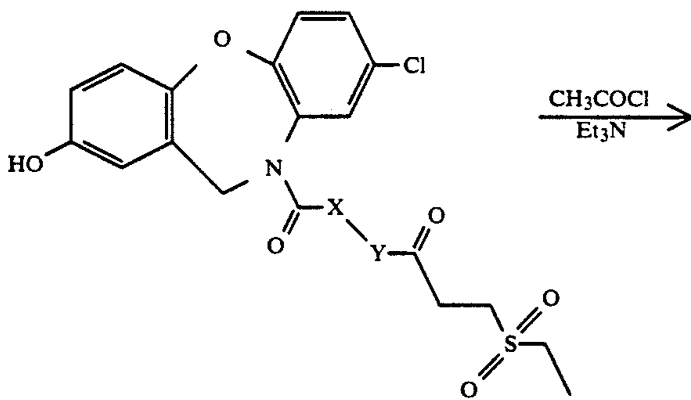
GENERAL REACTION SCHEME NO. 10
