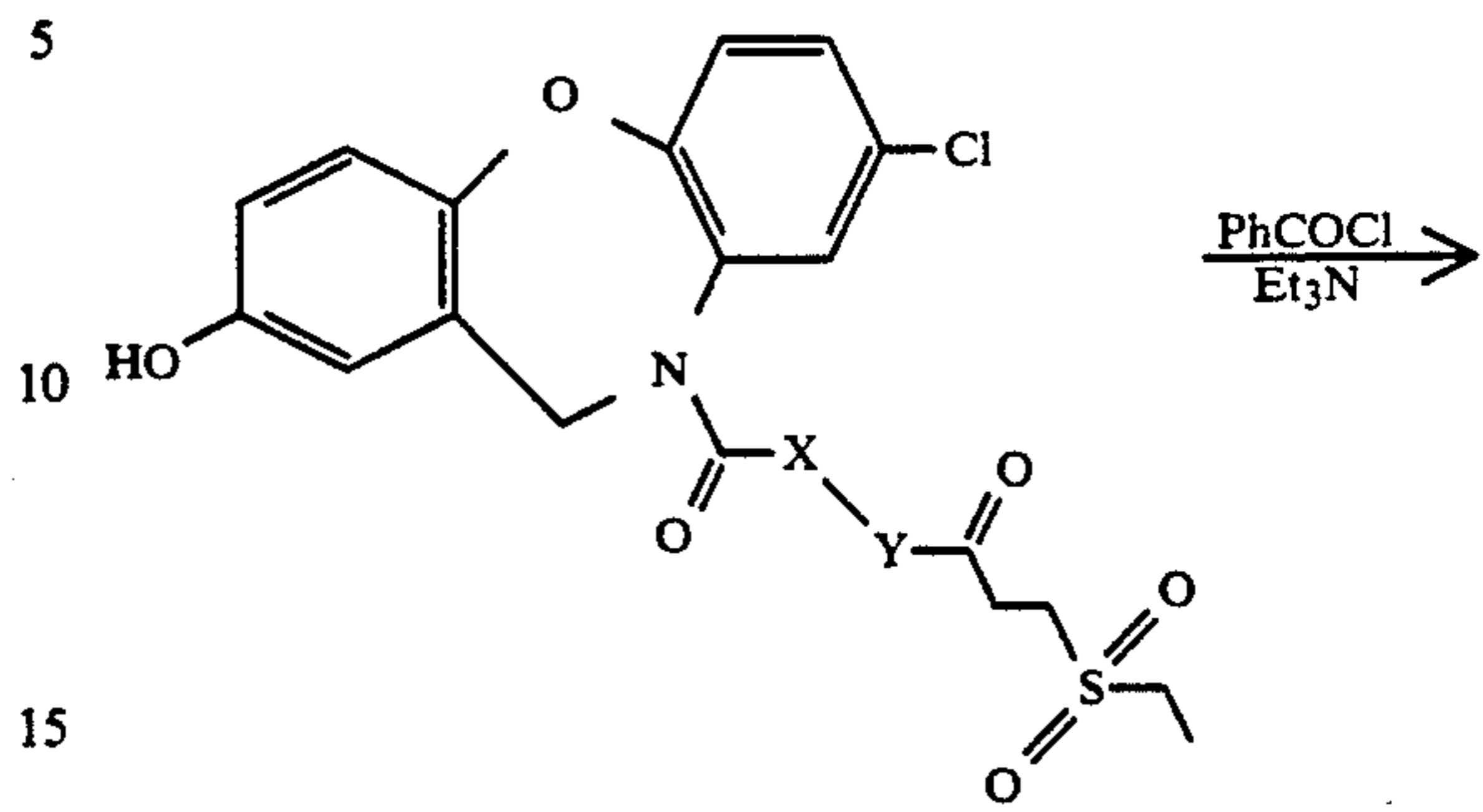
GENERAL REACTION SCHEME NO. 11
