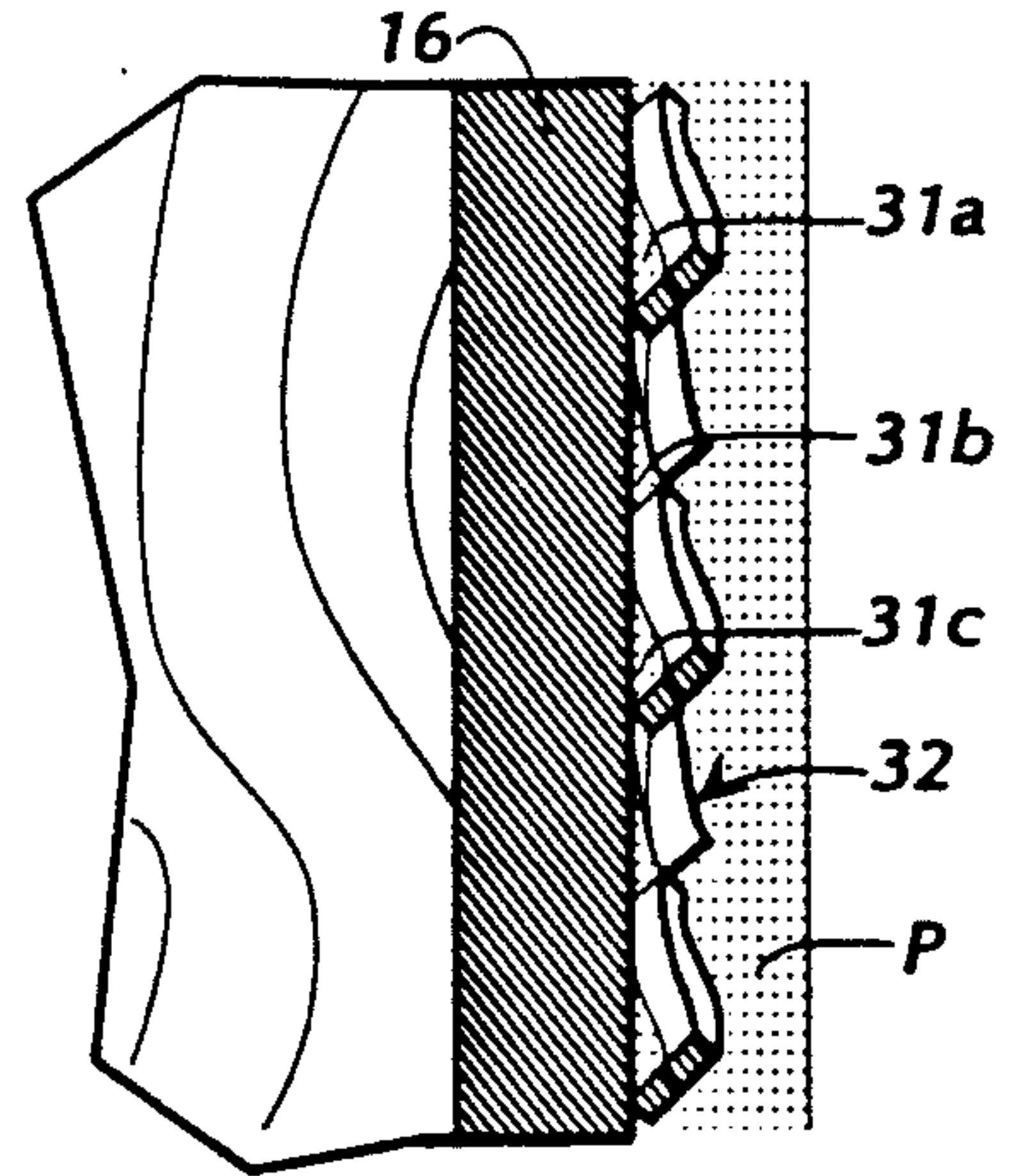
FIG 2 (PRIOR ART)
