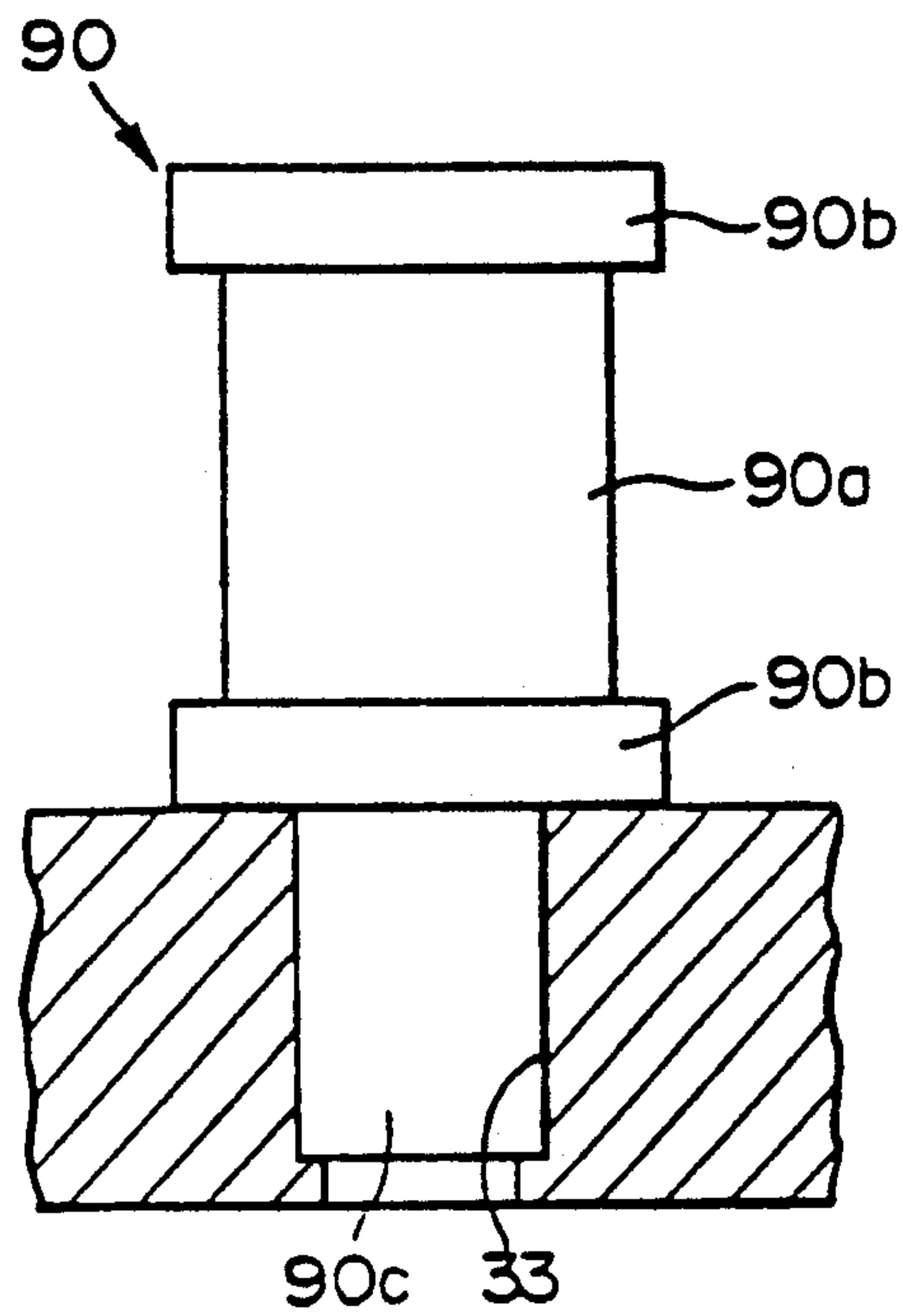
FIG. 1 (PRIOR ART)
