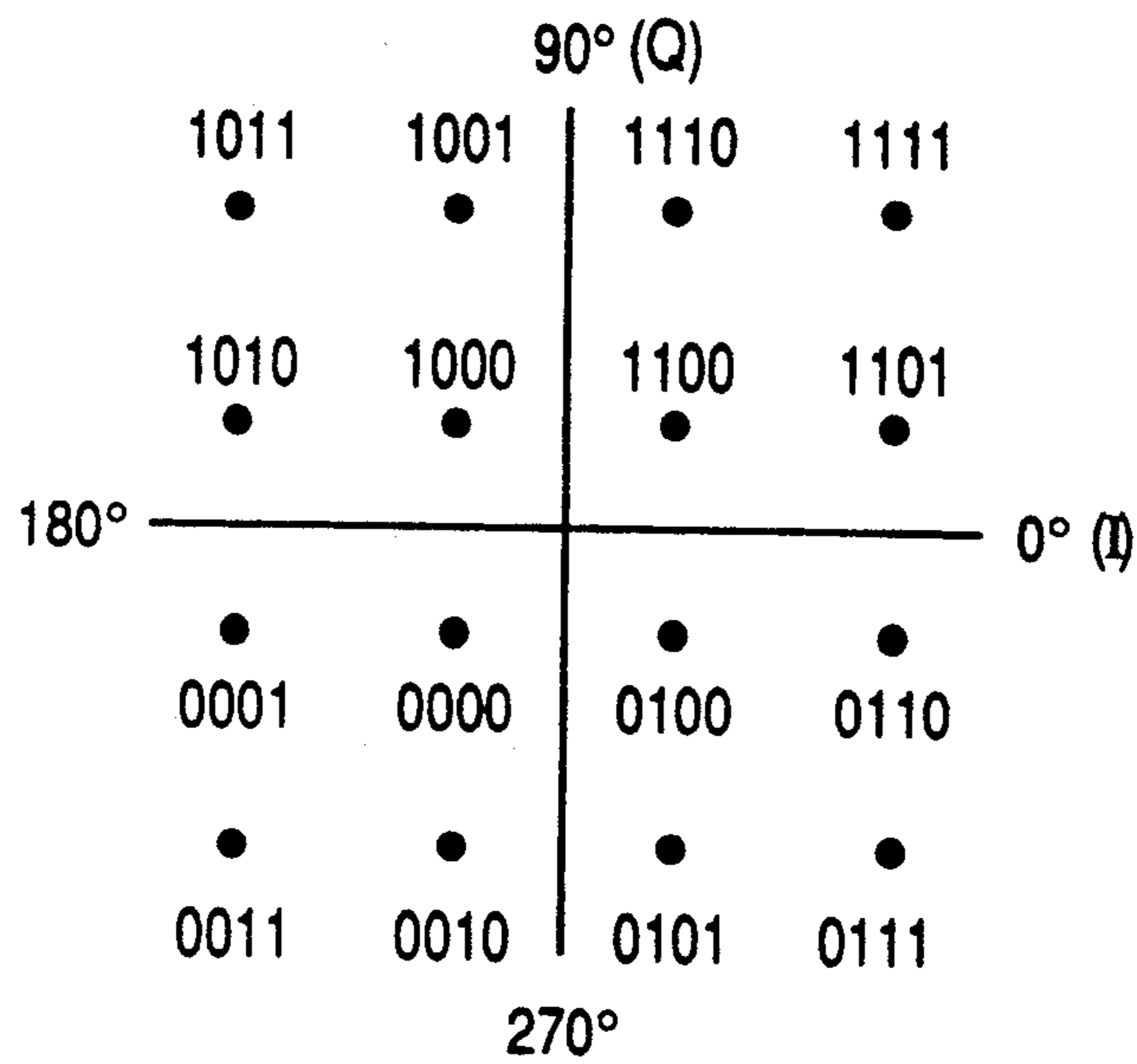
BIT ASSIGNMENT FOR 16-LEVEL QAM SIGNAL CONSTELLATION
