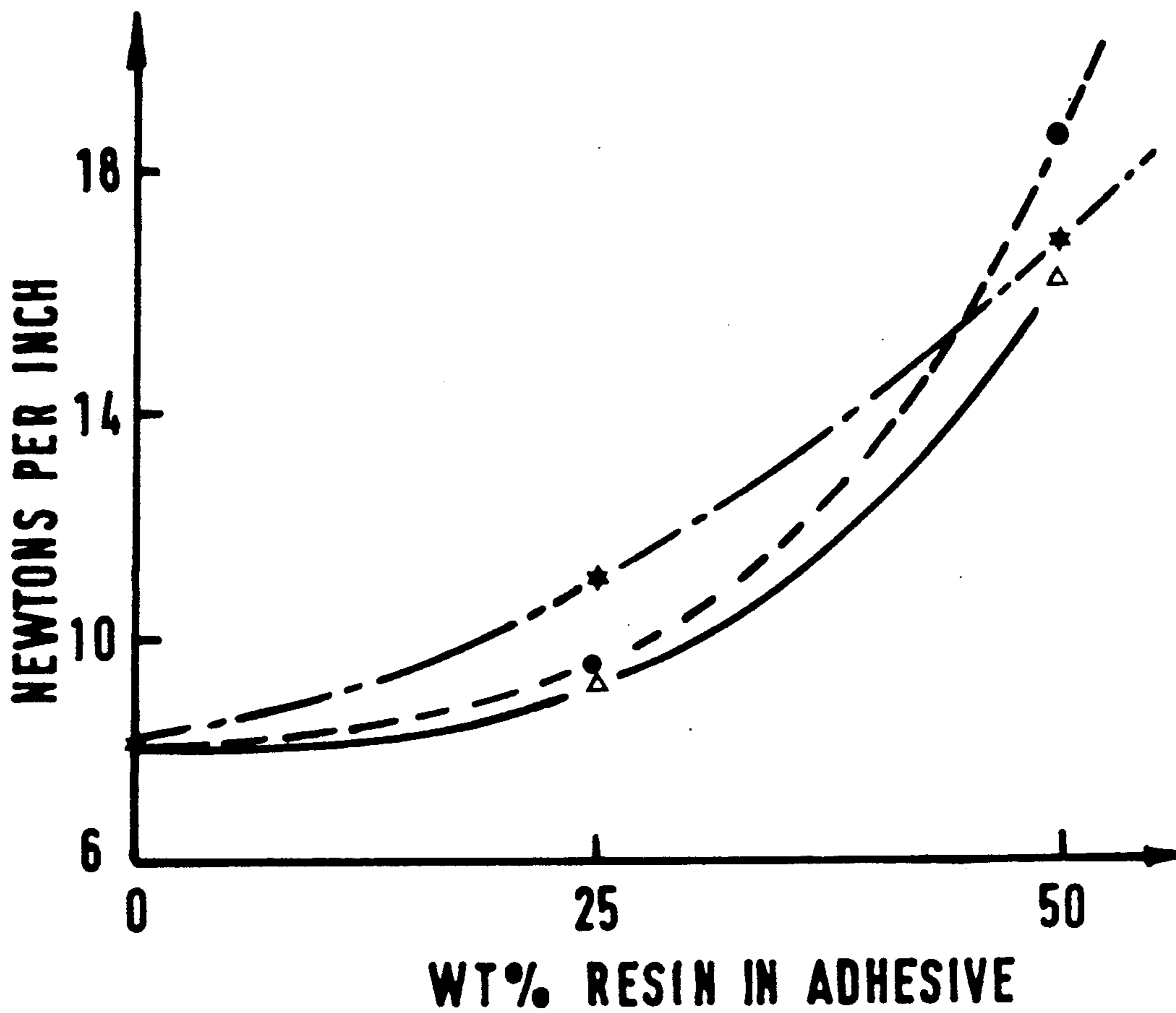
FIG. 1 PEEL STRENGTH
