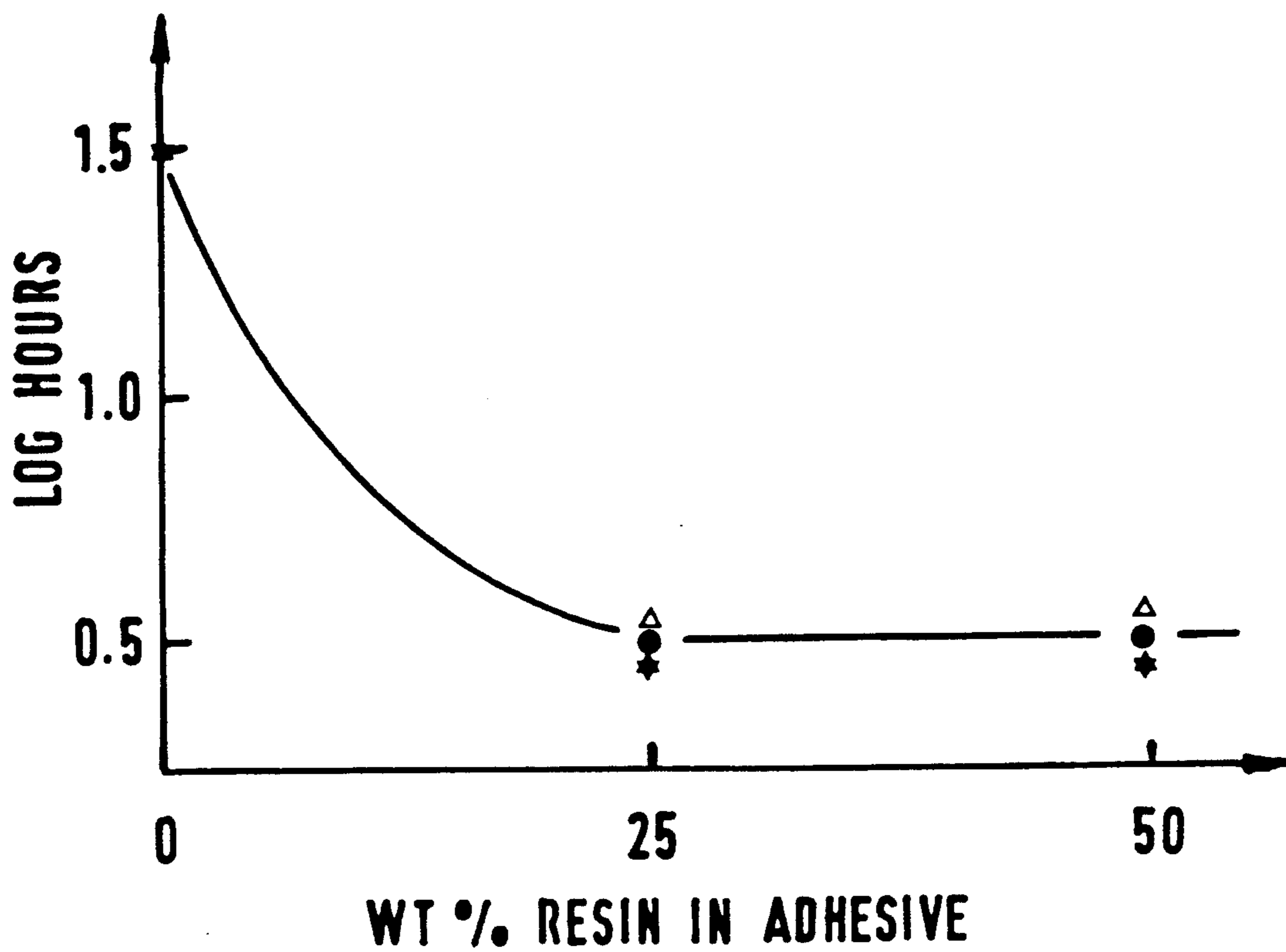
FIG. 6 SHEAR
