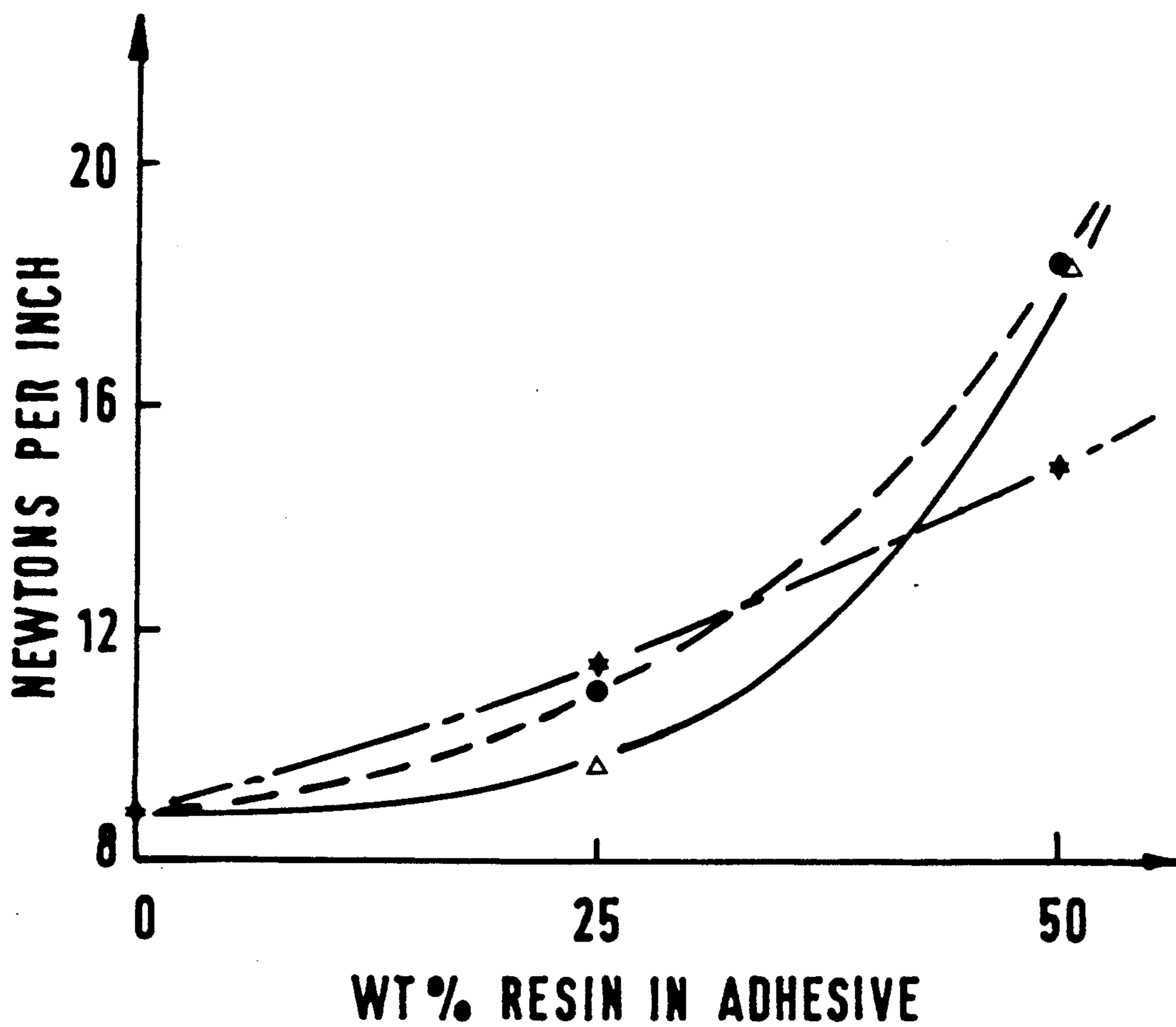
FIG. 5 LOOP TACK
