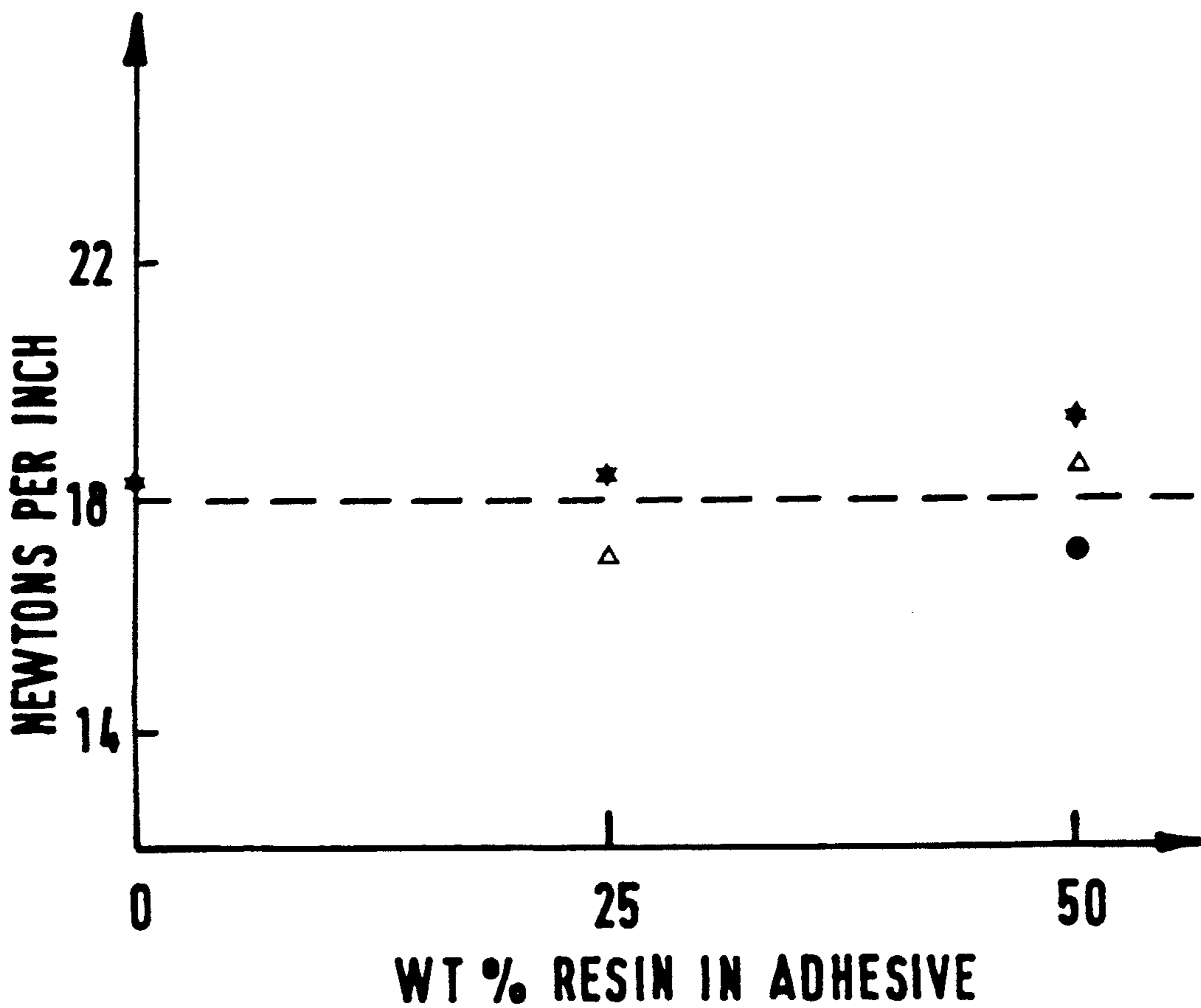
FIG. 4 PEEL STRENGTH
