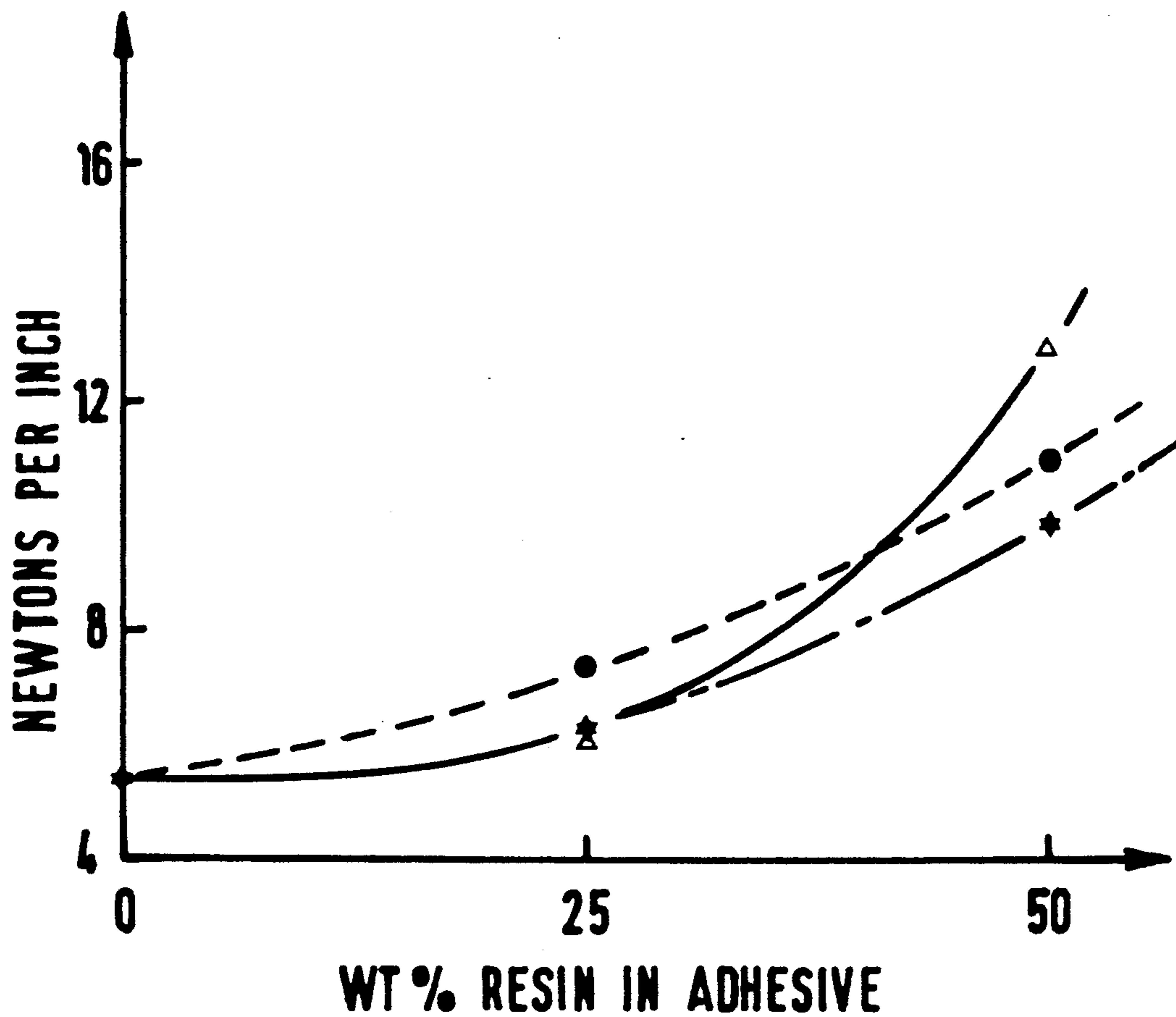
FIG. 2 LOOP TACK
