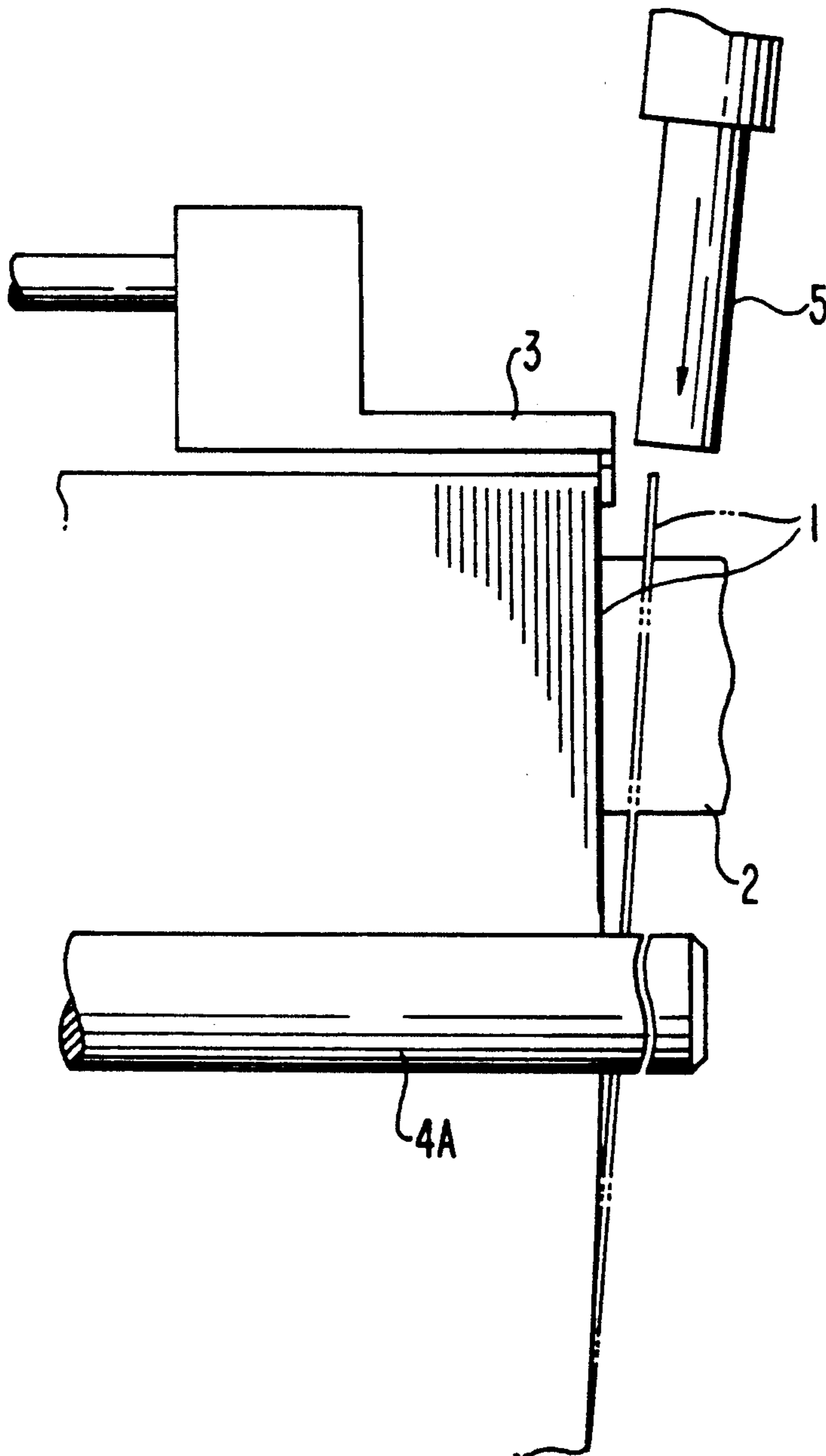
FIG. 16 (PRIOR ART)
