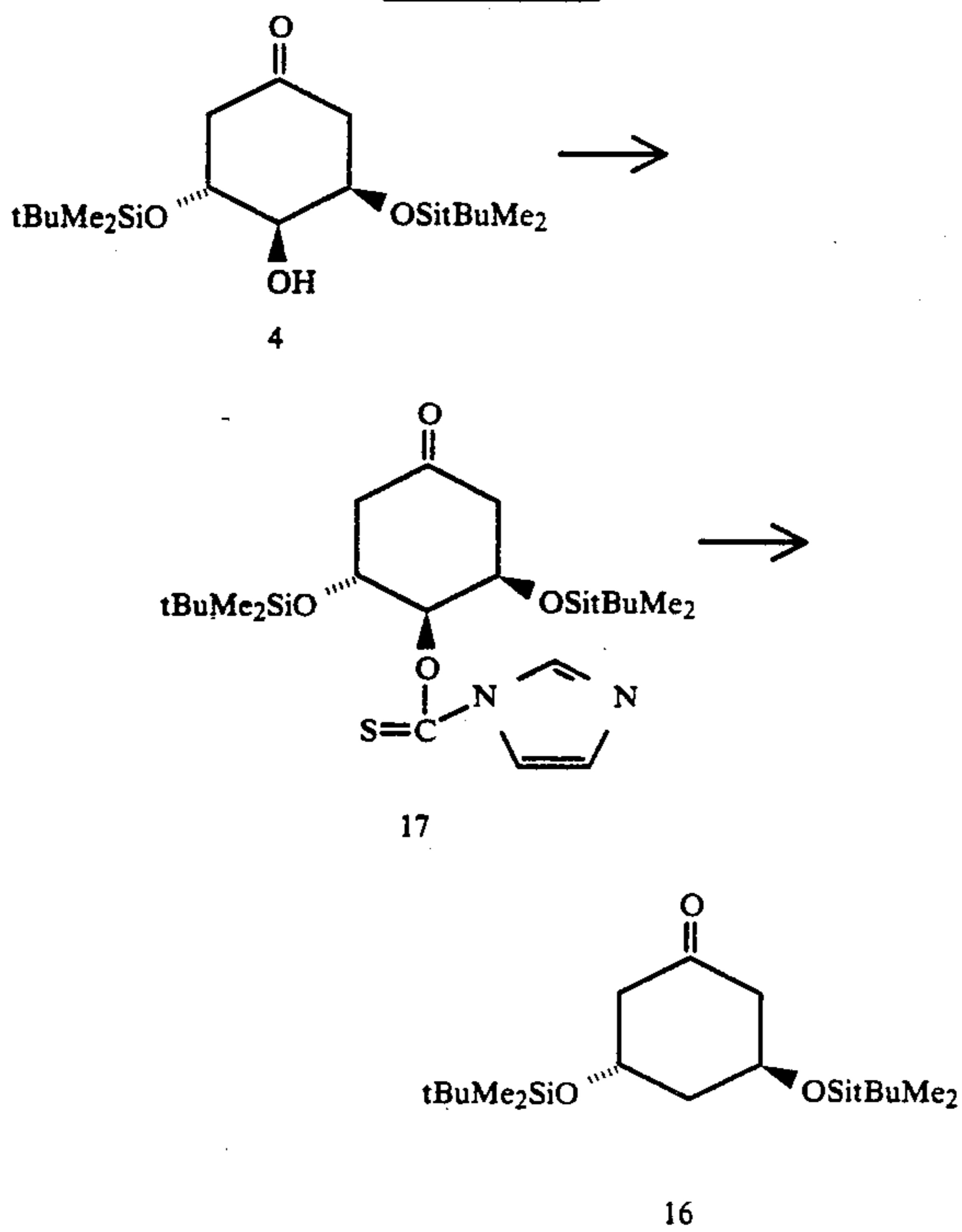
Scheme III
