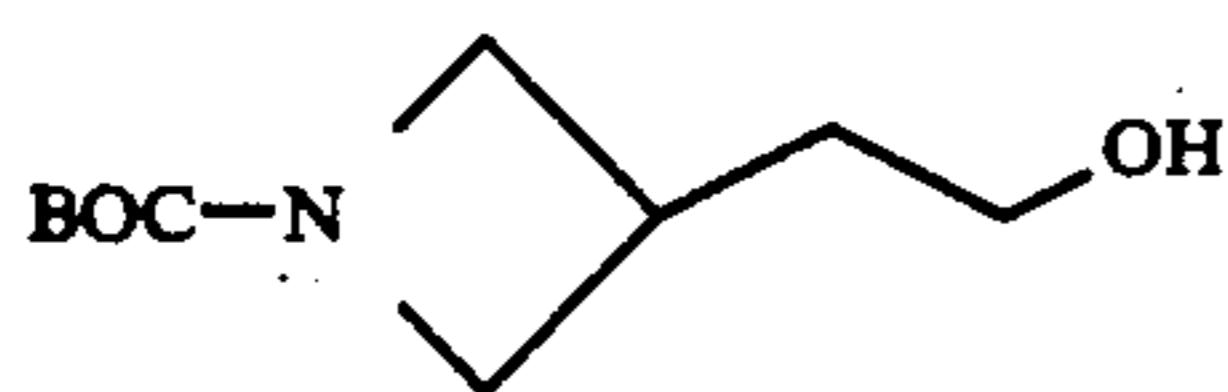
N-BOC-Azetidin-3-ylethanol (133)
