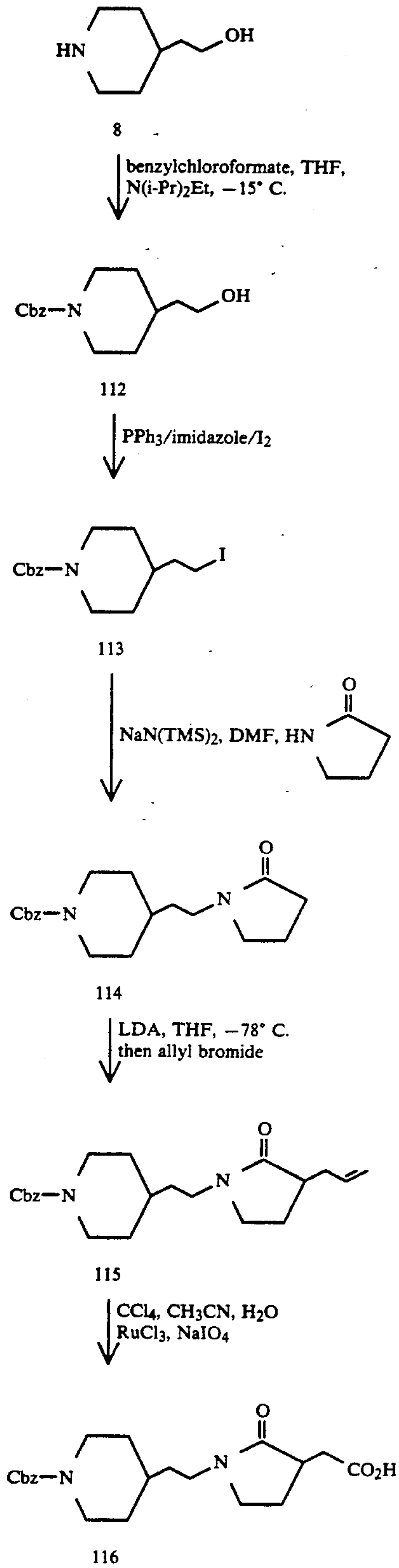
SCHEME 14
