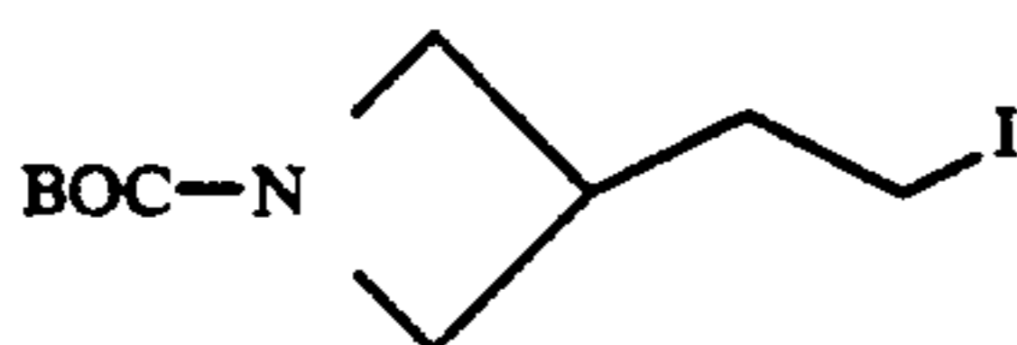
N-BOC-Azetidin-3-ylethyl iodide (134)
