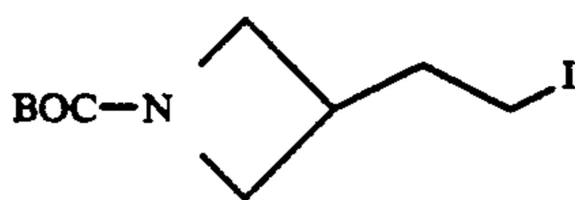
N-BOC-Azetidin-3-ylethyl iodide (134)
