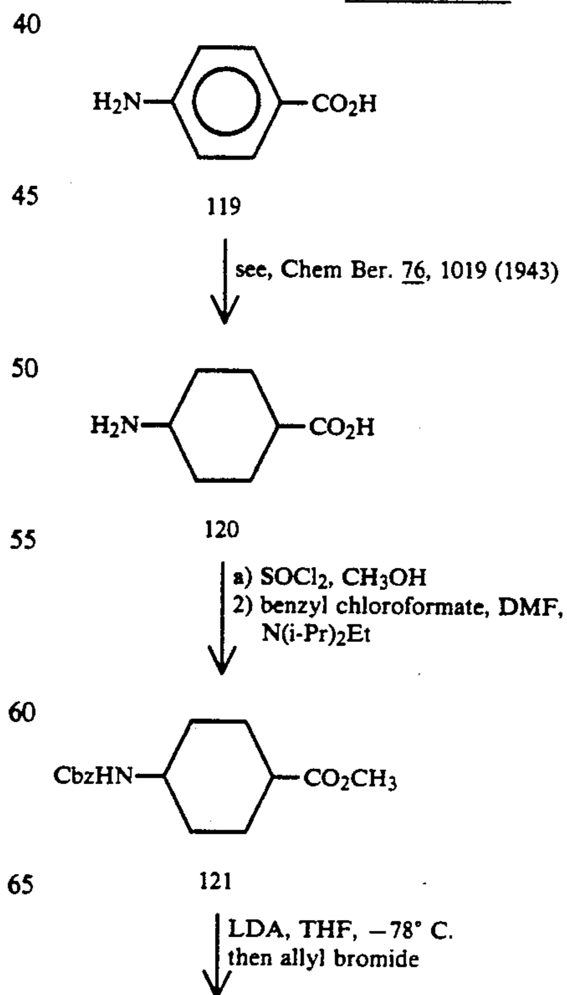
SCHEME 15
