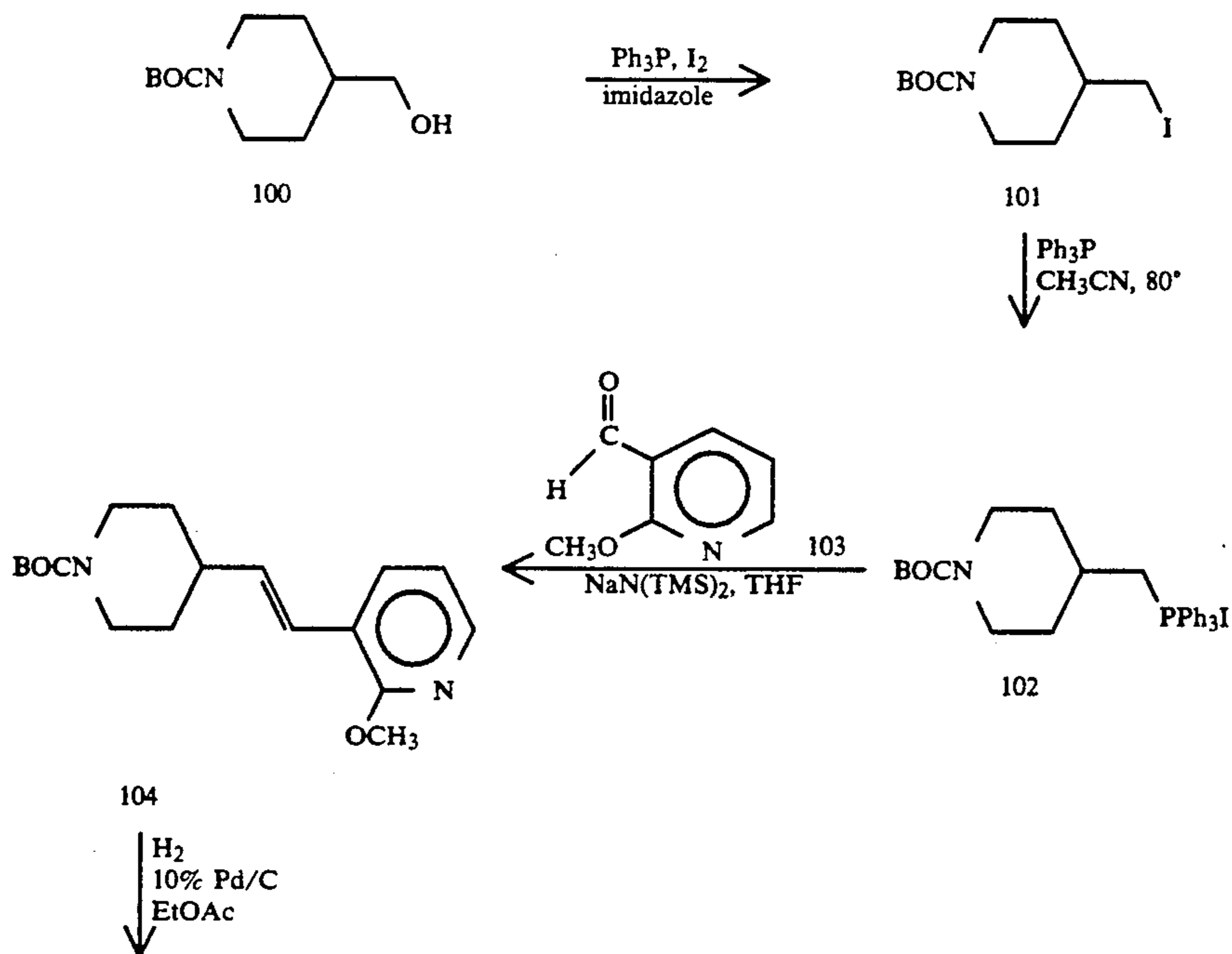
SCHEME 13
