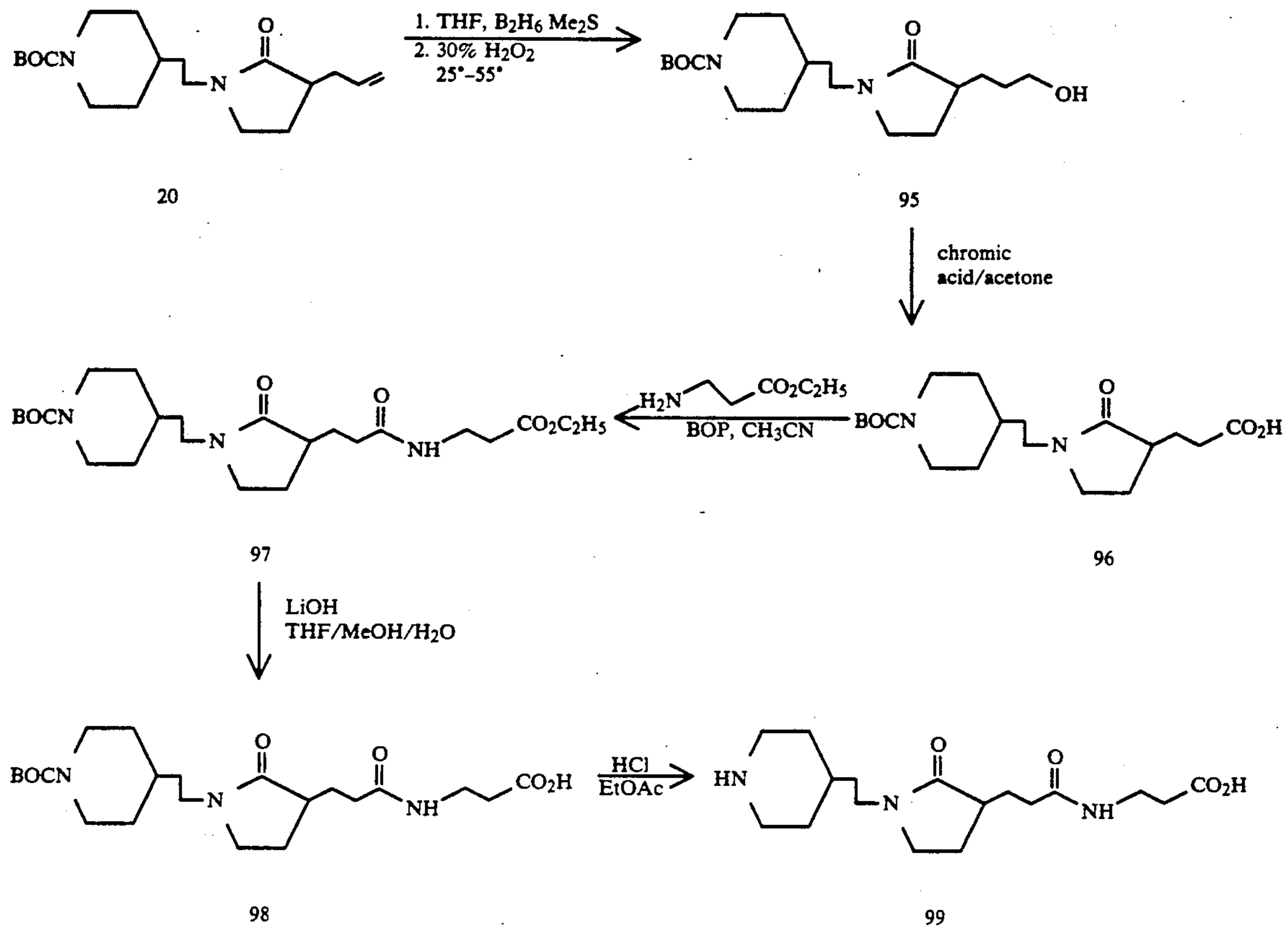
SCHEME 12
