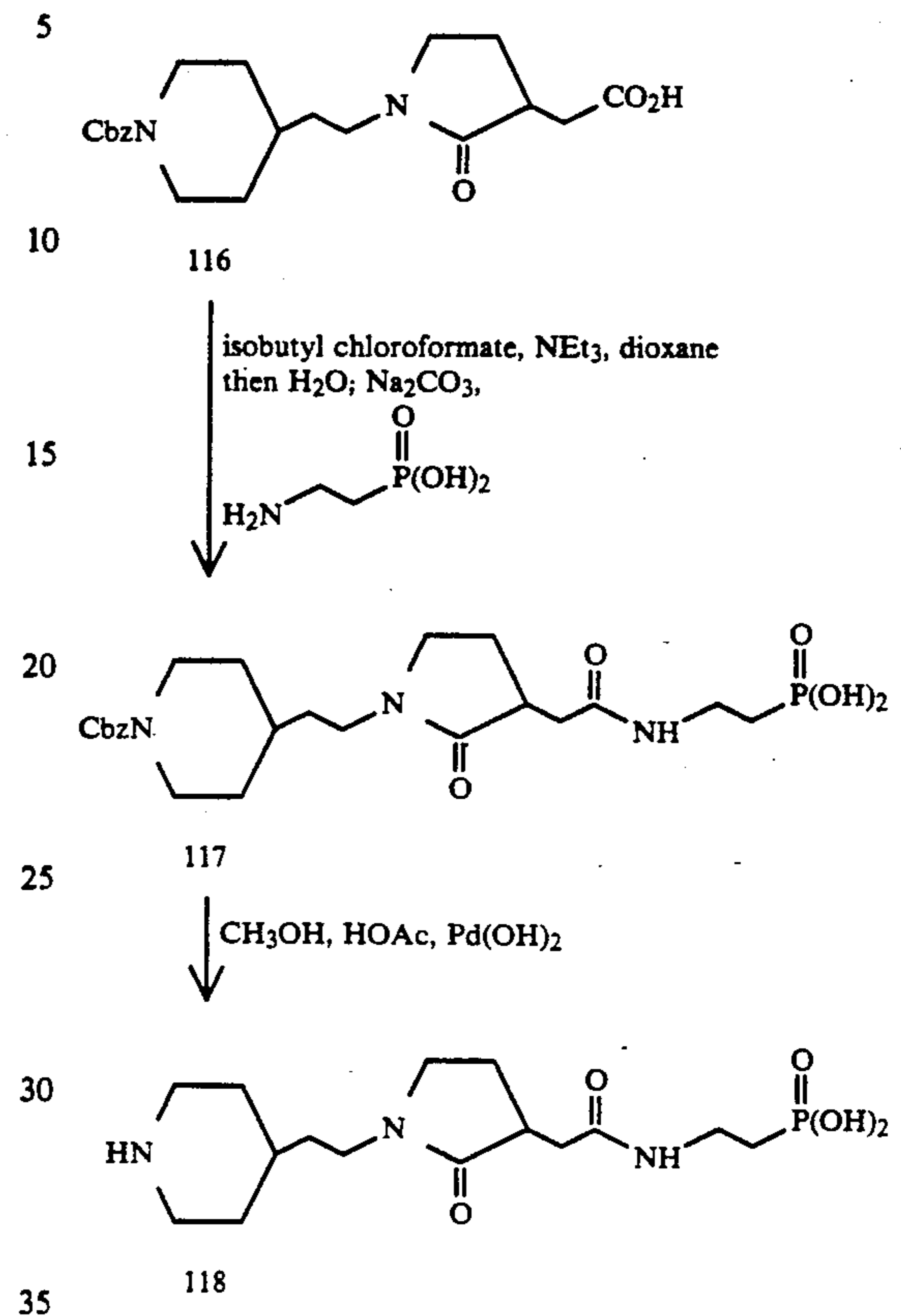
SCHEME 14
