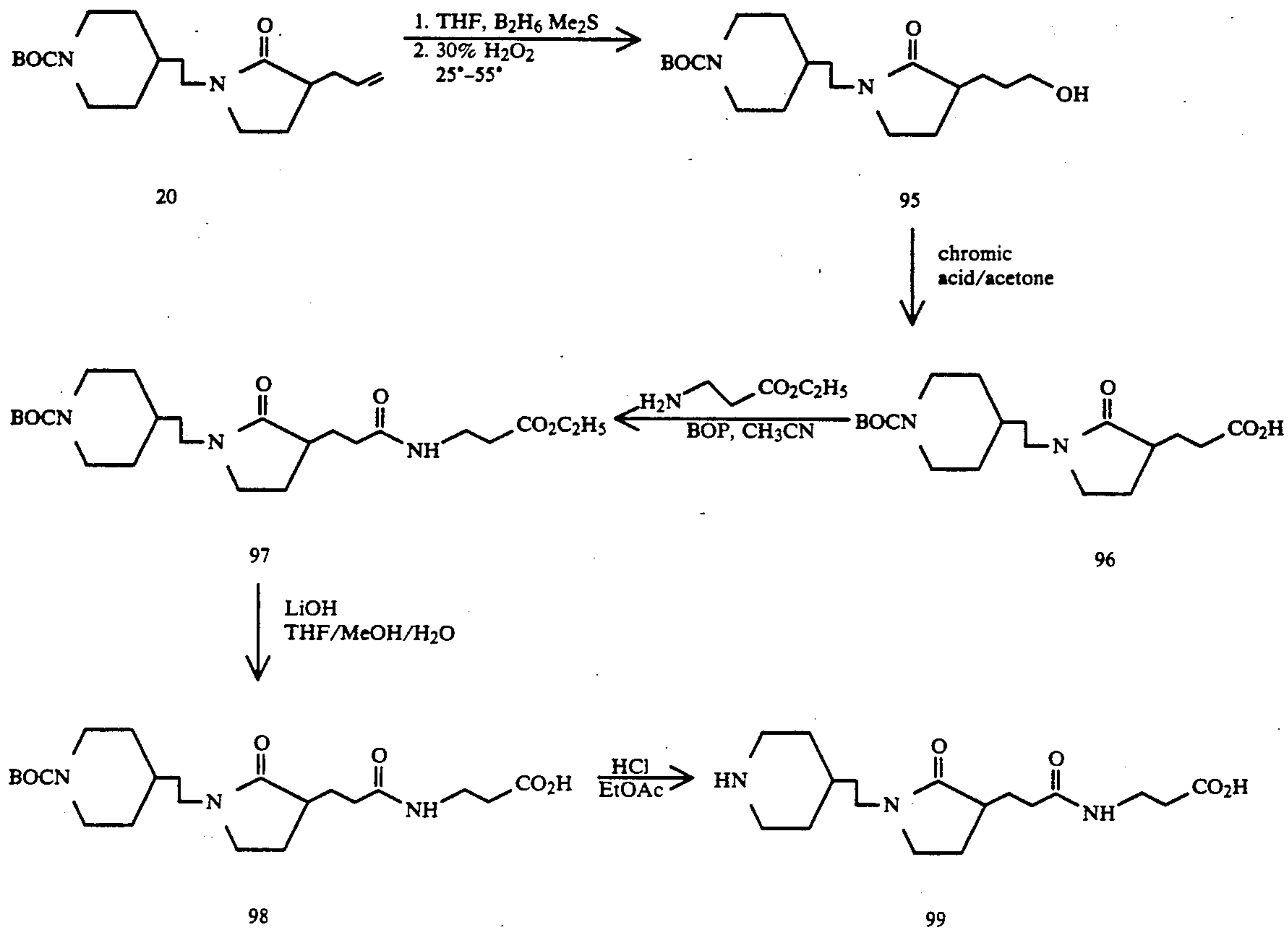
SCHEME 12
