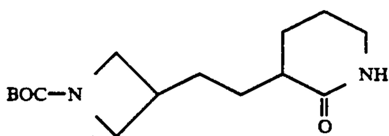
3-[N-BOC-2-(Azetidin-3-yl)ethyl]-2-piperidone (136)
