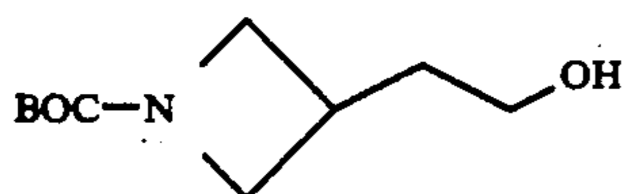
N-BOC-Azetidin-3-ylethanol (133)
