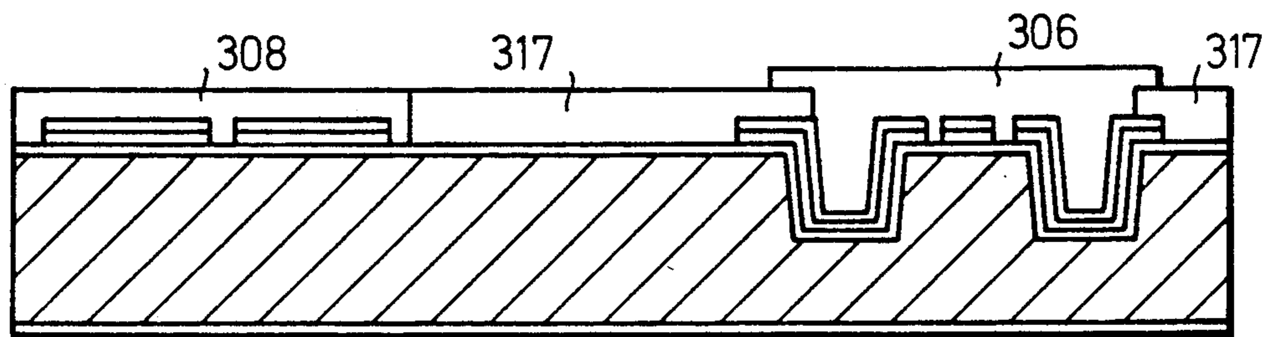
Fig.3(l1) I-I SECTION
