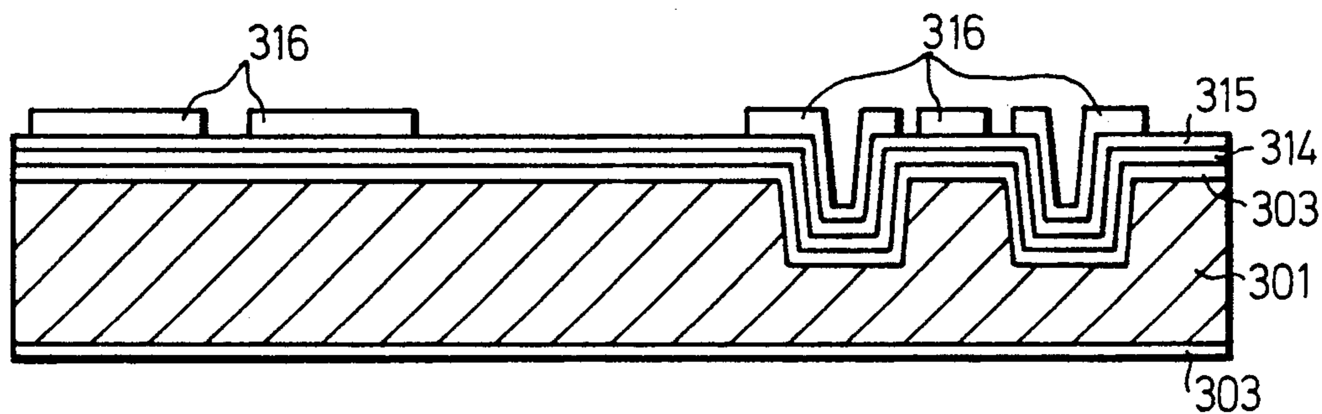
Fig.3(h1) I-I SECTION
