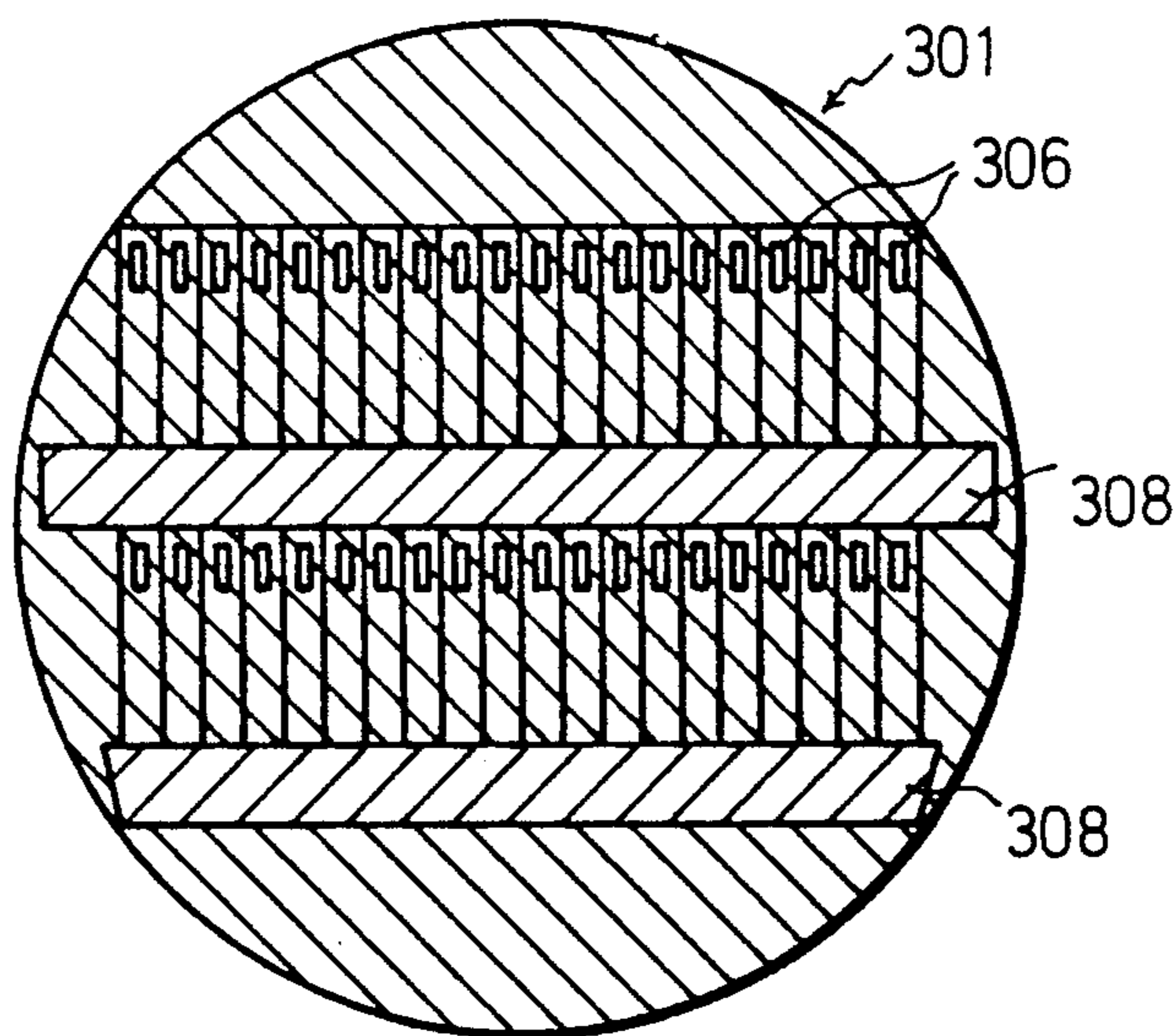
Fig.3(l2) PLAN VIEW (ENTIRE WAFER)
