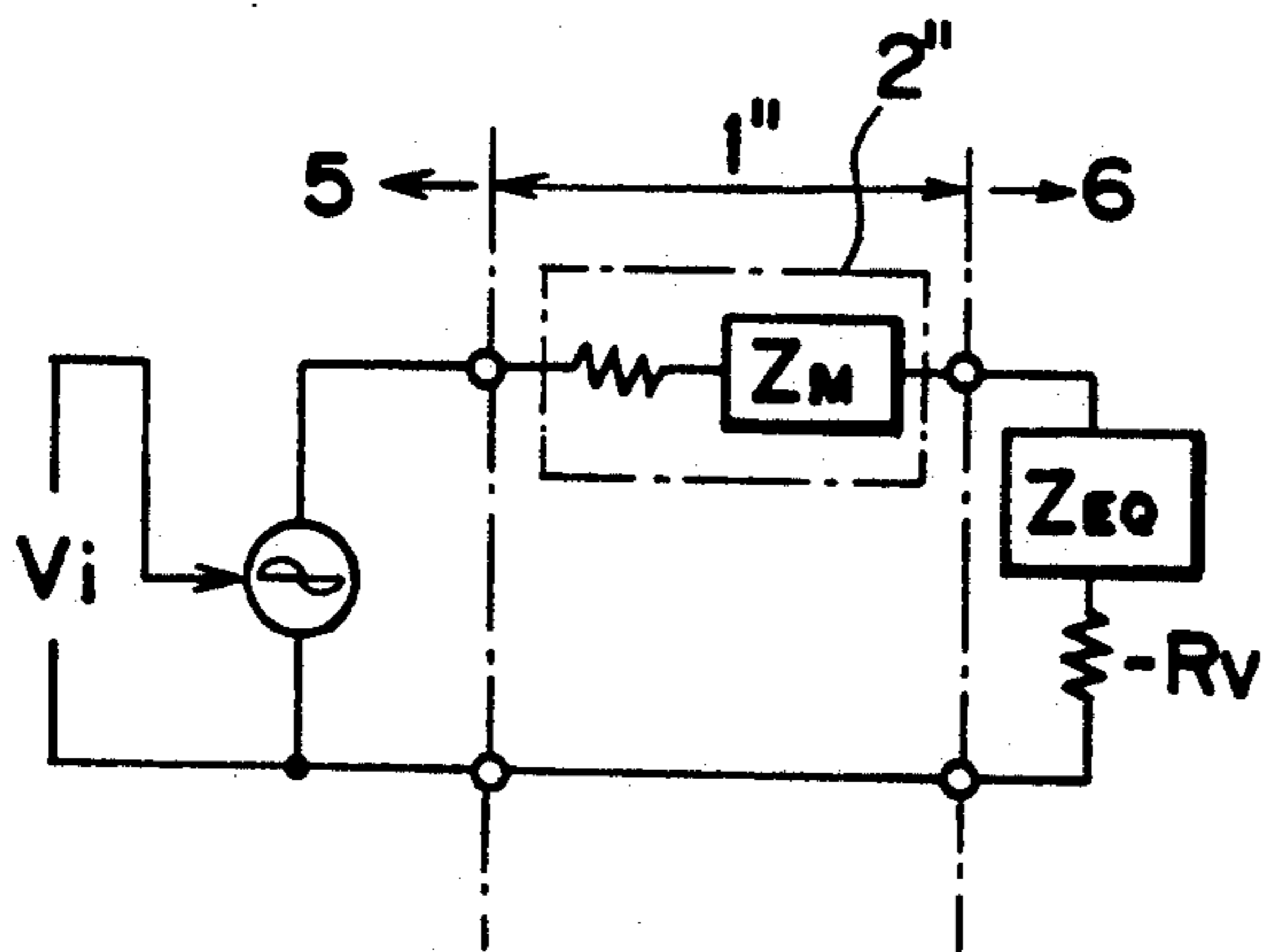
FIG. 3C PRIOR ART
