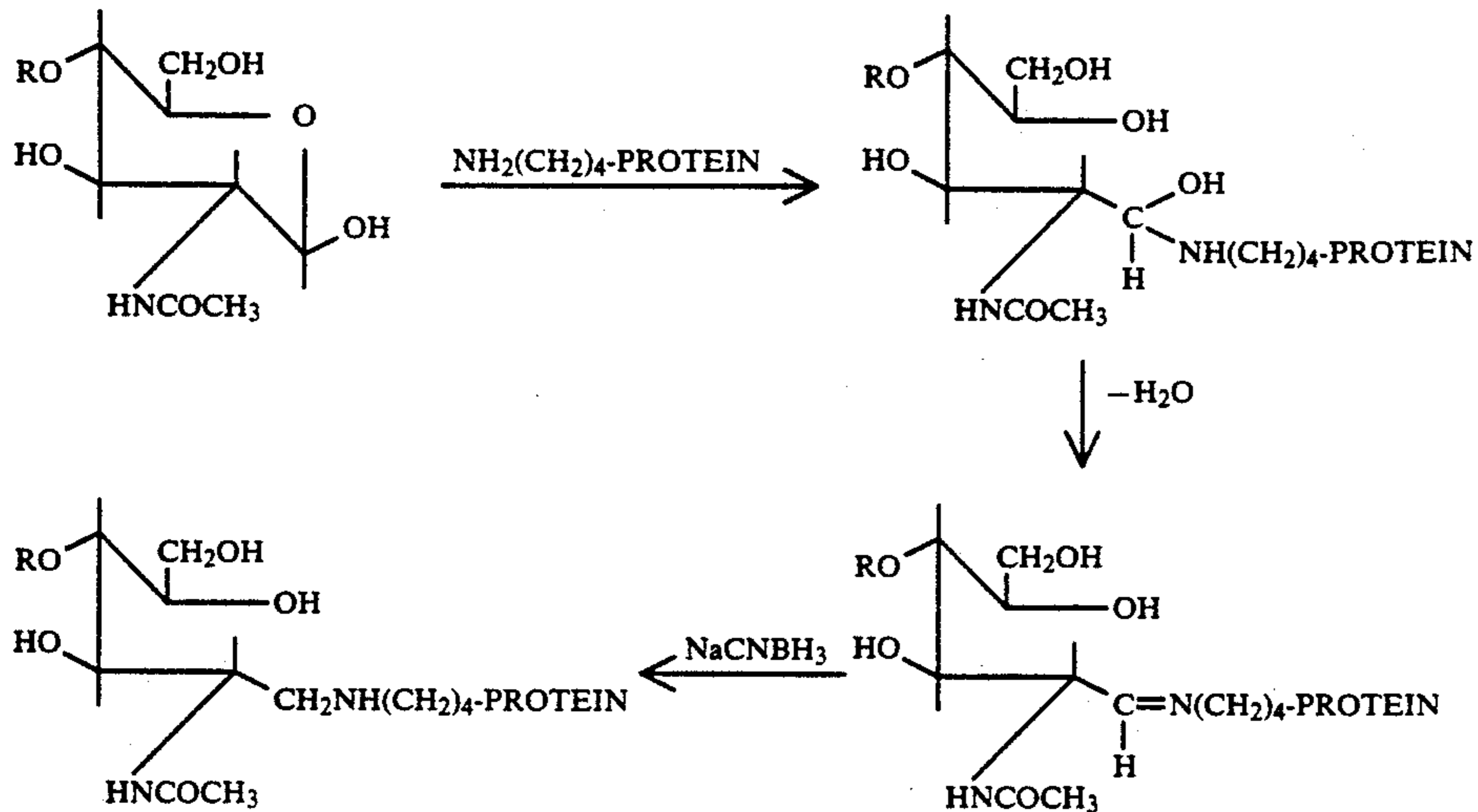
NEOGLYCOPROTEIN FORMATION BY REDUCTIVE AMINATION
