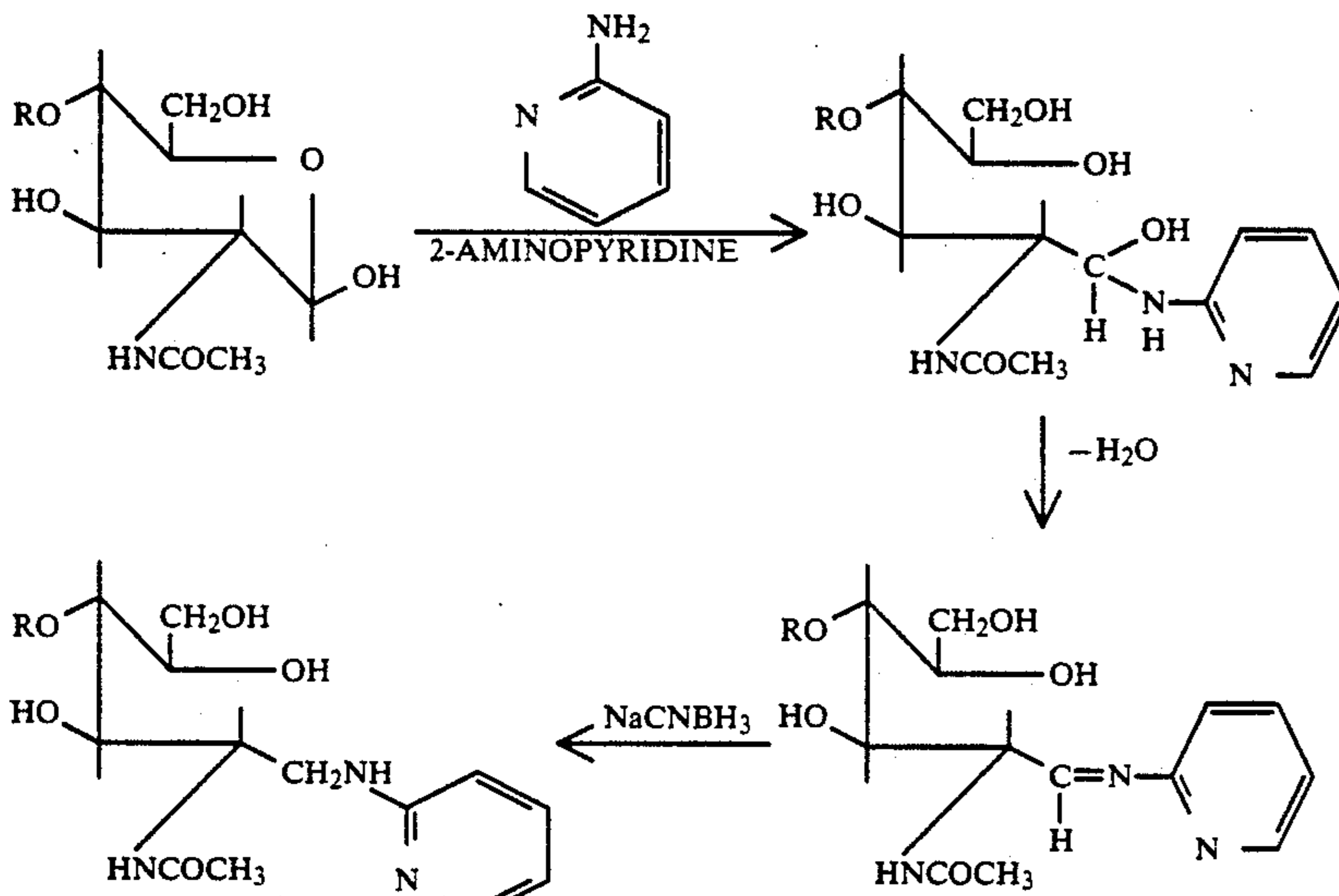
FLUORESCENT DERIVATIZATION BY REDUCTIVE AMINATION
