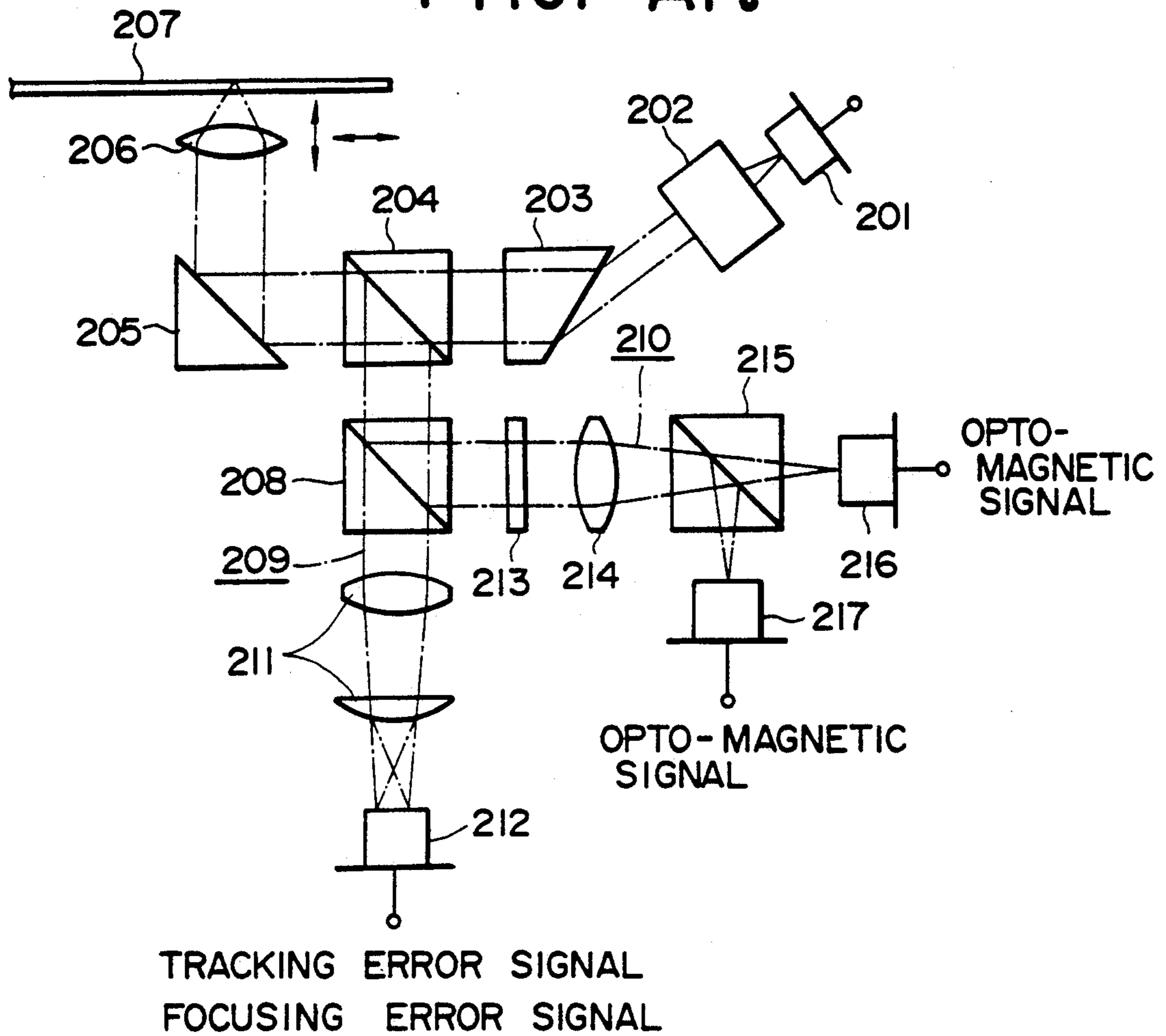
Fig. 24 Prior Art
