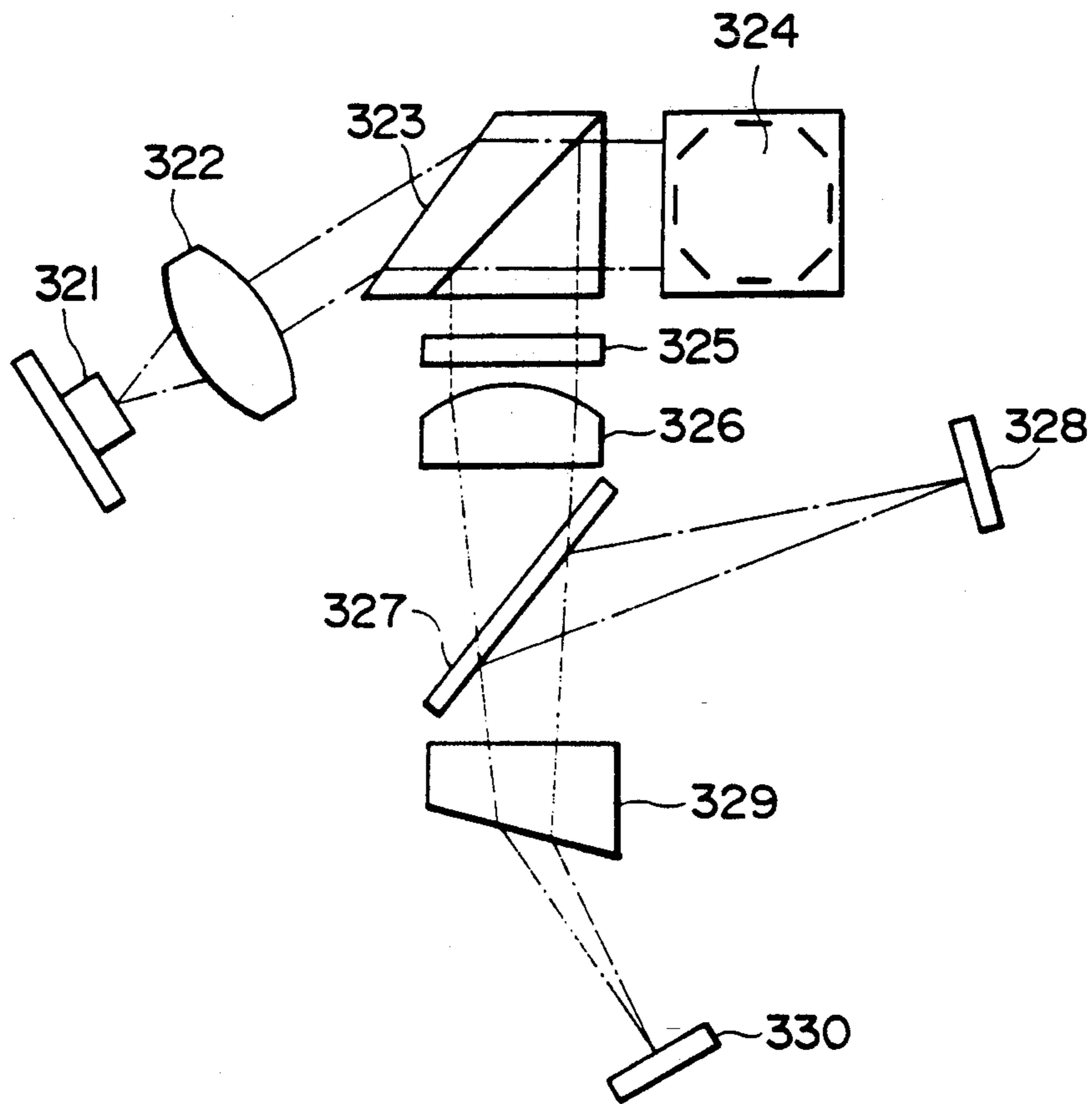
Fig. 34 Prior Art
