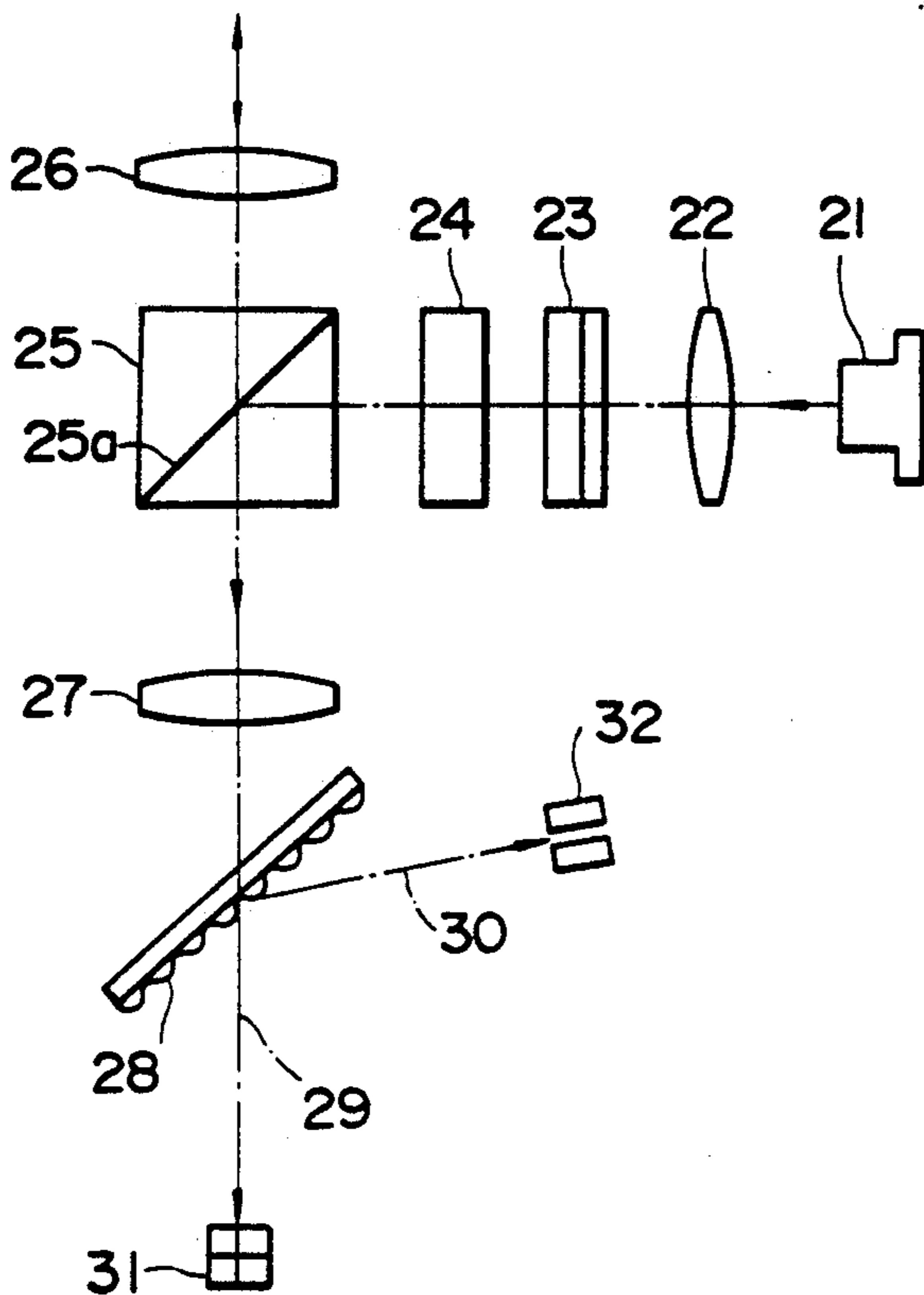
Fig. 10 Prior Art
