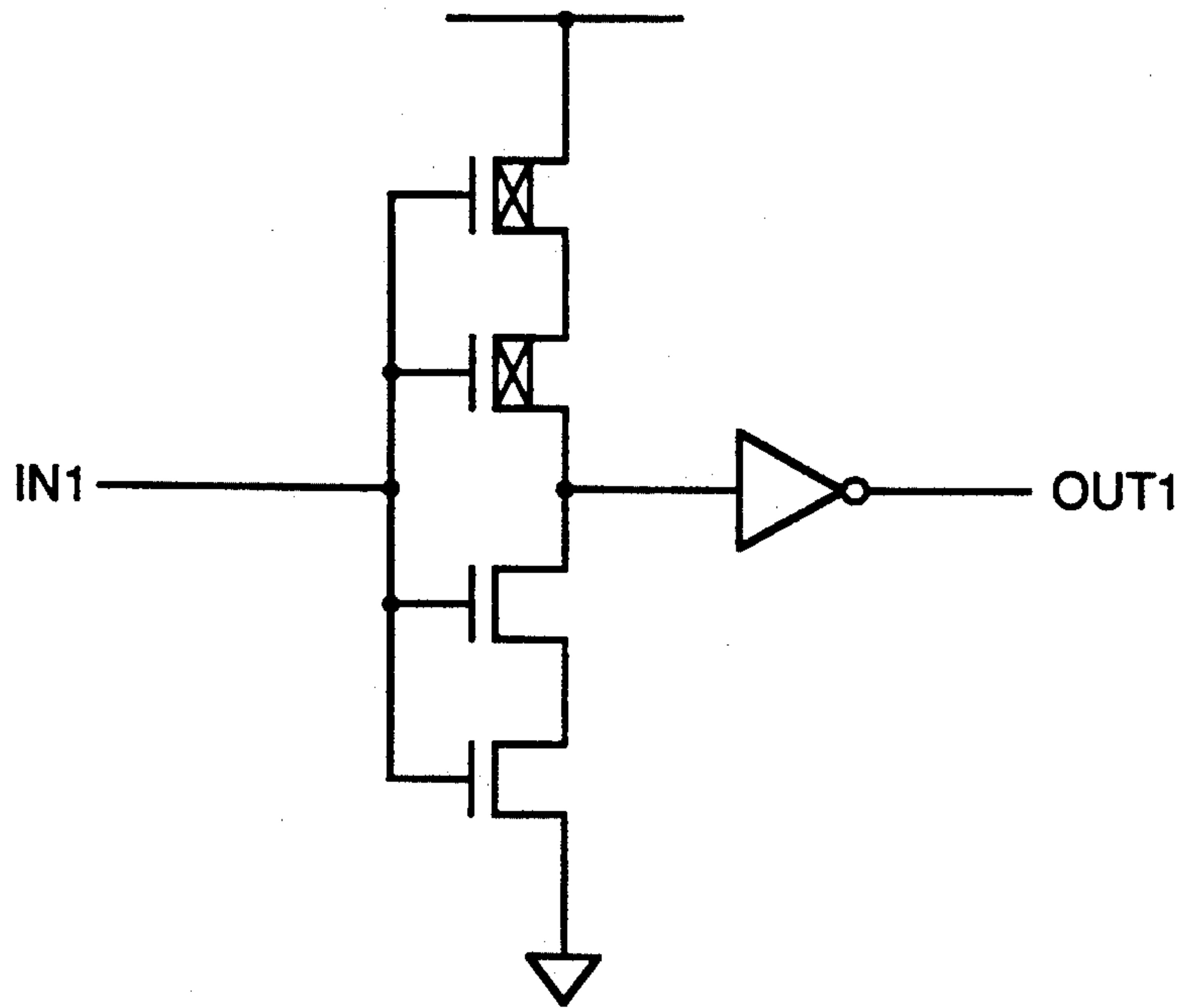
FIG. 1 (PRIOR ART)
