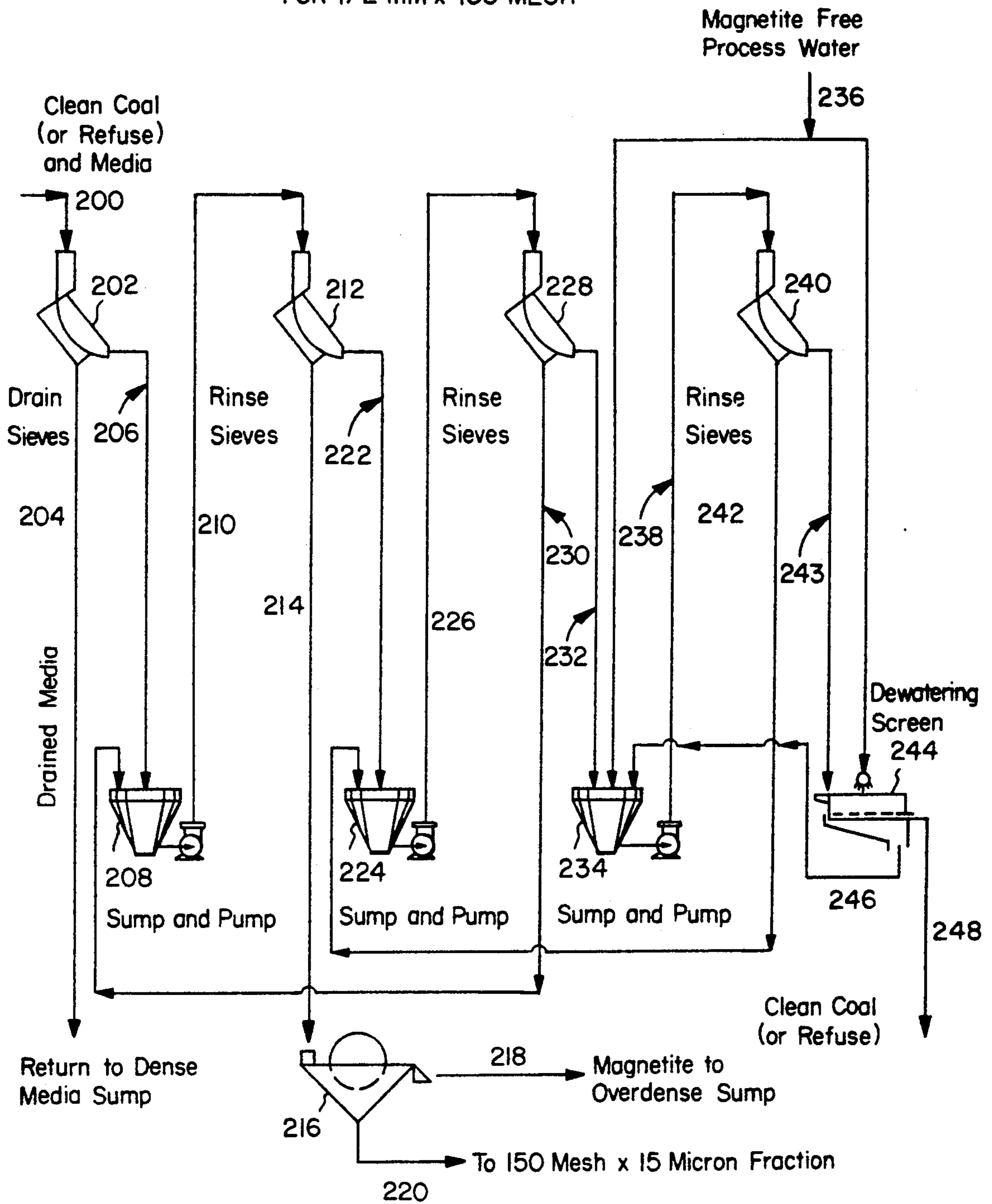
MAGNETITE RECOVERY CIRCUIT FOR 1/2 mm x 150 MESH
