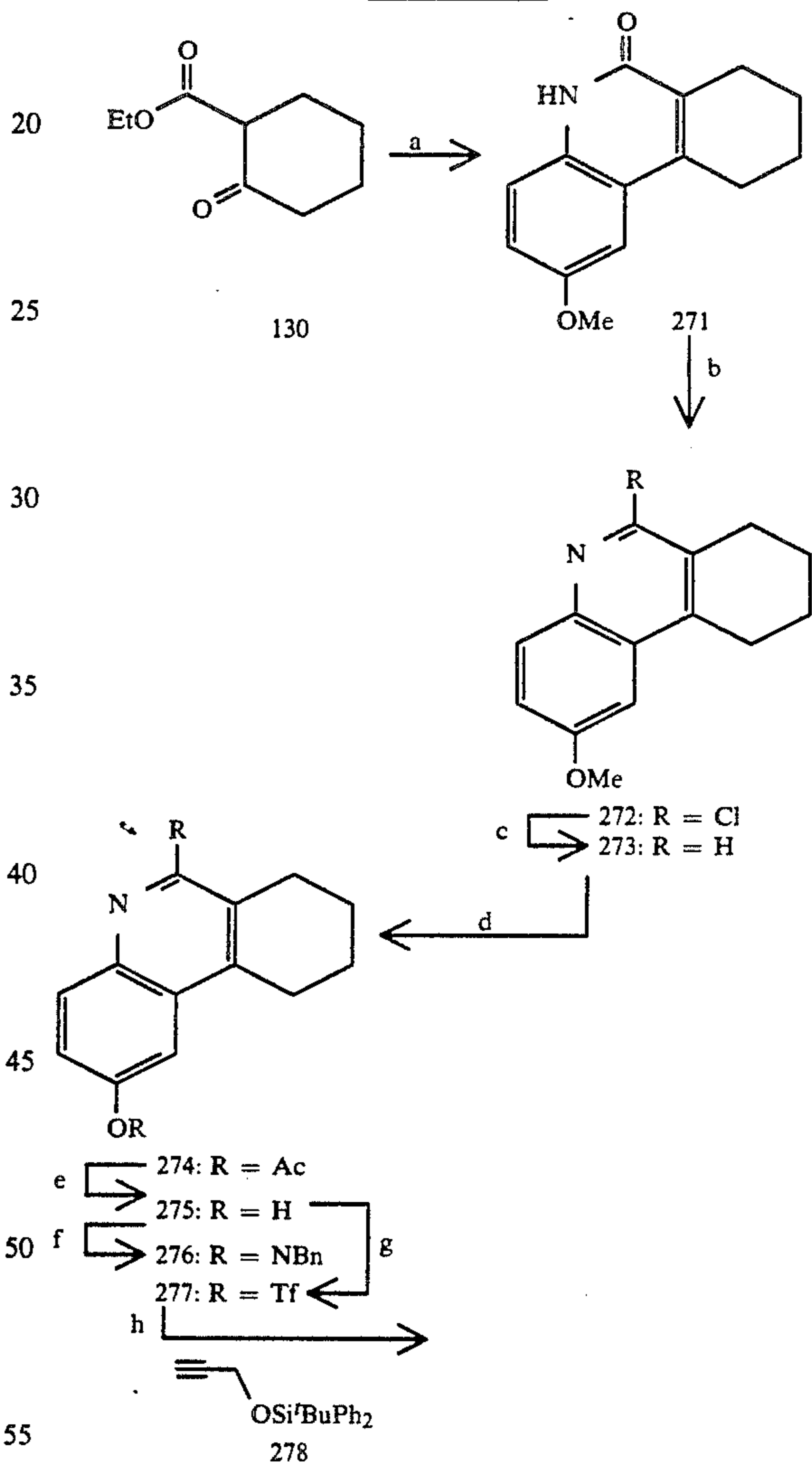
-continued Scheme XX
