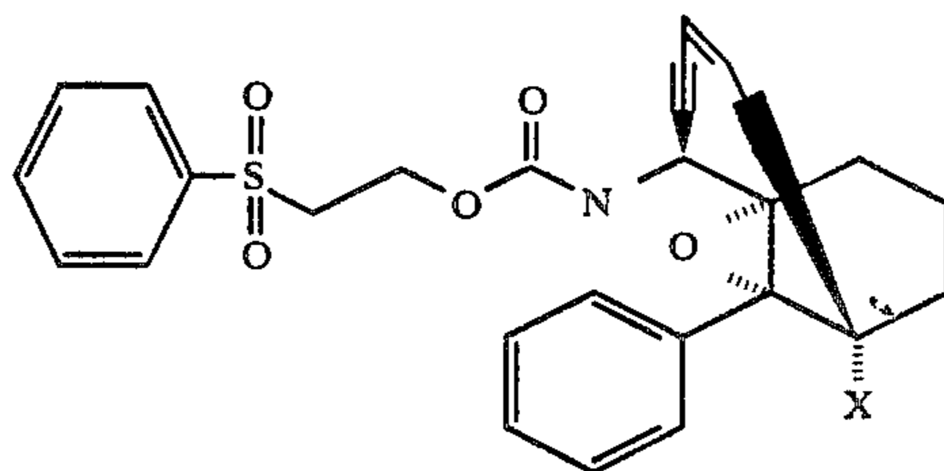
Anticancer Activity (IC 50 ) Of Eneidyne Compounds
