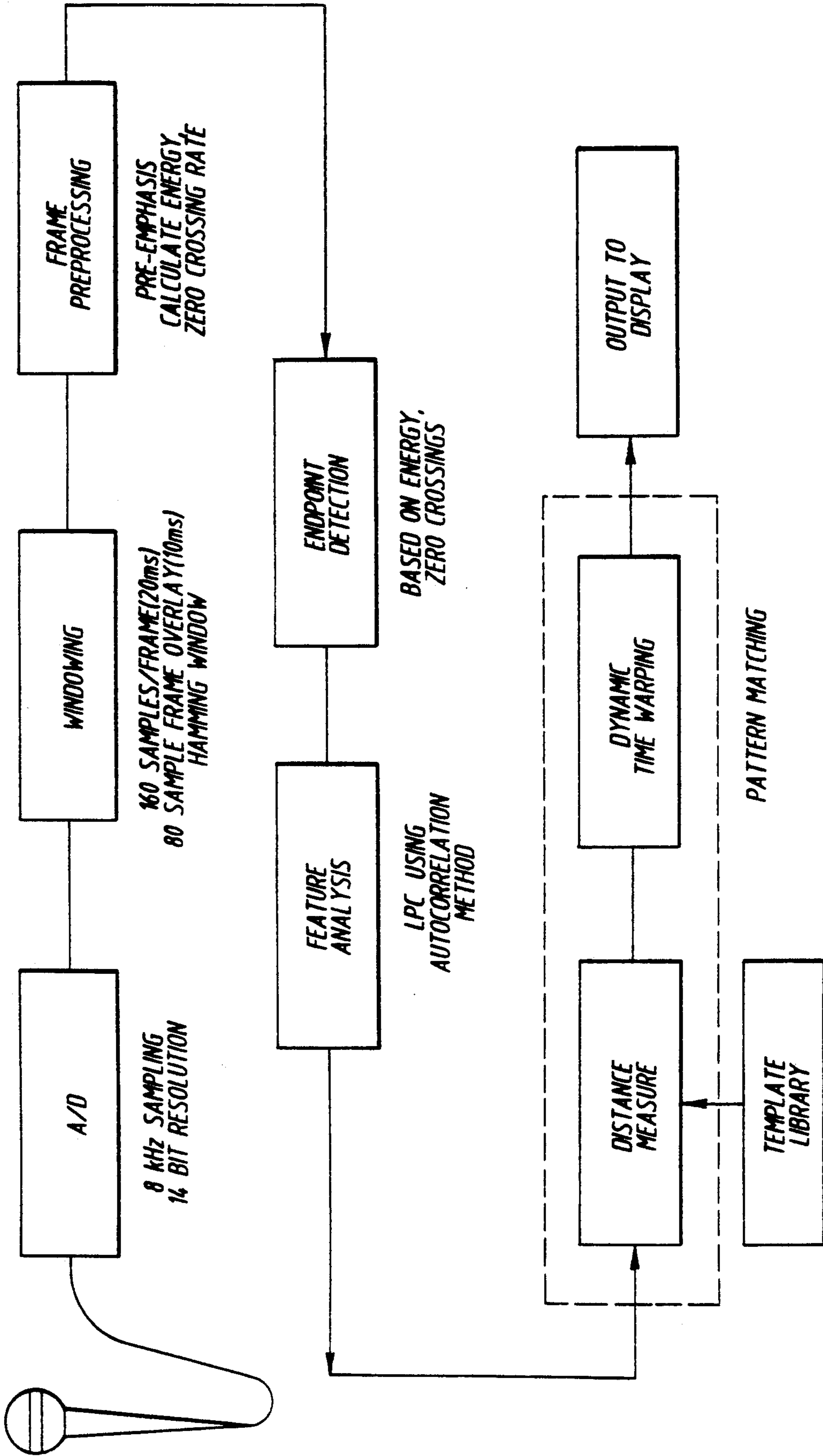
FIG. 7 SPEECH RECOGNITION FLOW DIAGRAM
