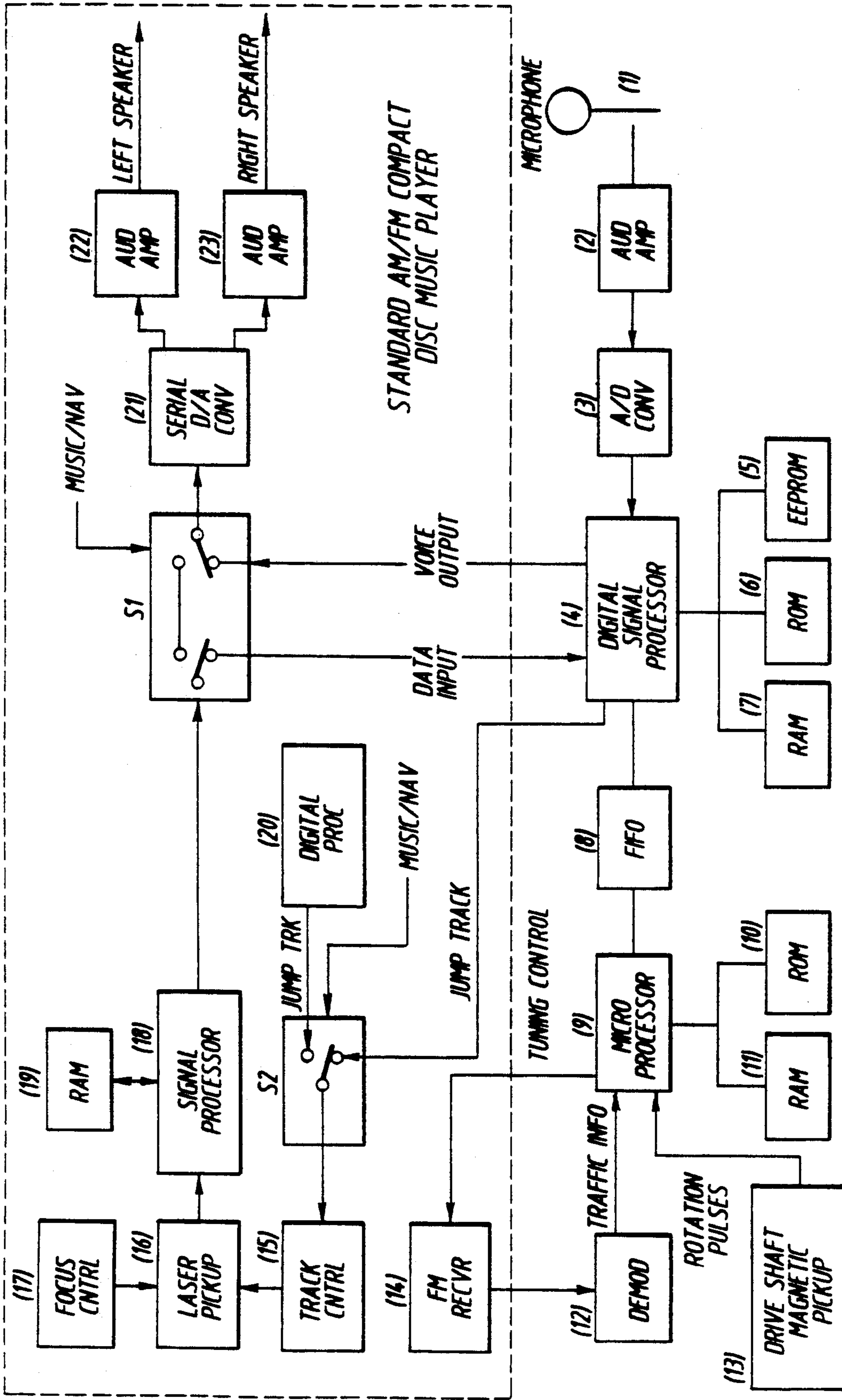
FIG. 4 DUAL PROCESSOR, TRAFFIC UPDATE - ONE SENSOR NAVIGATOR
