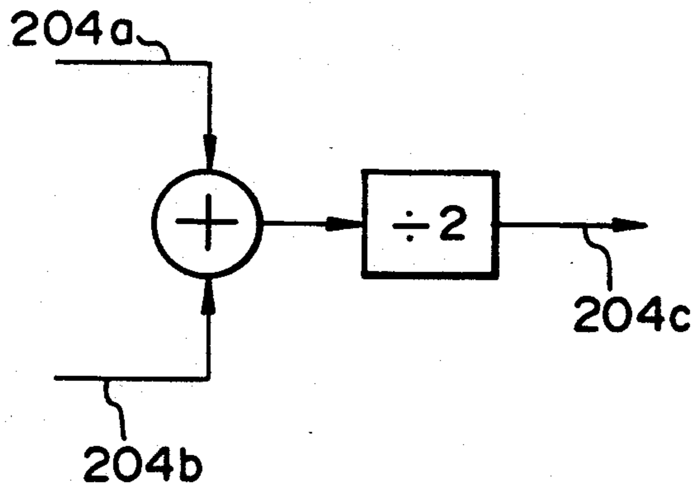
INTERPOLATION SECTION
