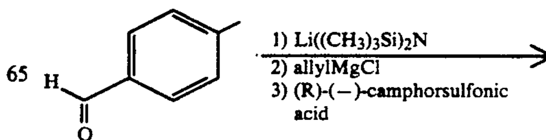
SCHEME 1
