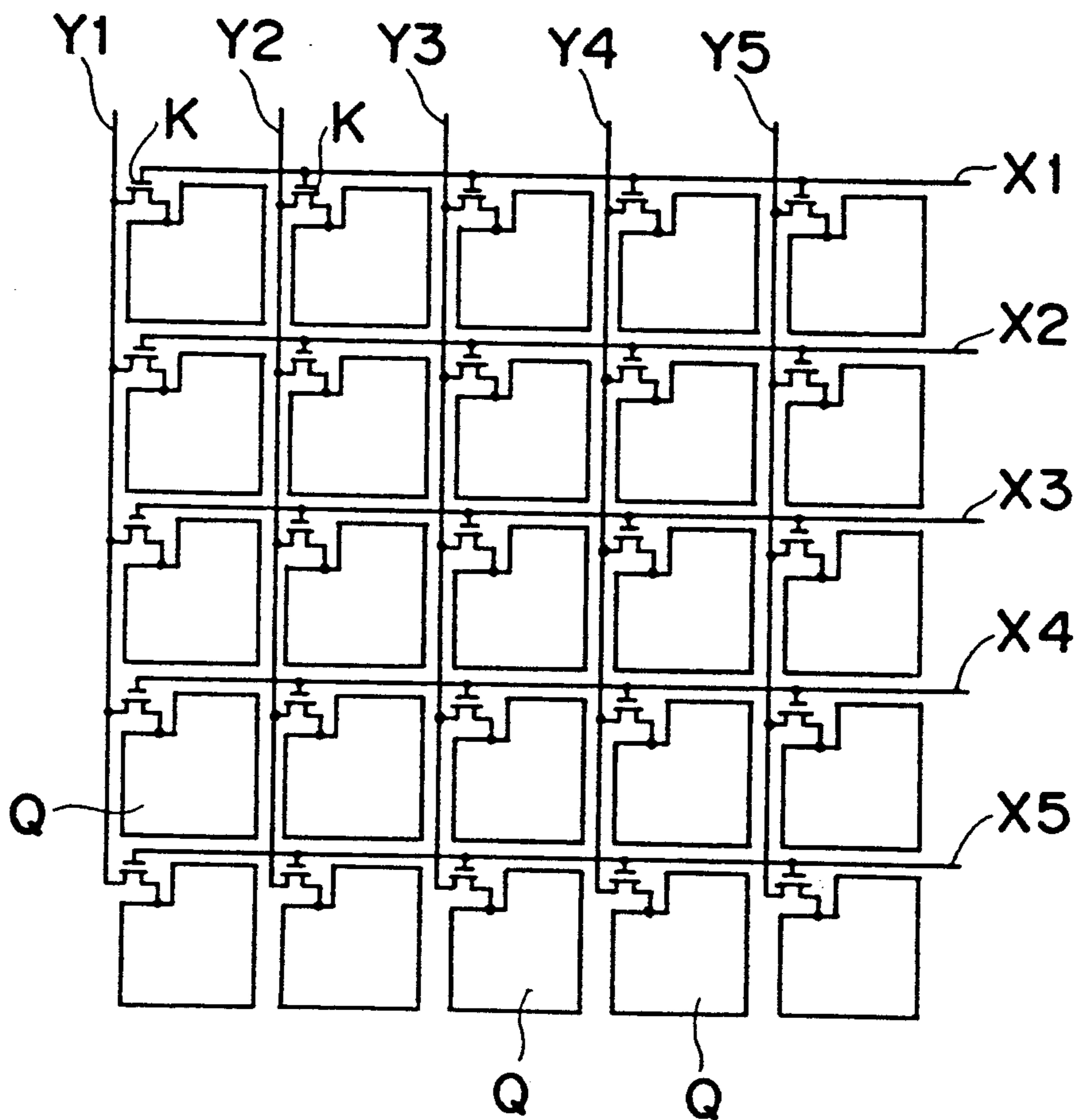
Fig. 7 PRIOR ART
