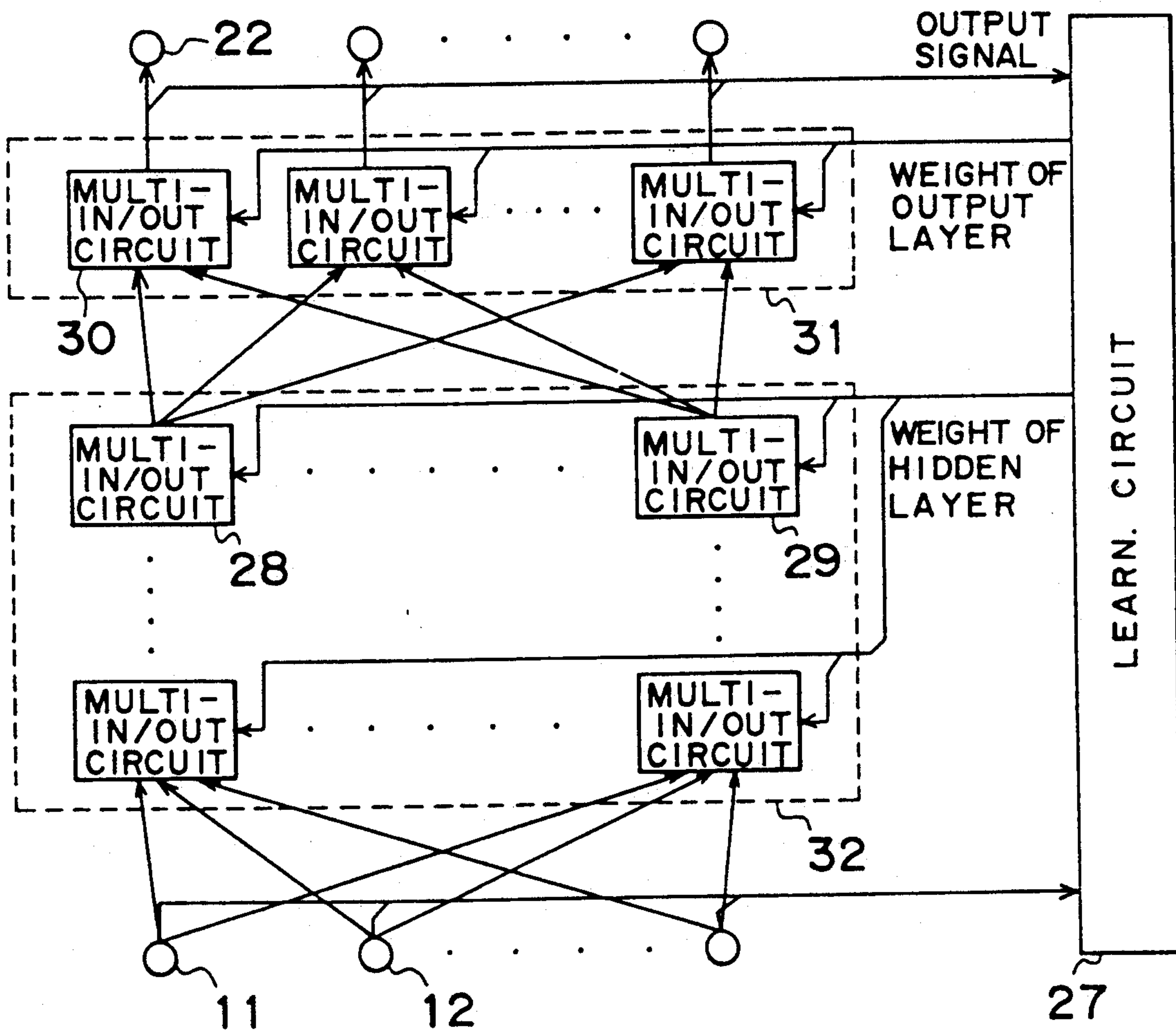
Fig. 2 PRIOR ART
