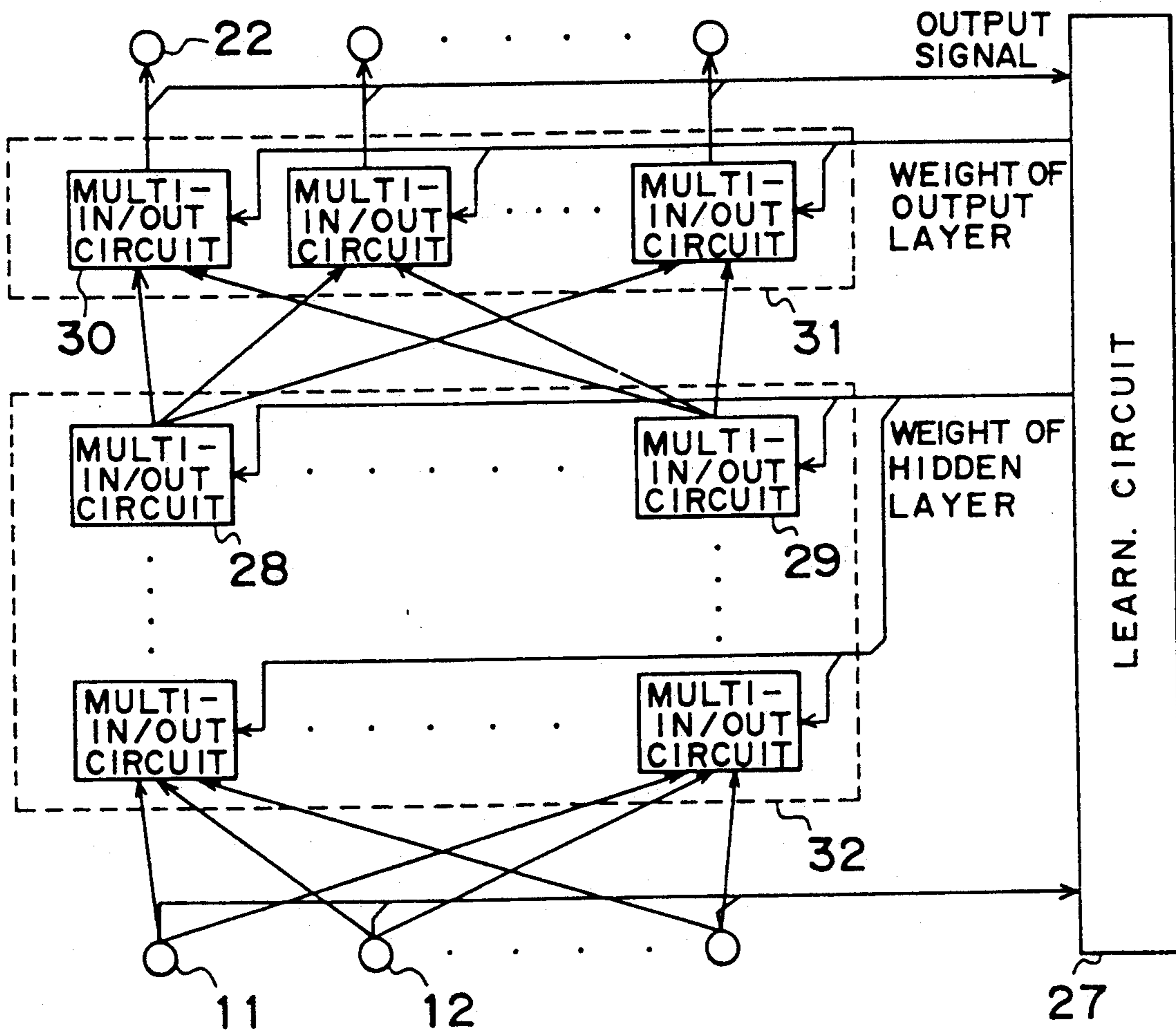
Fig. 2 PRIOR ART
