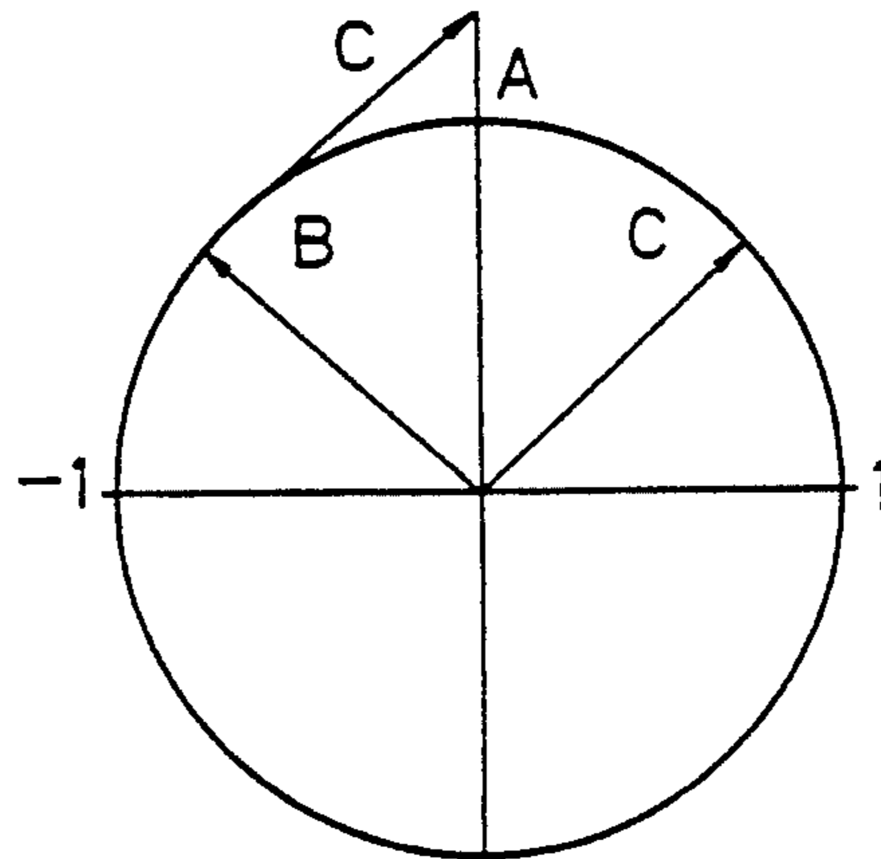
DECOMPOSITION TO TWO CONSTANT ENVELOPE SIGNALS
