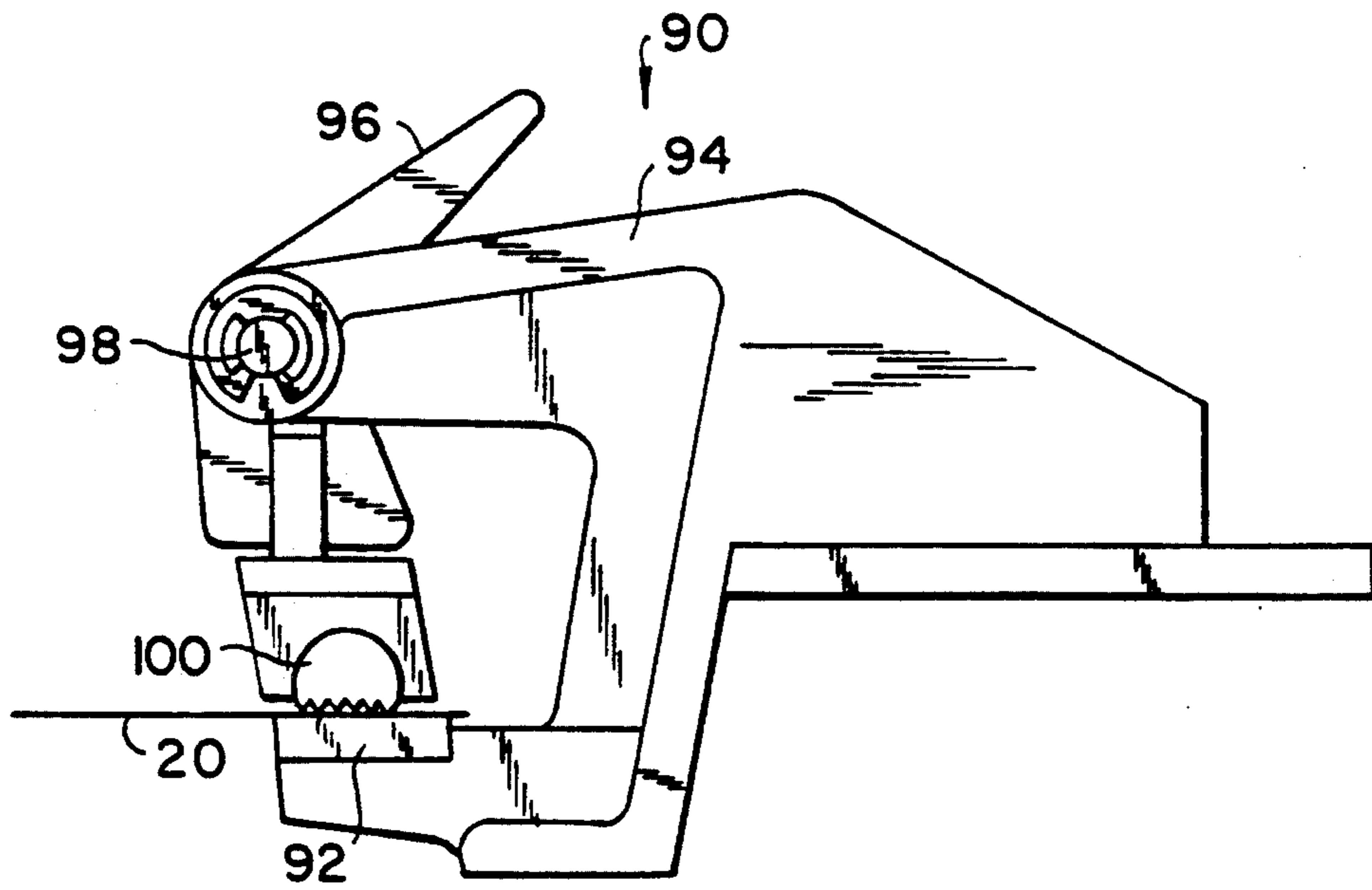
FIG. 4 PRIOR ART
