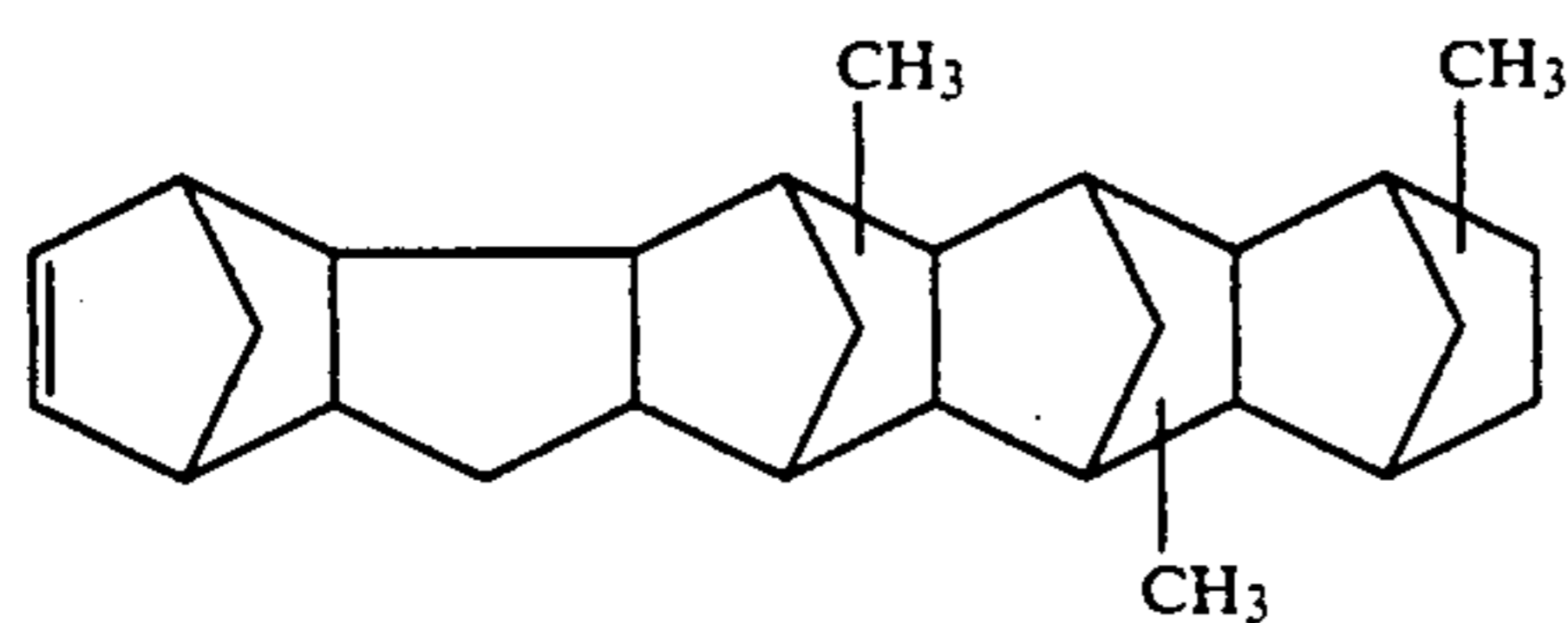
Trimethyl-substituted nonacyclo[9.10.1.14.7.03.8.02.10.012.21.113.20.014.19.115.18]-5-pentacosene
