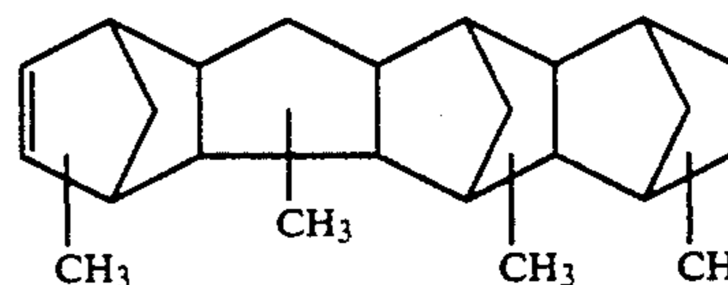
Tetramethyl-heptacyclo[8.7.0.0 2.7.1 3.6.1 10.17.0 11.16.1 12.15 ]eicosene-4
