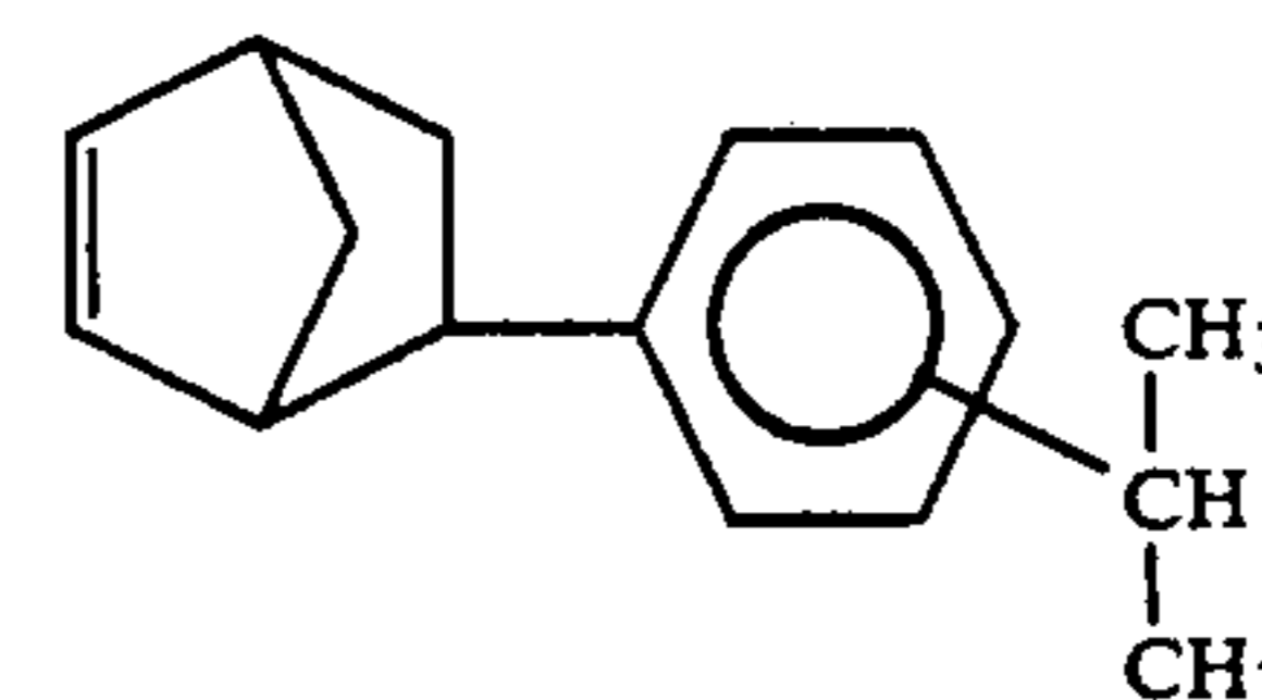
5-(Isopropylphenyl)bicyclo[2.2.1]hept-2-ene
