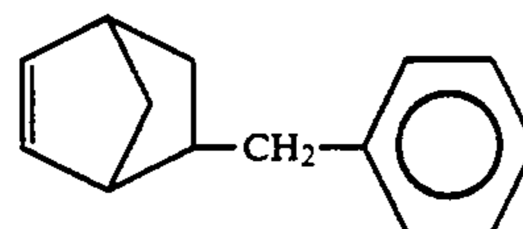
5-Benzylbicyclo[2.2.1]hept-2-ene
