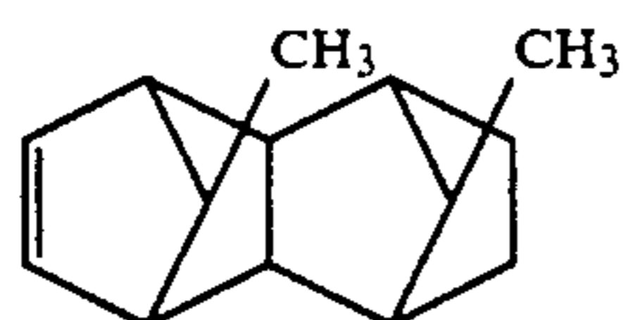
11,12-Dimethyltetracyclo[4.4.0.1 2,5 .1 7,10 ]-3-dodecene
