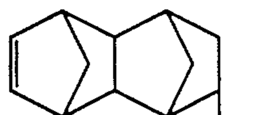
8-Hexyltetracyclo[4.4.0.1 2,5 .1 7,10 ]-3-dodecene
