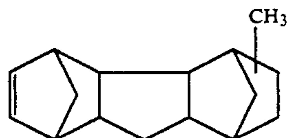
Methyl-substituted-pentacyclo[4.7.0.12.5.08.13.19.12]-3-pentadecene
