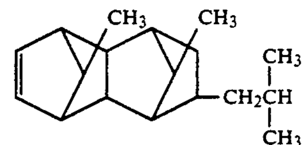
9-Isobutyl-11,12-dimethyltetracyclo[4.4.0.1 2,5 .1 7,10 ]-3-dodecene
