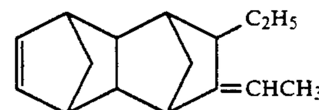
8-Ethylidene-9-ethyltetracyclo[4.4.0.1 2,5 .1 7,10 ]-3-dodecene
