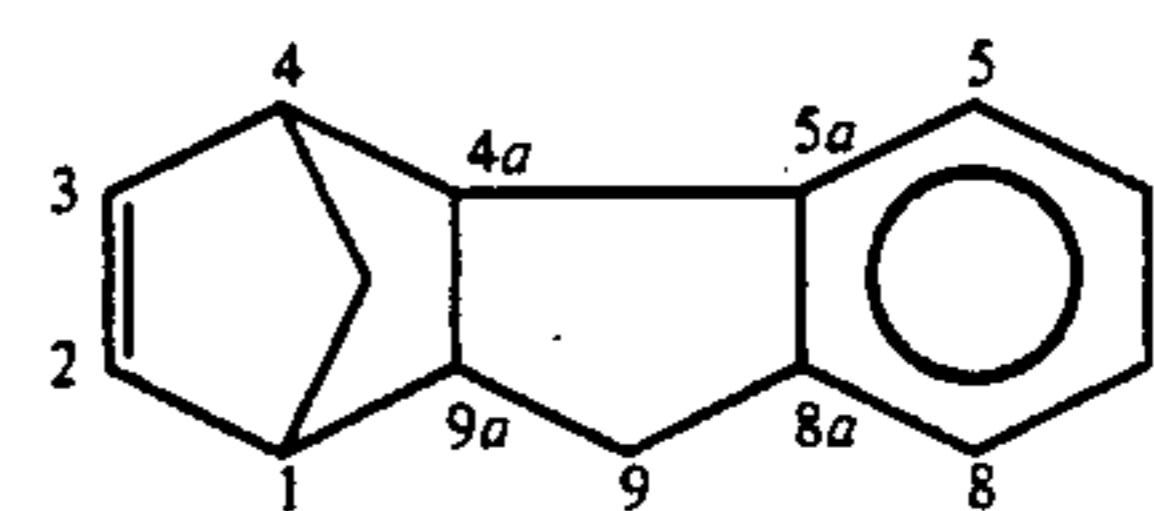
1,4-Methano-1,4,4a,9a-tetrahydrofluorene
