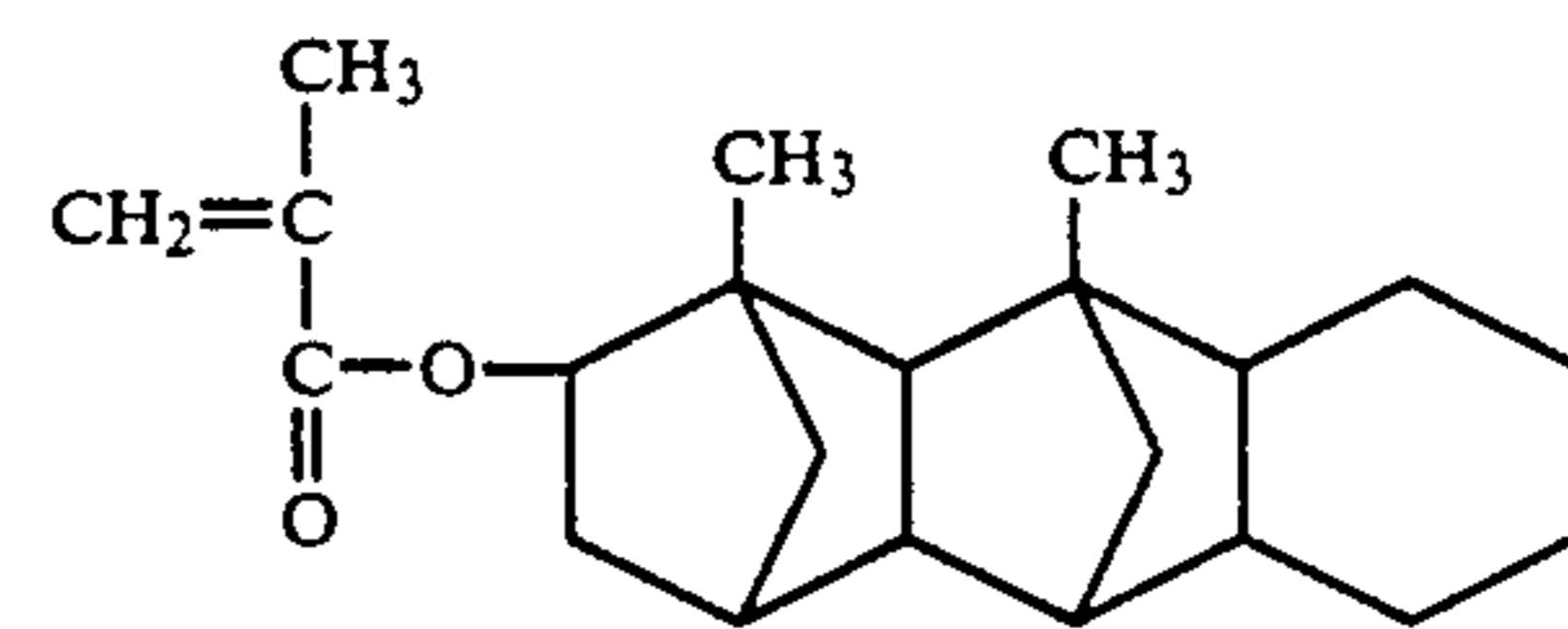
1,3-Dimethylpentacyclo[6.6.1.1 3 .6.0 2 .7.0 9 .14]hexadecyl-4-methacrylate
