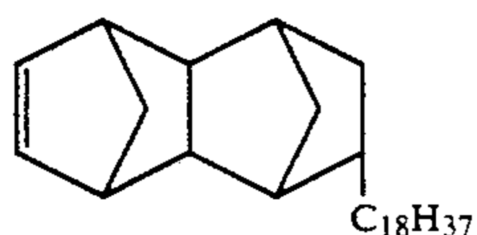
8-Stearyltetracyclo[4.4.0.1 2,5 .1 7,10 ]-3-dodecene
