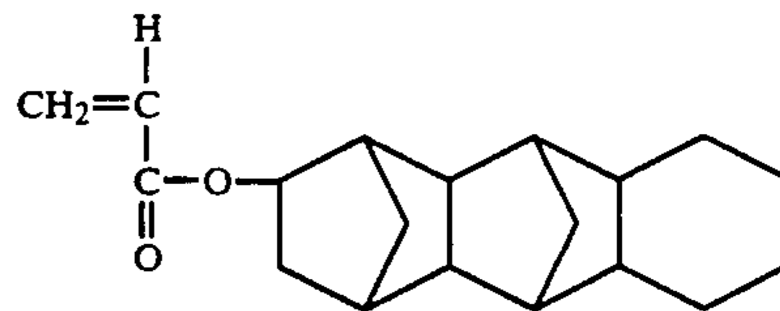
Pentacyclo[6.6.1.1.3.6.0.2.7.0.9.14]-hexadecyl-4-acrylate
