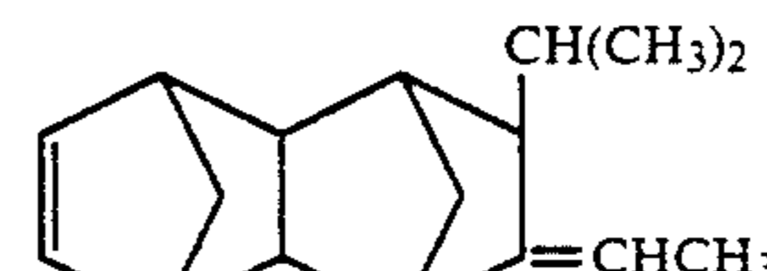
8-Ethylidene-9-isopropyltetracyclo[4.4.0.1 2,5 .1 7,10 ]-3-dodecene
