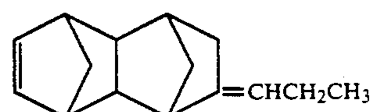
8-n-Propylidenetetracyclo[4.4.0.1 2,5 .1 7,10 ]-3-dodecene
