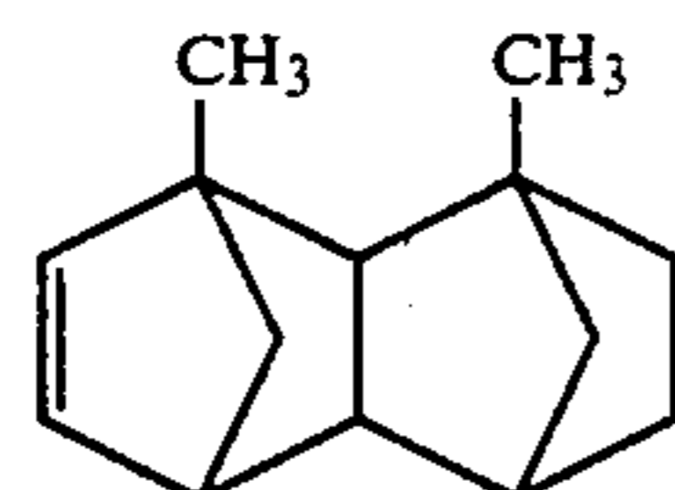
2,10-Dimethyltetracyclo[4.4.0.1 2,5 .1 7,10 ]-3-dodecene
