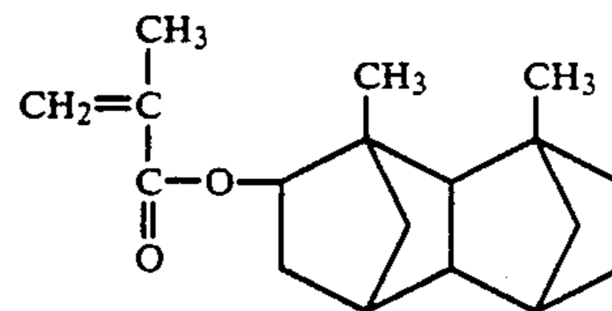
2,10-Dimethyltetracyclo[4.4.0.1 2,5 .1 7,10 ]-dodecyl-3-methacrylate
