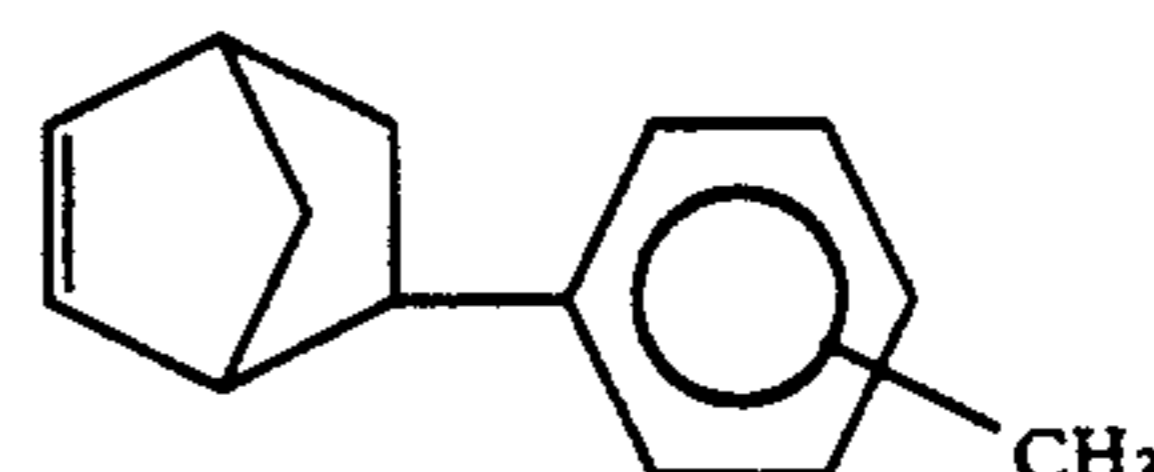
5-Tolylbicyclo[2.2.1]hept-2-ene
