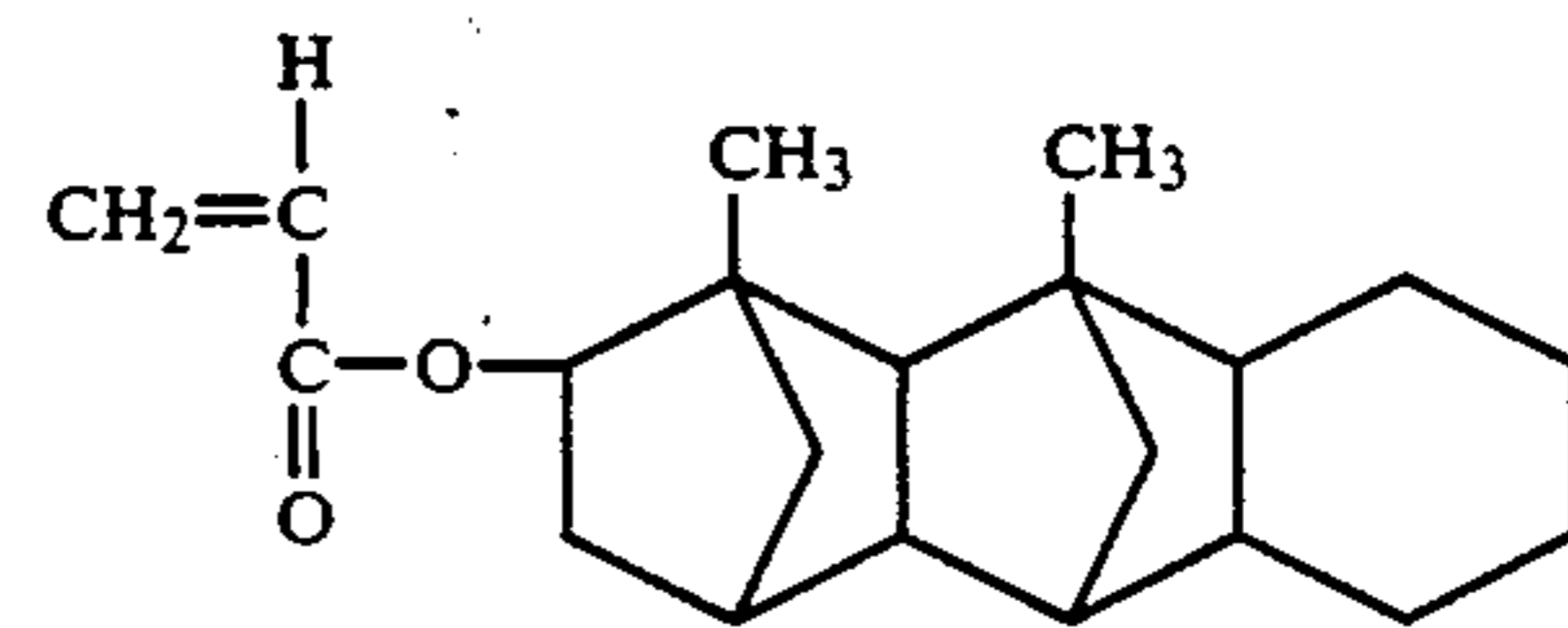
1,3-Dimethylpentacyclo[6.6.1.1 3 .6.0 2 .7.0 9 .14]hexadecyl-4-acrylate
