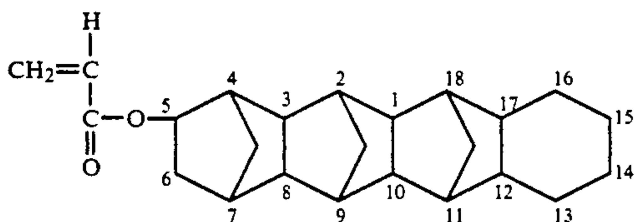
Octacyclo[8.8.1 2 .9.1 4 .7.1 11 .18.1 15 .16.0 3 .8.0 12 .17]docosyl-5-acrylate
