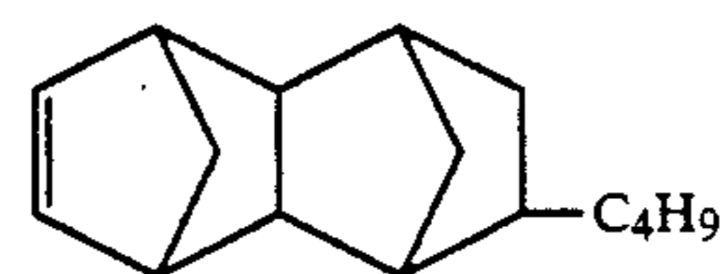
8-Butyltetracyclo[4.4.0.1 2,5 .1 7,10 ]-3-dodecene
