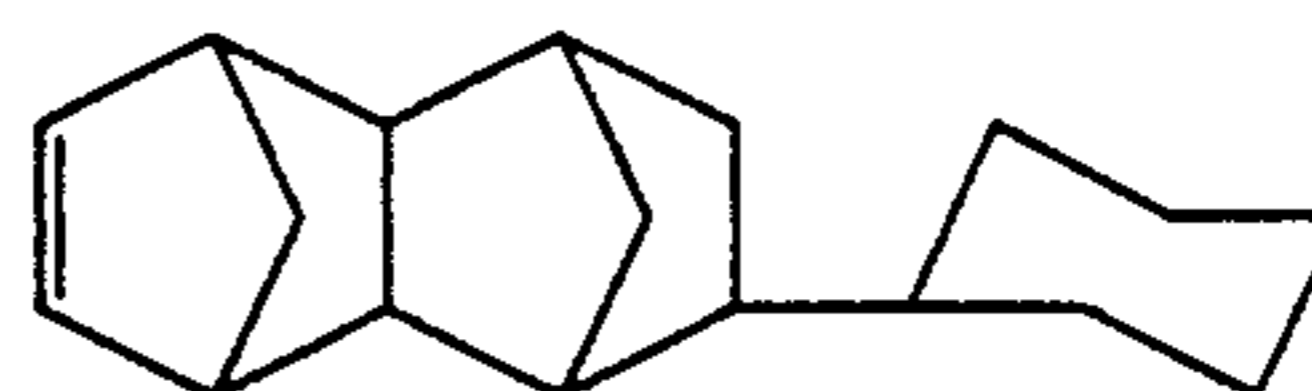
8-Cyclohexyltetracyclo[4.4.0.1 2,5 .1 7,10 ]-3-dodecene
