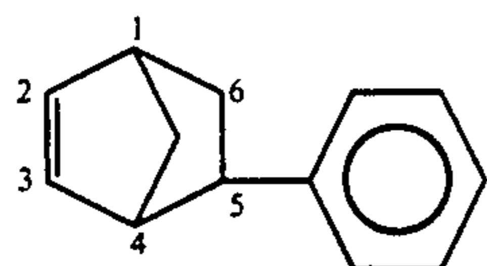
5-Phenylbicyclo[2.2.1]hept-2-ene
