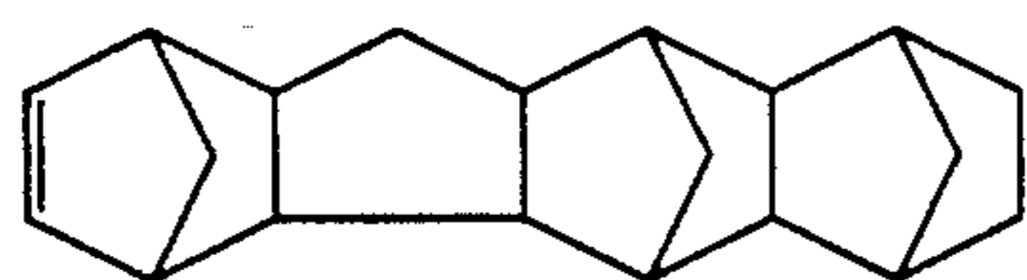
Heptacyclo[8.7.0.0 2.7.1 3.6.1 10.17.0 11.16.1 12.15 ]eicosene-4
