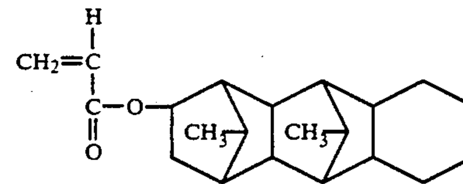
15,16-Dimethylpentacyclo[6.6.1.1.3.6.0.2.7.0.9.14]hexadecyl-4-acrylate
