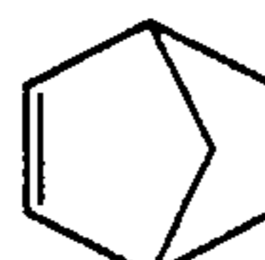
Bicyclo[2.2.1]hept-2-ene
