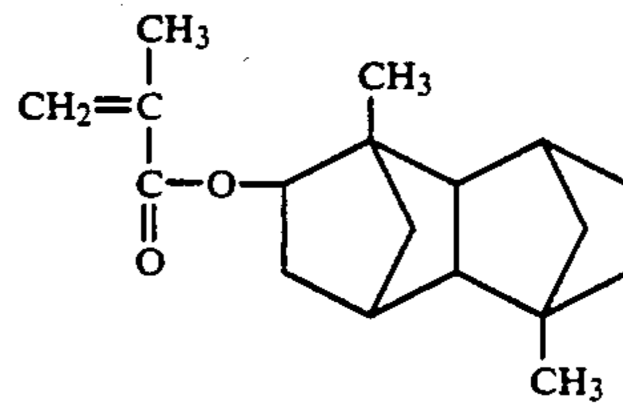
2,7-Dimethyltetracyclo[4.4.0.1 2,5 .1 7,10 ]-dodecyl-3-methacrylate
