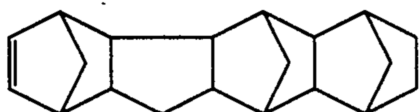
Heptacyclo[7.8.0.13.6.02.7.110.17.011.16.112.15]-4-eicosene
