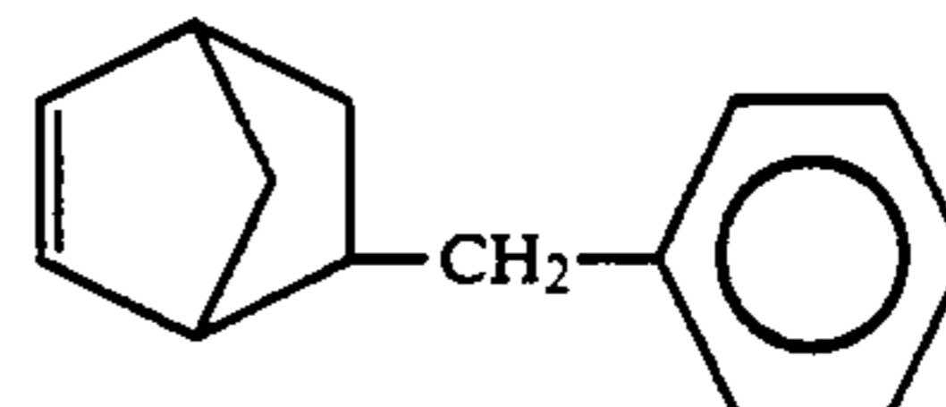
5-Benzylbicyclo[2.2.1]hept-2-ene
