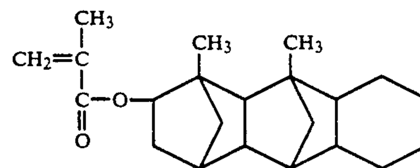
1,3-Dimethylpentacyclo[6.6.1.1.3.6.0.2.7.0.9.14]hexadecyl-4-methacrylate
