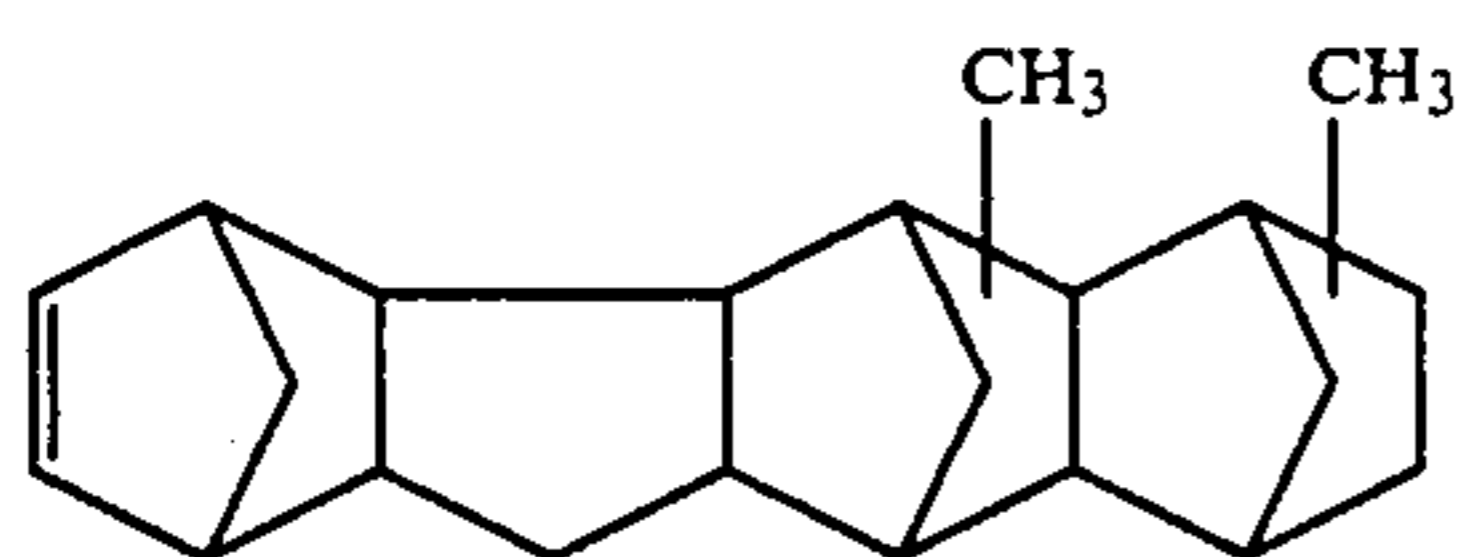
Dimethyl-substituted heptacyclo[7.8.0.13.6.02.7.110.17.011.16.112.15]-4-eicosene
