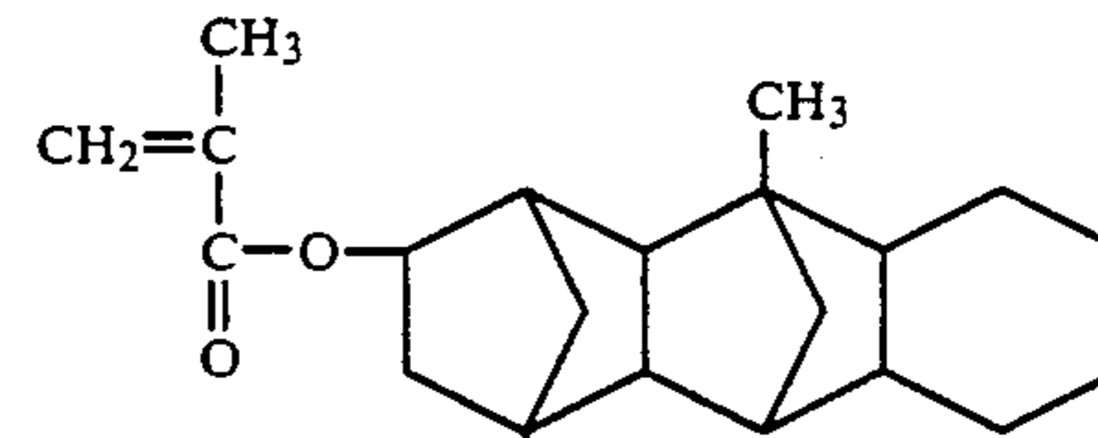
1,6-Dimethylpentacyclo[6.6.1.1.3.6.0.2.7.0.9.14]hexadecyl-4-methacrylate
