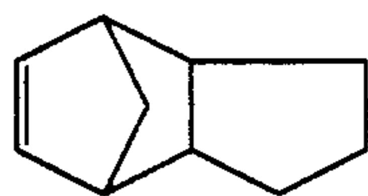
Tricyclo[4.3.0.1 2,5 ]-3-decene
