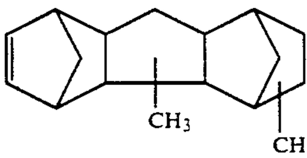
Dimethyl-pentacyclo[7.4.0.1 2.5.0 8.13.1 9.12 ]pentadecene-3
