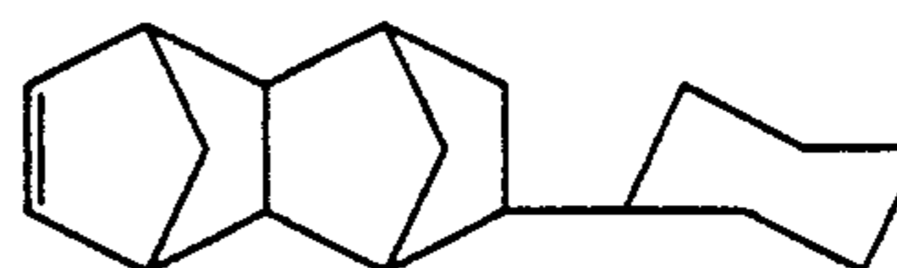
8-Cyclohexyltetracyclo[4.4.0.1 2,5 .1 7,10 ]-3-dodecene
