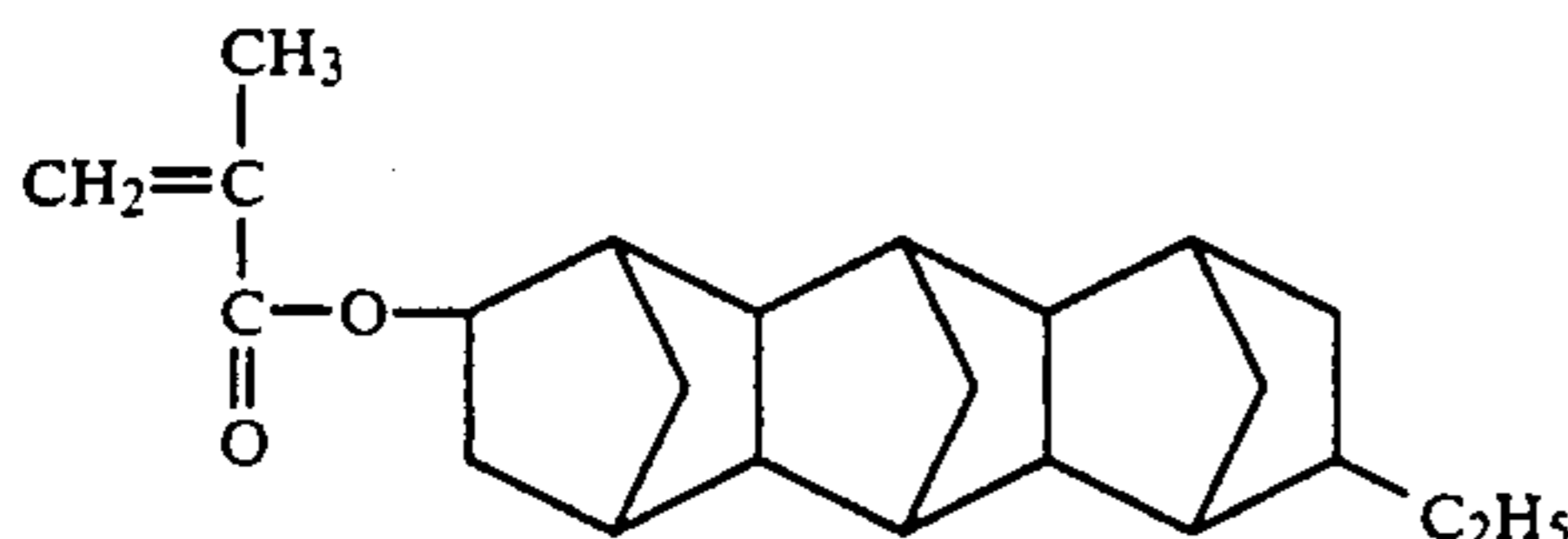
11-Ethylhexacyclo[6.6.1.1 3 .6.1 10 .13.0 2 .7.0 9 .14]-heptadecyl-4-methacrylate
