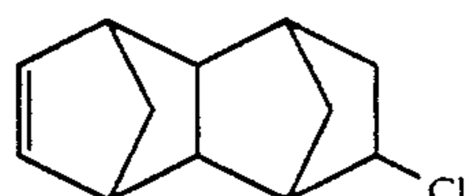
8-Chlorotetracyclo[4.4.0.1 2,5 .1 7,10 ]-3-dodecene
