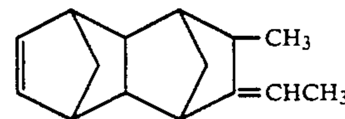
8-Ethylidene-9-methyltetracyclo[4.4.0.1 2,5 .1 7,10 ]-3-dodecene
