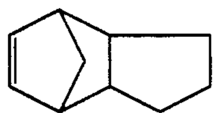
Tricyclo[4.3.0.1 2.5 ]-3-decene
