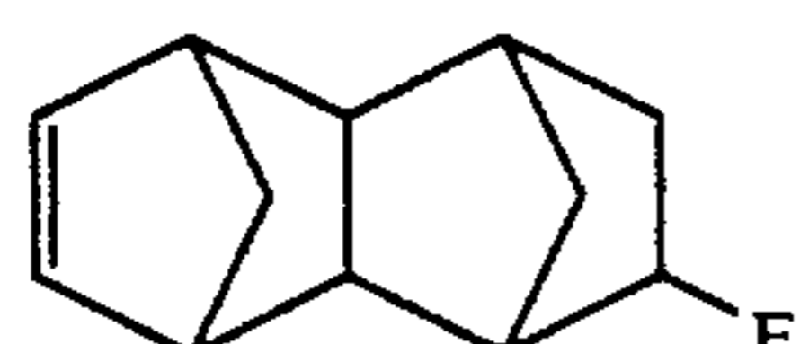
8-Fluorotetracyclo[4.4.0.1 2,5 .1 7,10 ]-3-dodecene
