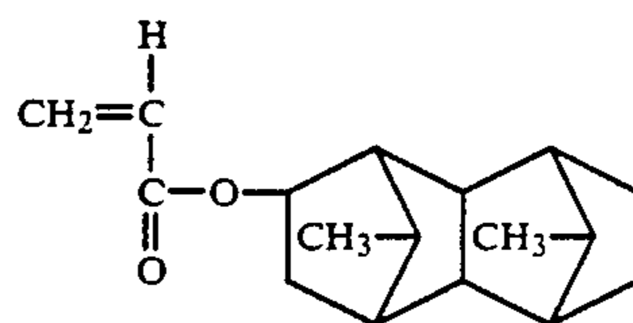
2,7-Dimethyltetracyclo[4.4.0.1 2,5 .1 7,10 ]-dodecyl-3-methacrylate
