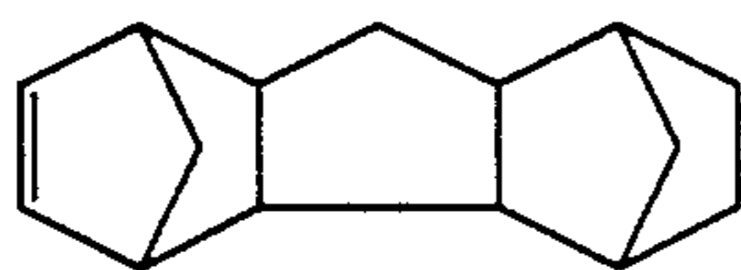
Pentacyclo[7.4.0.1 2.5.0 8.13.1 9.12 ]pentadecene-3
