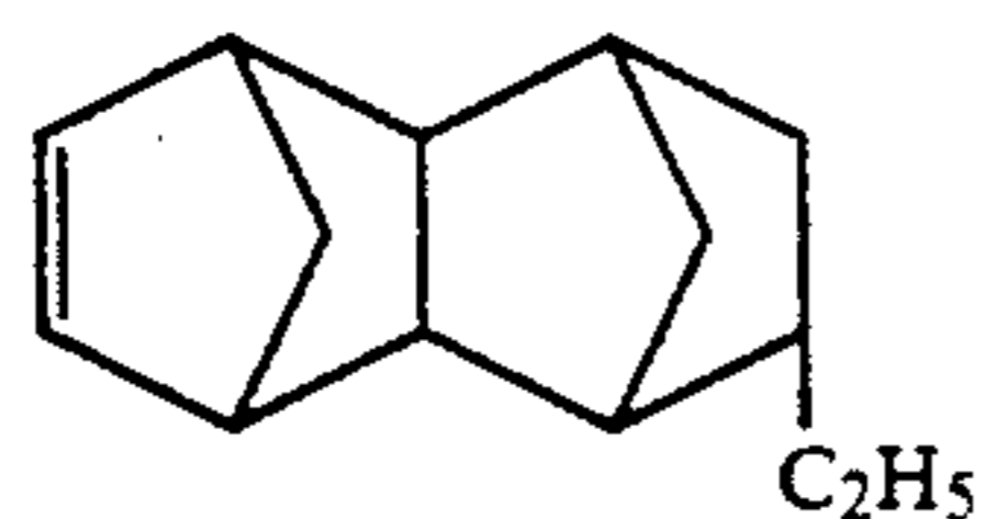
8-Ethyltetracyclo[4.4.0.1 2,5 .1 7,10 ]-3-dodecene
