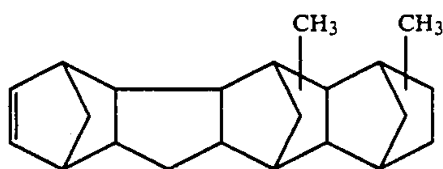
Dimethyl-substituted heptacyclo[7.8.0.13.6.02.7.110.17.011.16.112.15]-4-eicosene
