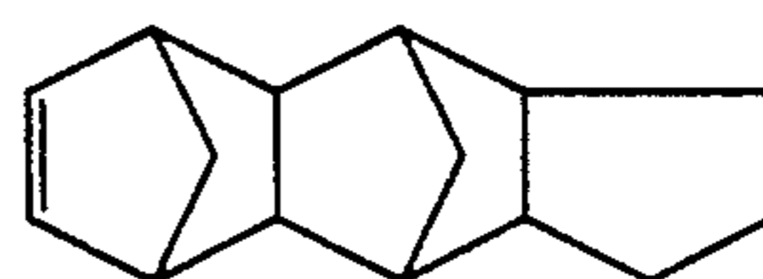
Pentacyclo[6.5.1.1 3 .6.0 2 .7.0 9 .13]-4-pentadecene
