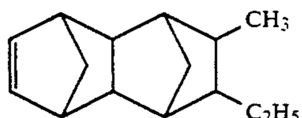
8-Methyl-9-ethyltetracyclo[4.4.0.1 2,5 .1 7,10 ]-3-dodecene
