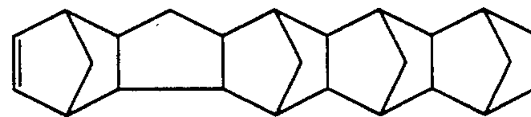
Nonacyclo[10.9.1.0 2.10.0 3.8.1 4.7.0 12.21.1 13.20.0 14.19.1 15.18 ]pentacosene-5
