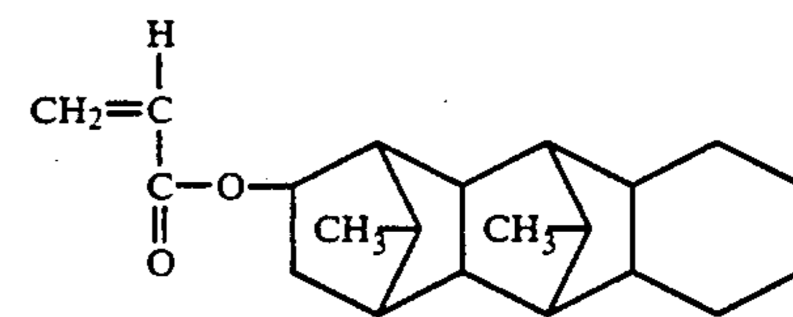
15,16-Dimethylpentacyclo[6.6.1.1 3 .6.0 2 .7.0 9 .14]hexadecyl-4-acrylate
