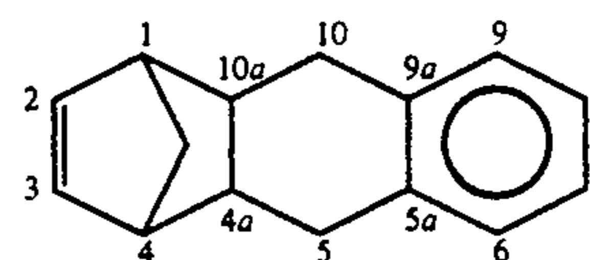
1,4-Methano-1,4,4a,5,10,10a-hexahydroanthracene
