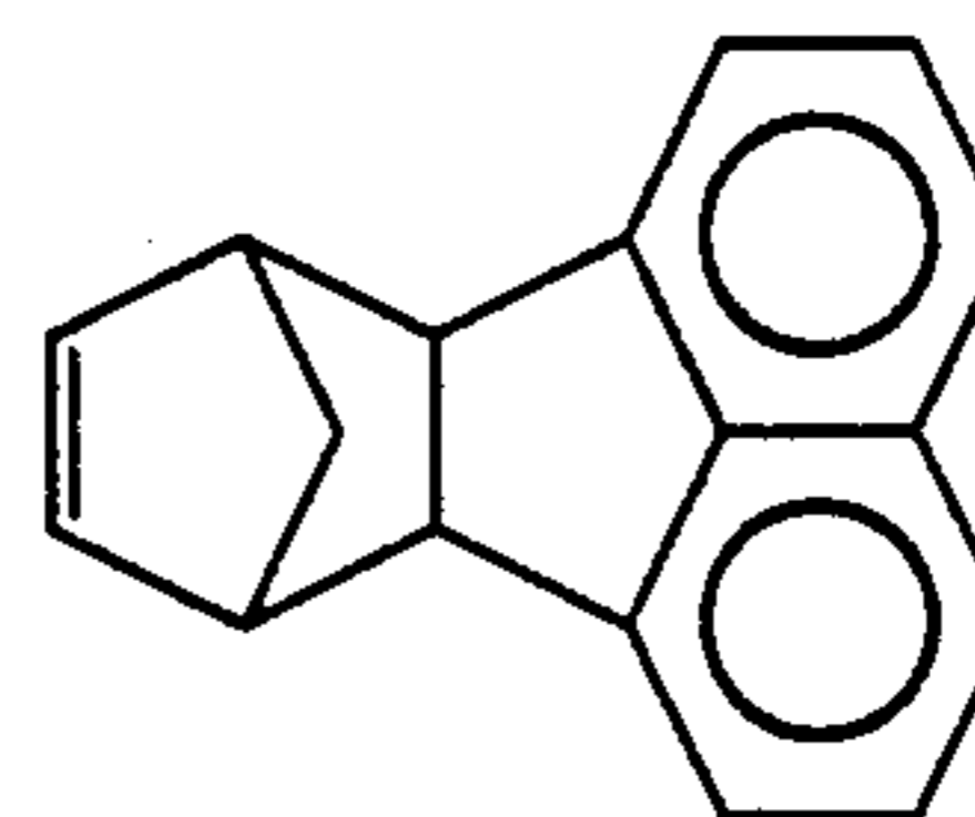
Cyclopentadiene-acenaphthylene adduct
