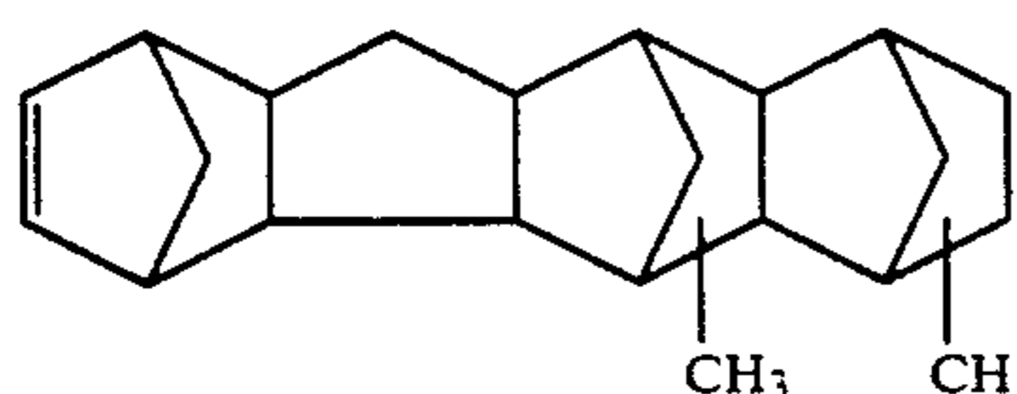
Dimethyl-heptacyclo[8.7.0.0 2.7.1 3.6.1 10.17.0 11.16.1 12.15 ]eicosene-4
