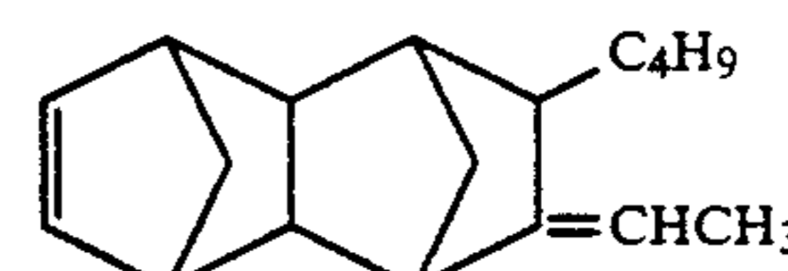
8-Ethylidene-9-butyltetracyclo[4.4.0.1 2,5 .1 7,10 ]-3-dodecene
