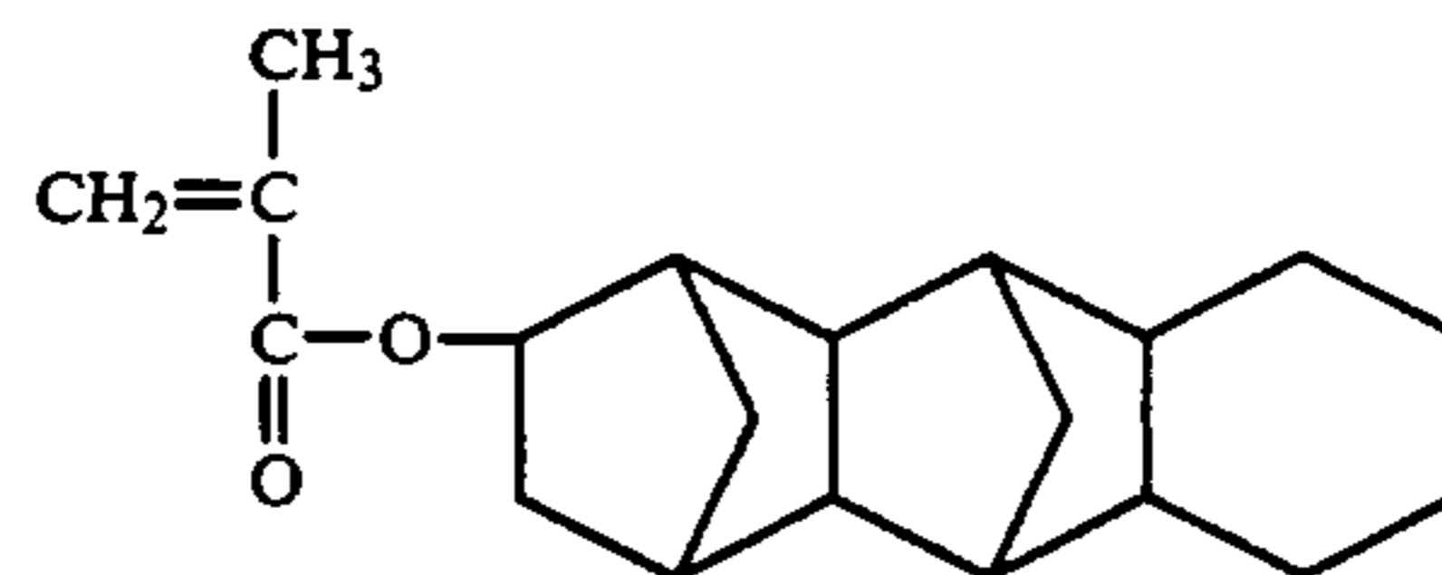
Pentacyclo[6.6.1.1.3.6.0.2.7.0.9.14]-hexadecyl-4-methacrylate
