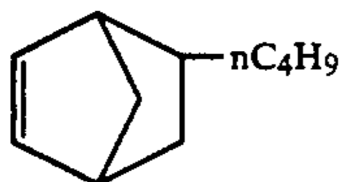
6-n-Butylbicyclo[2.2.1]hept-2-ene
