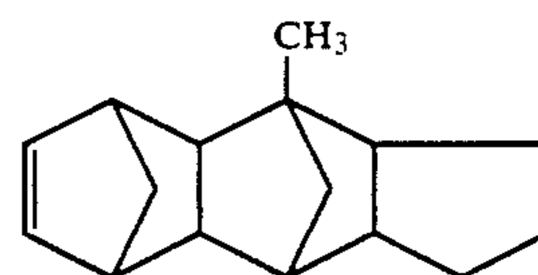
1,6-Dimethylpentacyclo[6.5.1.1 3 .6.0 2 .7.0 9 .13]-4-pentadecene
