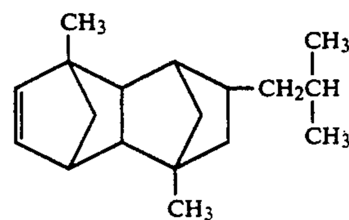
9-Isobutyl-2,7-dimethyltetracyclo[4.4.0.1 2,5 .1 7,10 ]-3-dodecene
