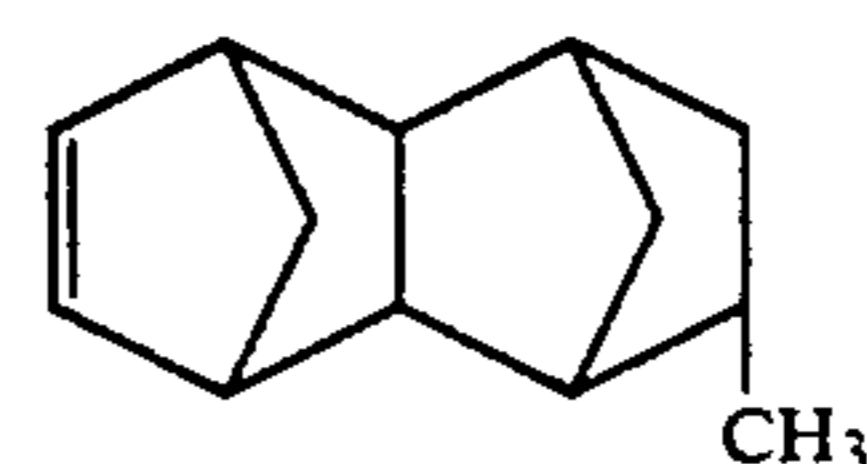
8-Methyltetracyclo[4.4.0.1 2,5 .1 7,10 ]-3-dodecene
