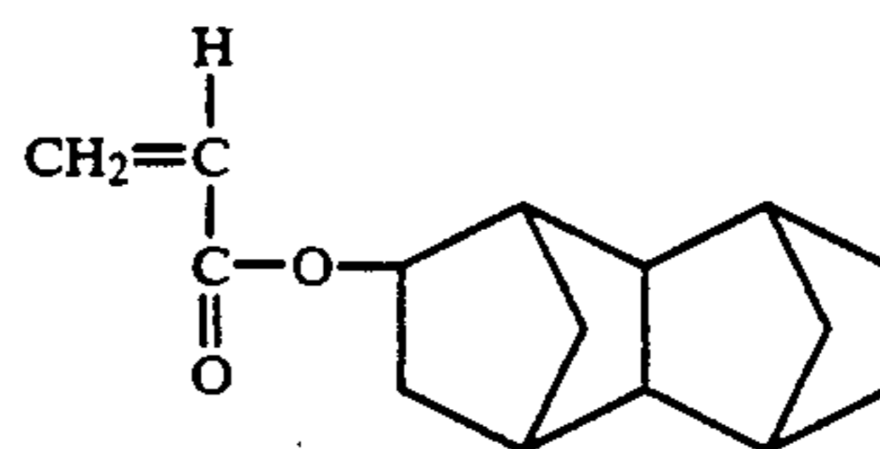
Tetracyclo[4.4.0.1 2,5 .1 7,10 ]-dodecyl-3-acrylate
