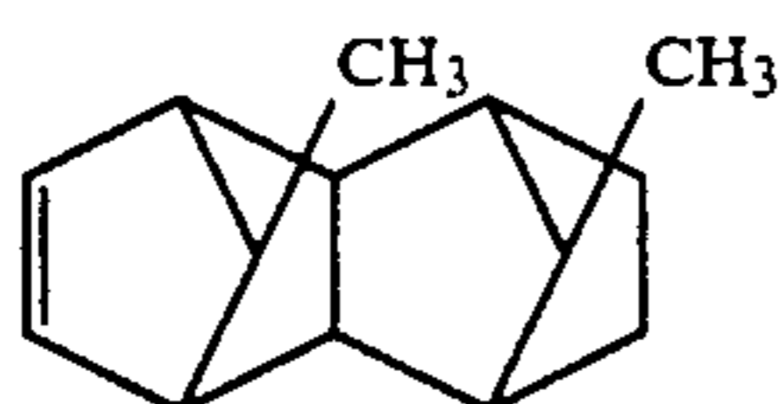
11,12-Dimethyltetracyclo[4.4.0.1 2,5 .1 7,10 ]-3-dodecene
