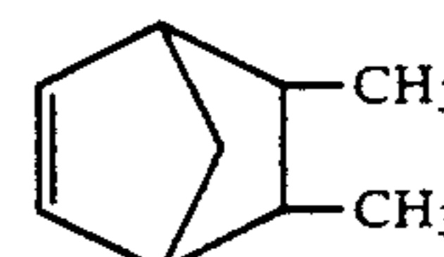
5,6-Dimethylbicyclo[2.2.1]hept-2-ene
