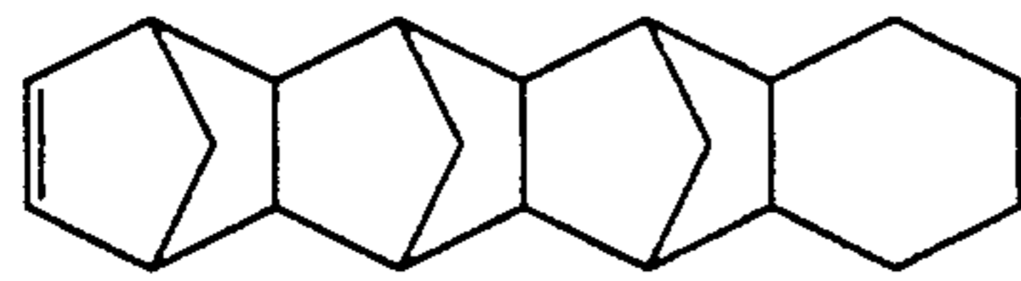
Heptacyclo[8.7.0.1 2 .9.14.7.11.18.0 3 .8.0 12 .17]-5-heneicosene
