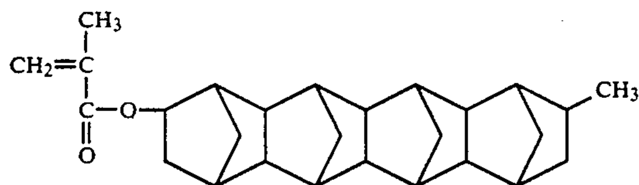
15-Methyloctacyclo[8.8.12.9.14.7.11.18.15.16.0.3.8.0.12.17]docosyl-5-methacrylate
