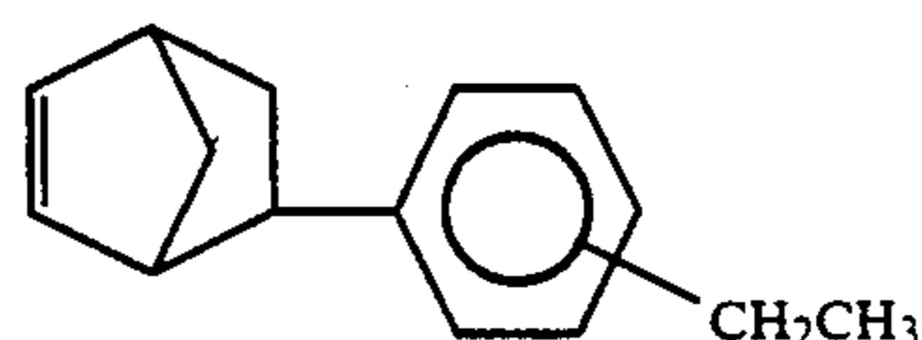
5-(Ethylphenyl)bicyclo[2.2.1]hept-2-ene
