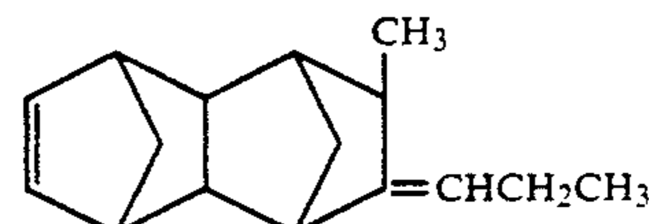
8-n-Propylidenetetracyclo[4.4.0.1 2,5 .1 7,10 ]-3-dodecene
