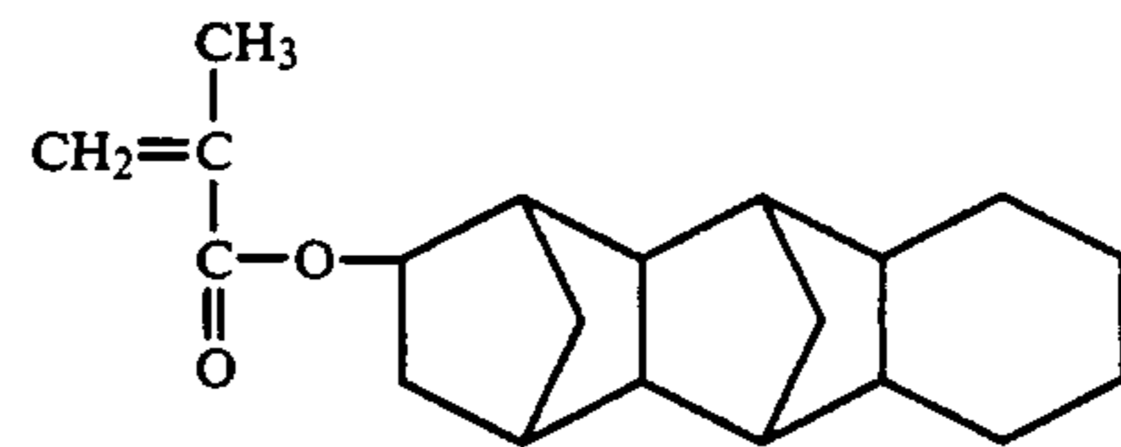
Pentacyclo[6.6.1.1 3 .6.0 2 .7.0 9 .14]-hexadecyl-4-methacrylate
