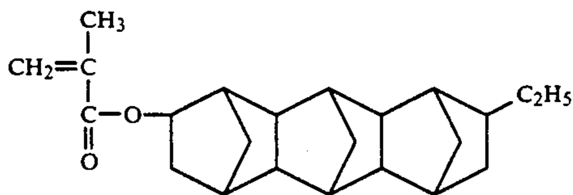
12-Ethylhexacyclo[6.6.1.1.3.6.10.13.0.2.7.0.9.14]-heptadecyl-4-methacrylate
