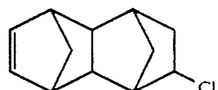
8-Chlorotetracyclo[4.4.0.1 2,5 .1 7,10 ]-3-dodecene
