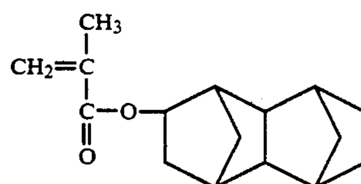
Tetracyclo[4.4.0.1 2,5 .1 7,10 ]-dodecyl-3-methacrylate
