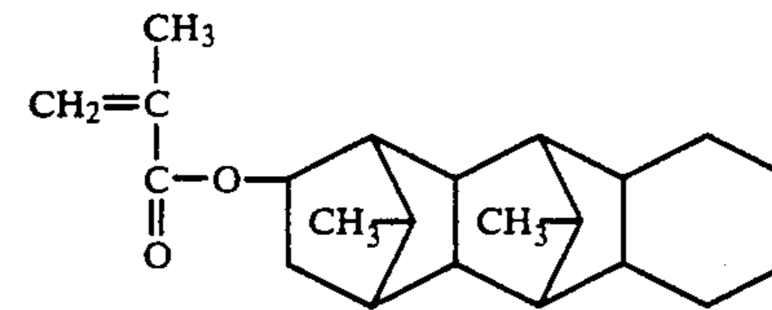
15,16-Dimethylpentacyclo-
