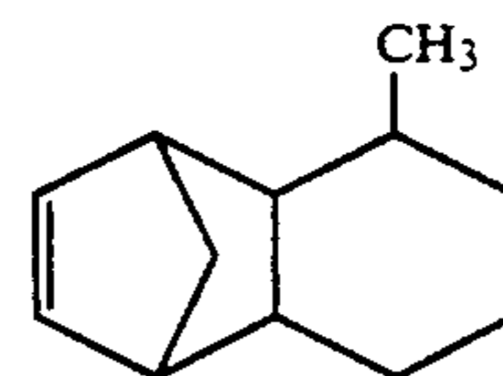
10-Methyltricyclo[4.4.0.1 2,5 ]-3-undecene
