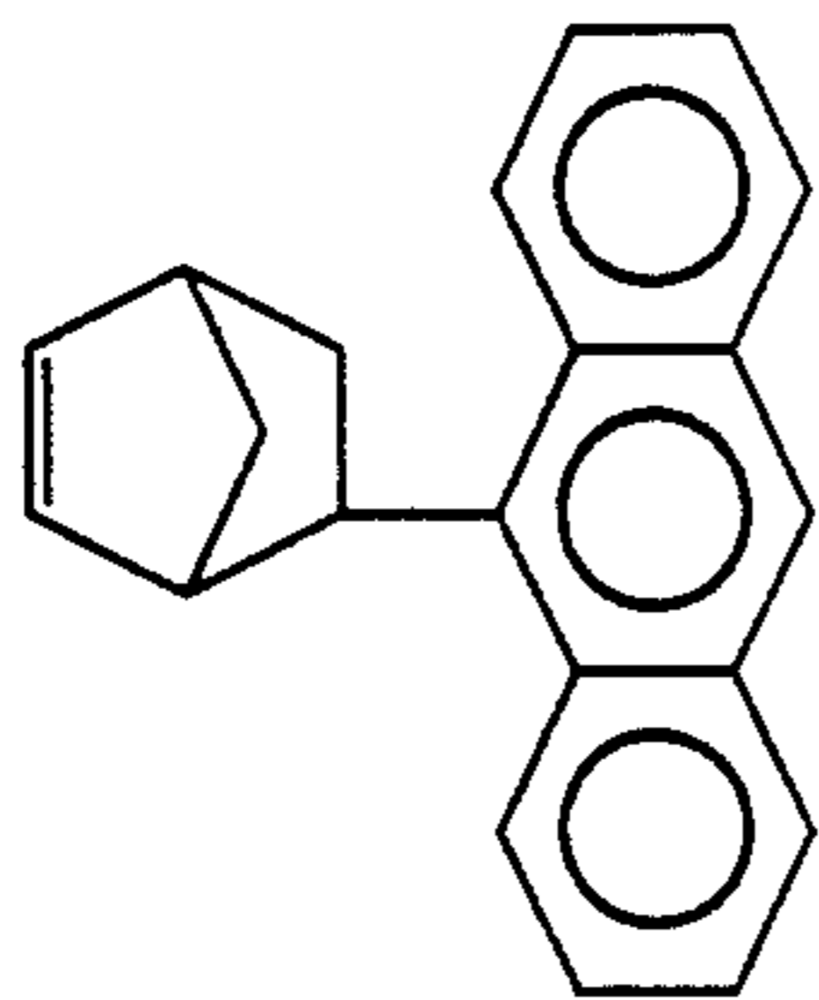
5-(Anthracenyl)bicyclo[2.2.1]hept-2-ene
