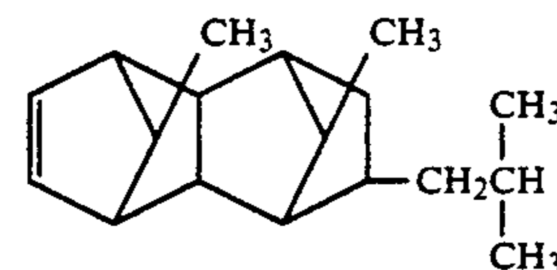
9-Isobutyl-11,12-dimethyltetracyclo[4.4.0.1 2,5 .1 7,10 ]-3-dodecene
