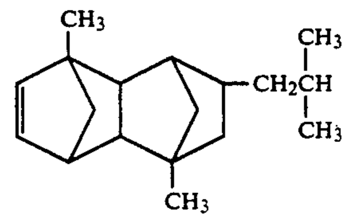
9-Isobutyl-2,7-dimethyltetracyclo[4.4.0.1 2,5 .1 7,10 ]-3-dodecene
