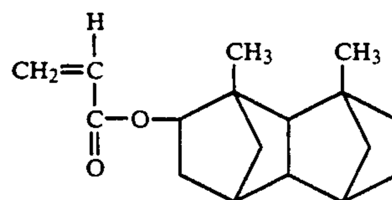
2,10-Dimethyltetracyclo[4.4.0.1 2,5 .1 7,10 ]-dodecyl-3-acrylate
