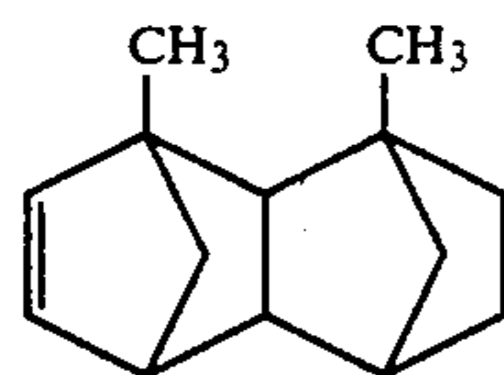
2,10-Dimethyltetracyclo[4.4.0.1 2,5 .1 7,10 ]-3-dodecene
