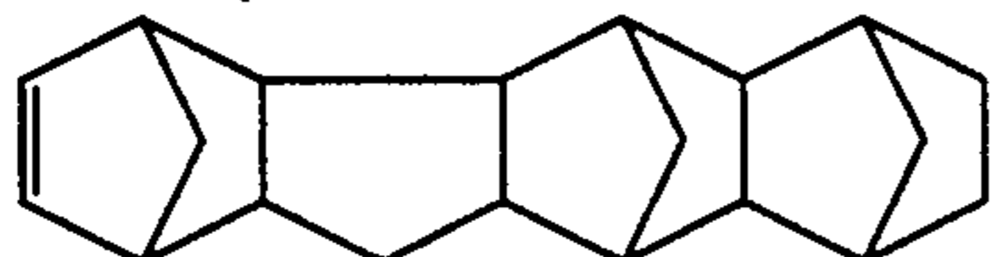
Heptacyclo[7.8.0.13.6.02.7.110.17.011.16.112.15]-4-eicosene
