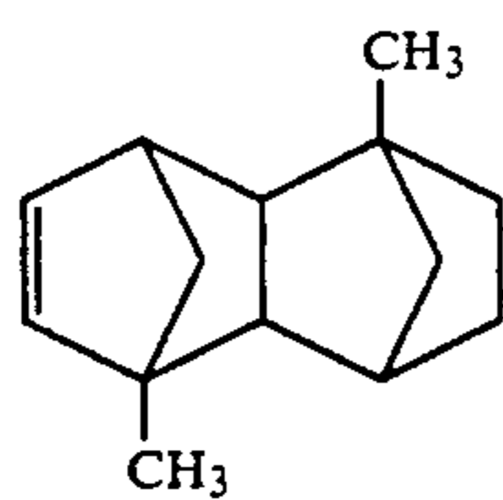
5,10-Dimethyltetracyclo[4.4.0.1 2,5 .1 7,10 ]-3-dodecene
