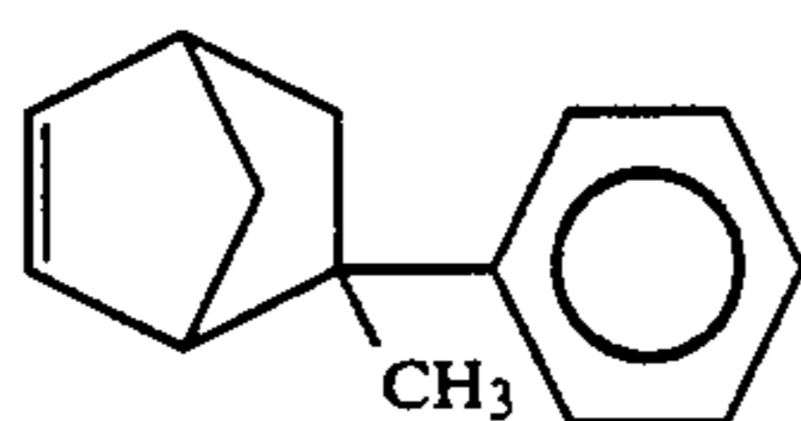
5-Methyl-5-phenylbicyclo[2.2.1]hept-2-ene
