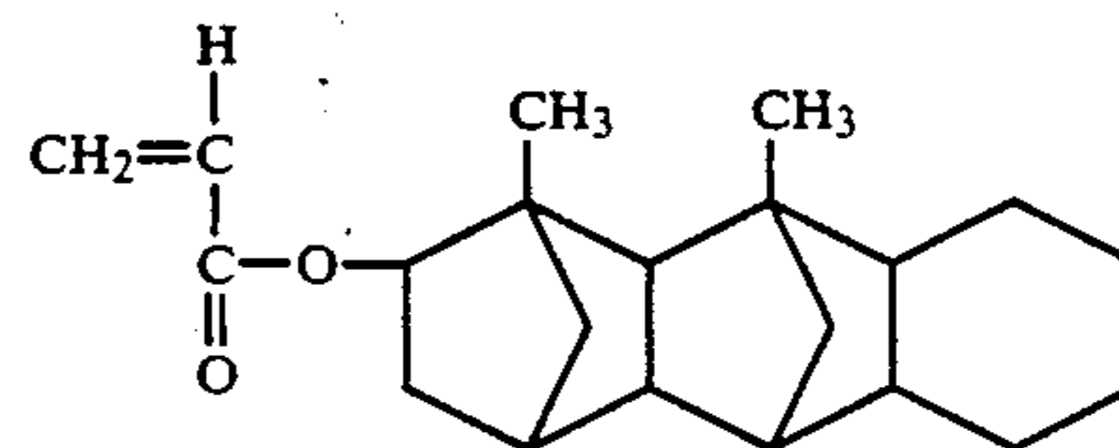
1,3-Dimethylpentacyclo[6.6.1.1.3.6.0.2.7.0.9.14]hexadecyl-4-acrylate
