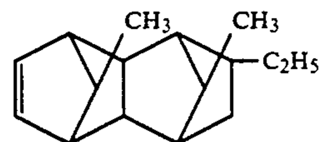
9-Ethyl-11,12-dimethyltetracyclo[4.4.0.1 2,5 .1 7,10 ]-3-dodecene
