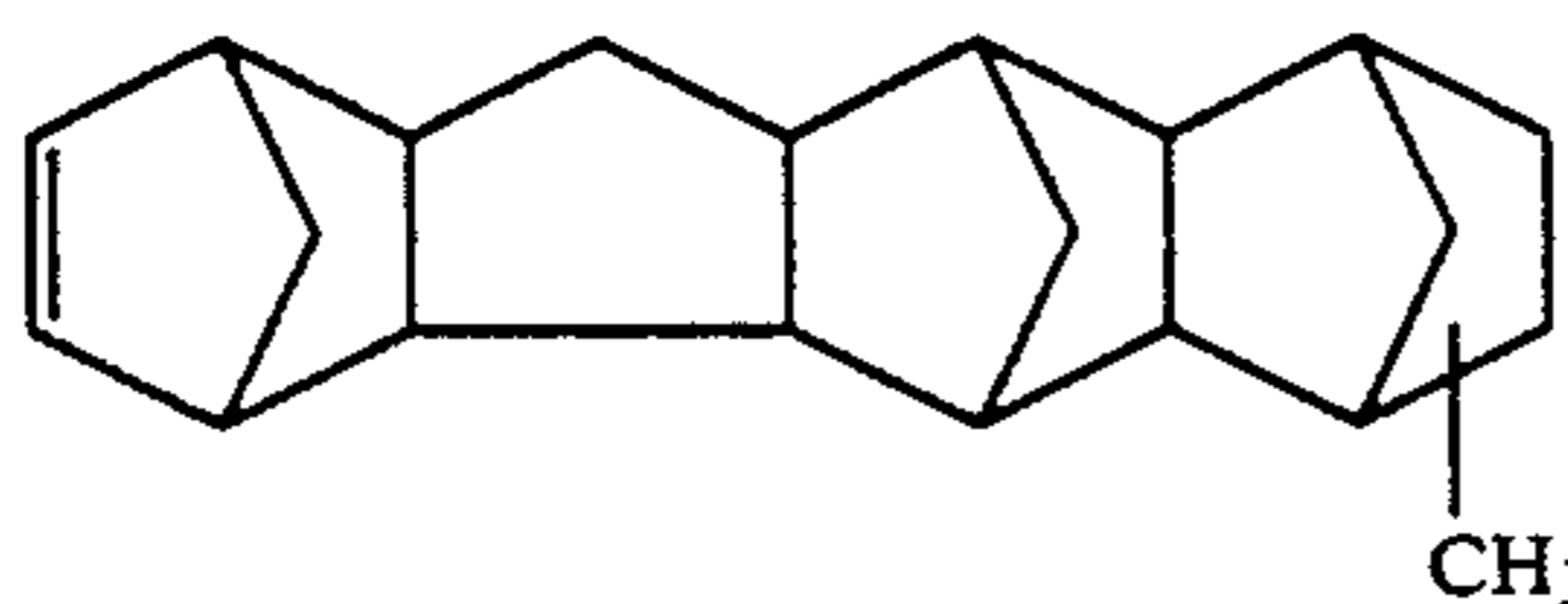
Methyl-heptacyclo[8.7.0.0 2.7.1 3.6.1 10.17.0 11.16.1 12.15 ]eicosene-4
