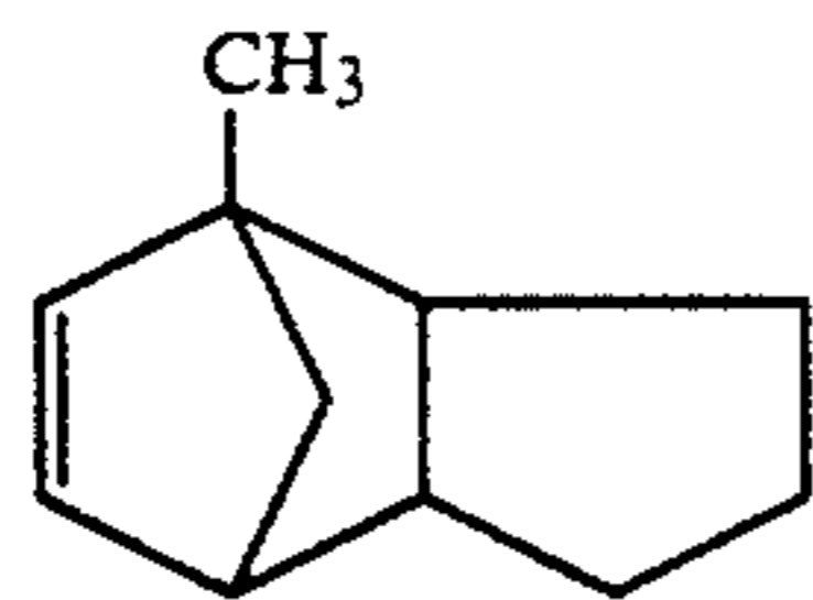
2-Methyltricyclo[4.3.0.1 2.5 ]-3-decene
