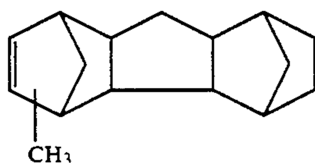
Methyl-pentacyclo[7.4.0.1 2.5.0 8.13.1 9.12 ]pentadecene-3
