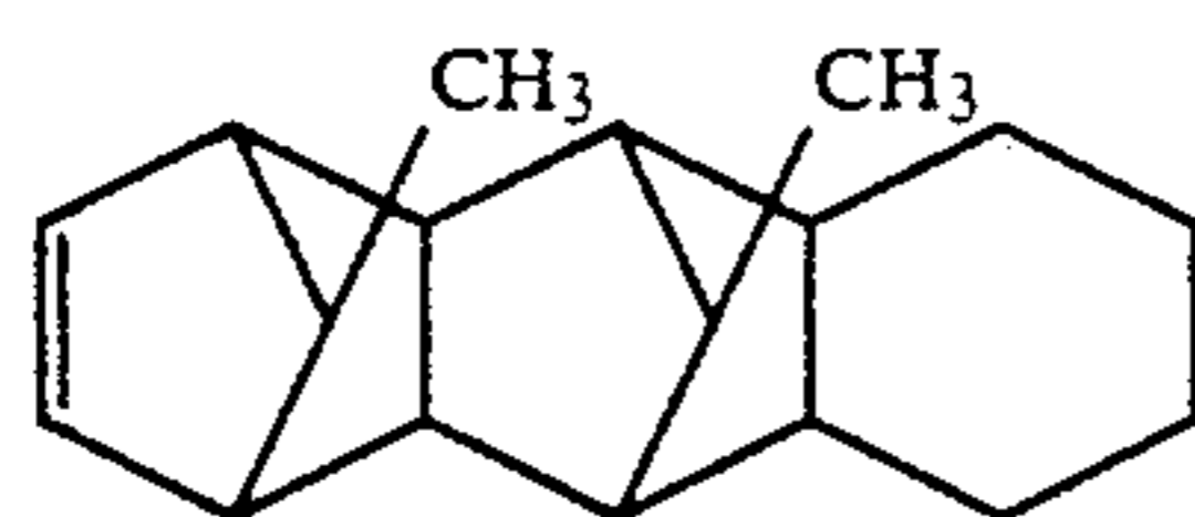
15,16-Dimethylpentacyclo[6.6.1.1.3.6.0.2.7.0.9.14]-4-hexadecene
