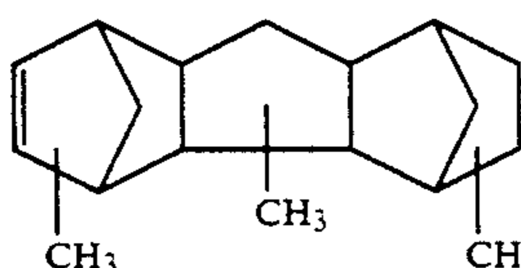
Trimethylpentacyclo[7.4.0.1 2.5.0 8.13.1 9.12 ]pentadecene-3
