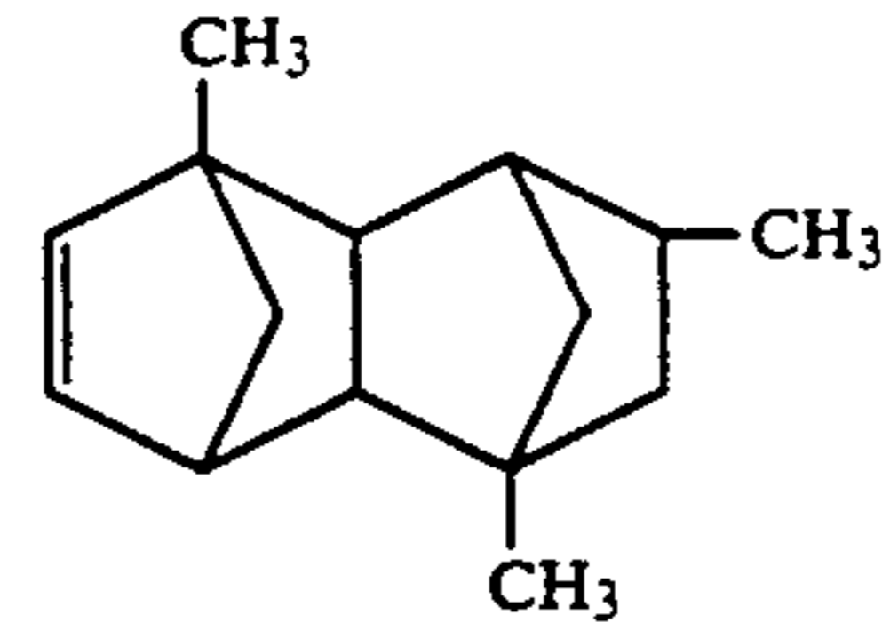
2,7,9-Trimethyltetracyclo[4.4.0.1 2,5 .1 7,10 ]-3-dodecene
