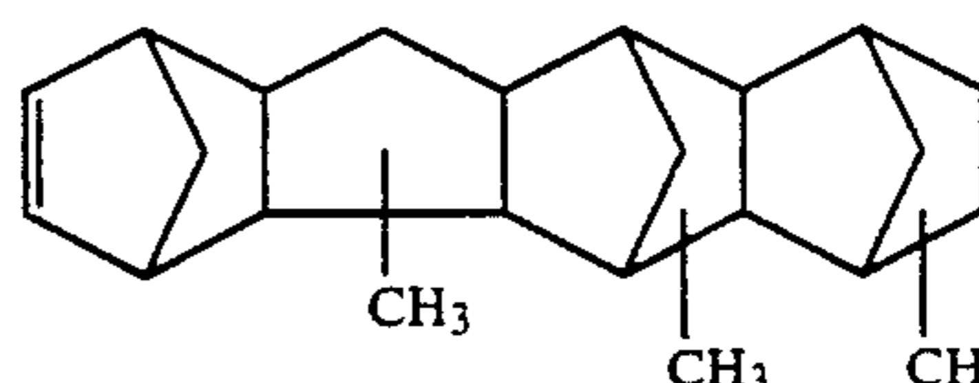
Trimethyl-heptacyclo[8.7.0.0 2.7.1 3.6.1 10.17.0 11.16.1 12.15 ]eicosene-4
