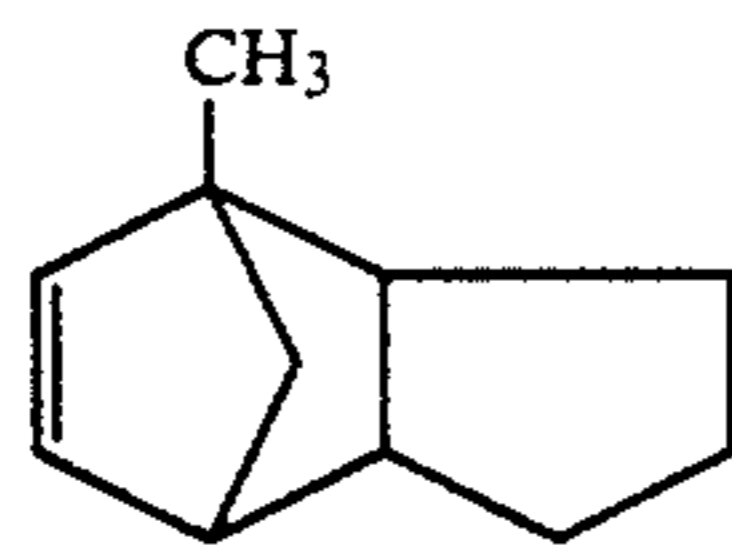
2-Methyltricyclo[4.3.0.1 2,5 ]-3-decene
