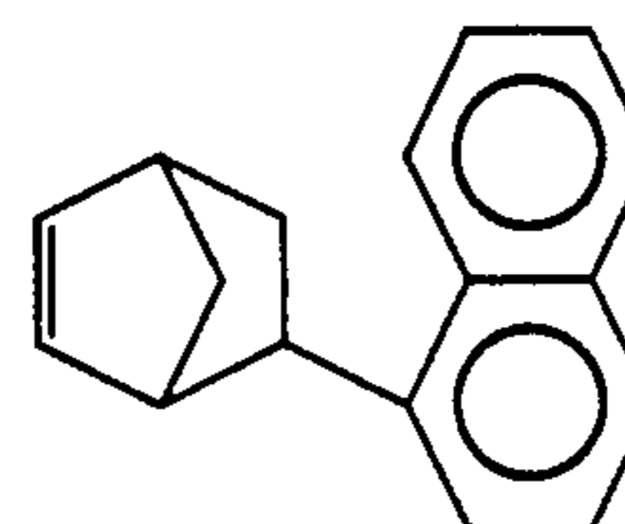
5-( \alpha -Naphthyl)bicyclo[2.2.1]hept-2-ene
