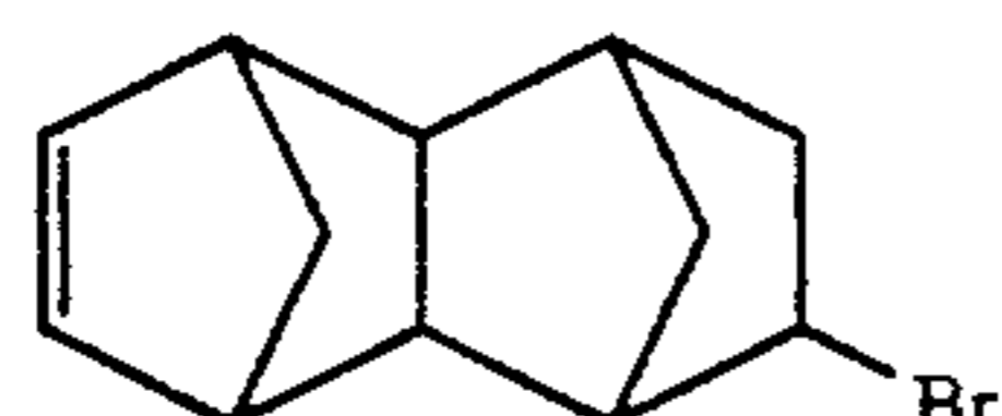
8-Bromotetracyclo[4.4.0.1 2,5 .1 7,10 ]-3-dodecene
