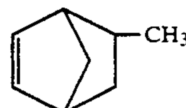
6-Methylbicyclo[2.2.1]hept-2-ene
