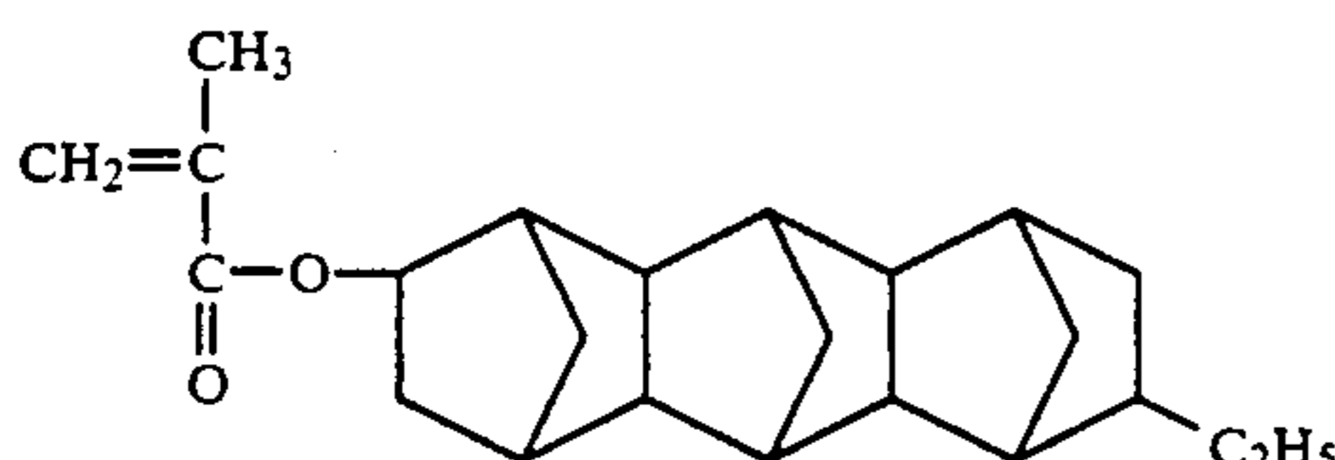
11-Ethylhexacyclo[6.6.1.1.3.6.10.13.0.2.7.0.9.14]-heptadecyl-4-methacrylate
