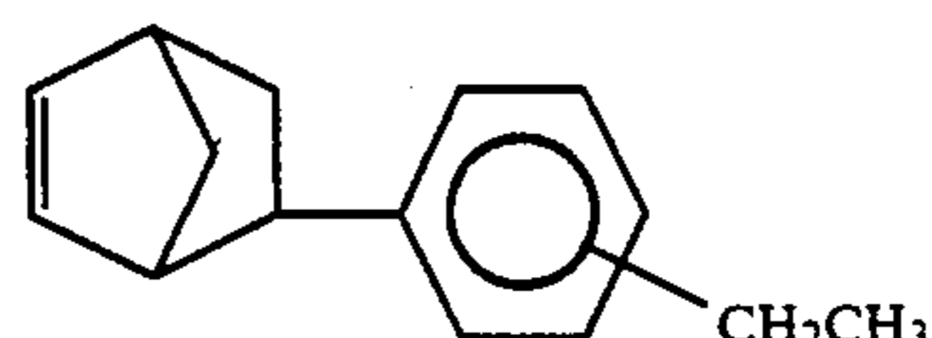
5-(Ethylphenyl)bicyclo[2.2.1]hept-2-ene
