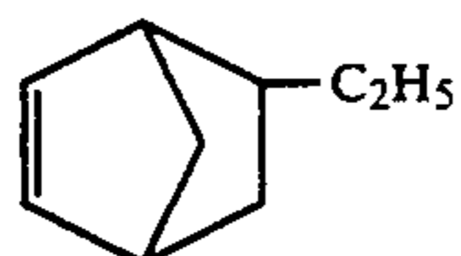
6-Ethylbicyclo[2.2.1]hept-2-ene
