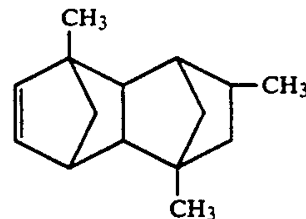
2,7,9-Trimethyltetracyclo[4.4.0.1 2,5 .1 7,10 ]-3-dodecene
