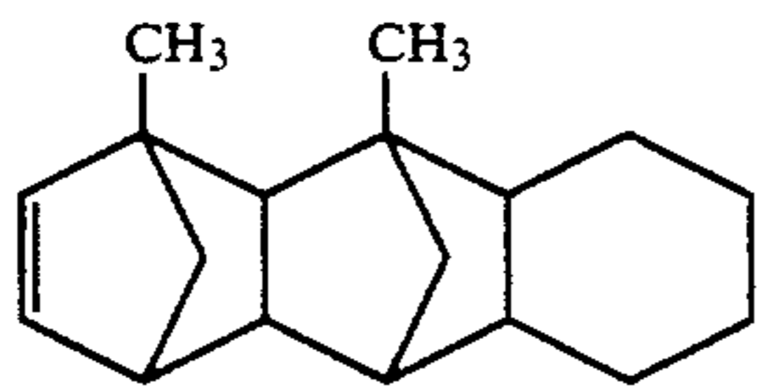
1,3-Dimethylpentacyclo[6.6.1.1.3.6.0.2.7.0.9.14]-4-hexadecene
