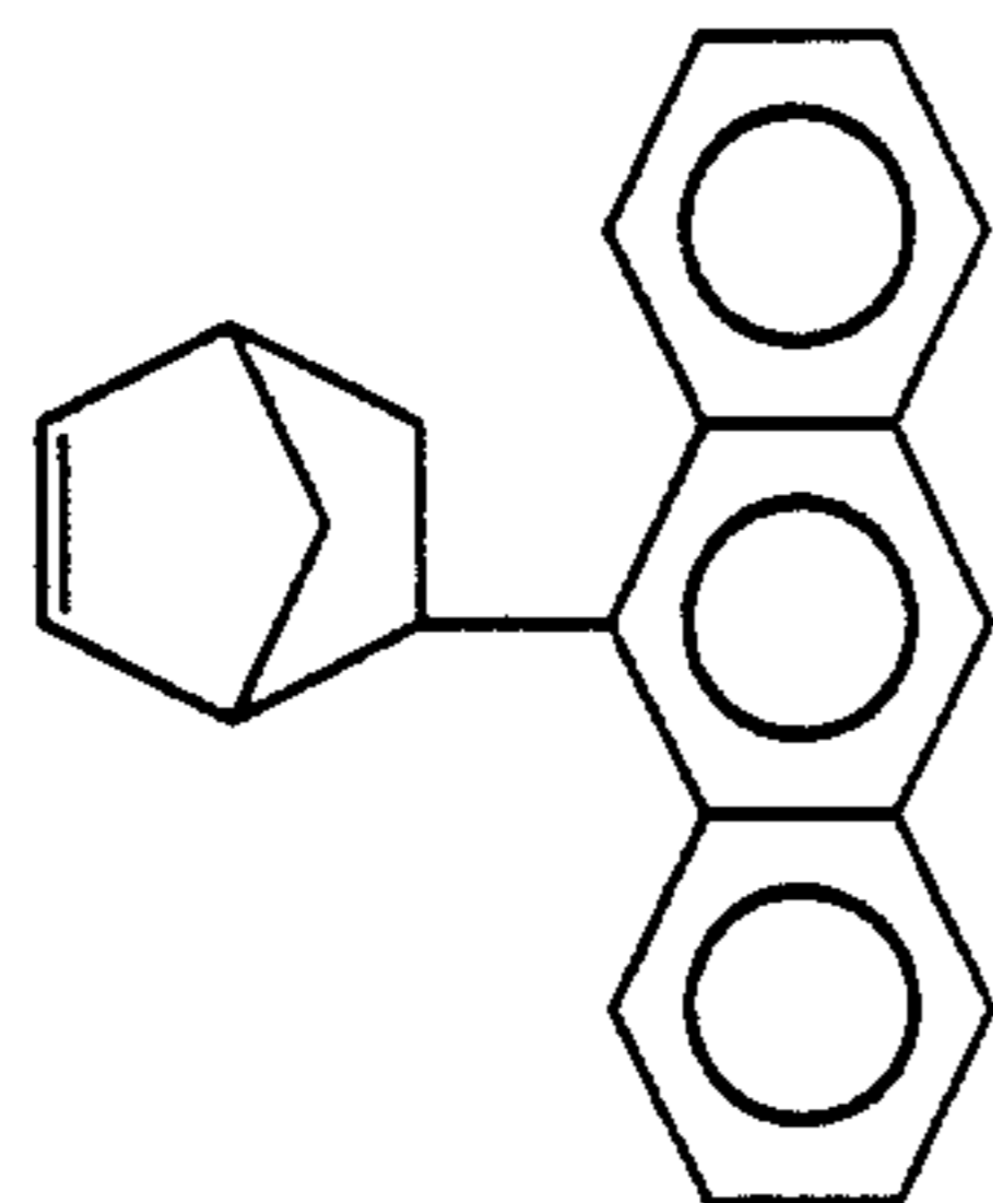
5-(Anthracenyl)bicyclo[2.2.1]hept-2-ene
