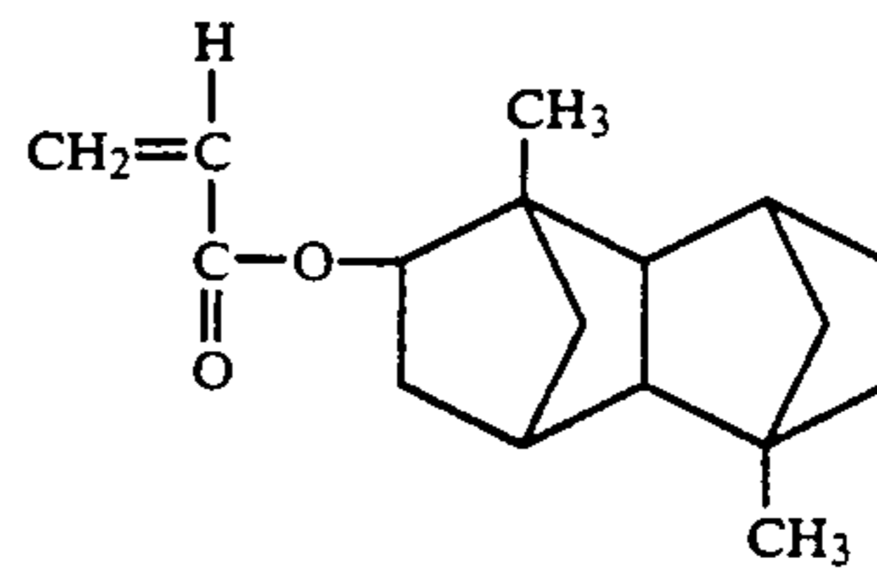
2,7-Dimethyltetracyclo[4.4.0.1 2,5 .1 7,10 ]-dodecyl-3-acrylate
