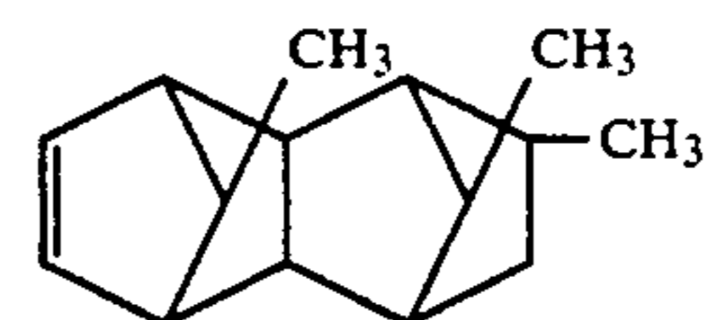
9,11,12-Trimethyltetracyclo[4.4.0.1 2,5 .1 7,10 ]-3-dodecene
