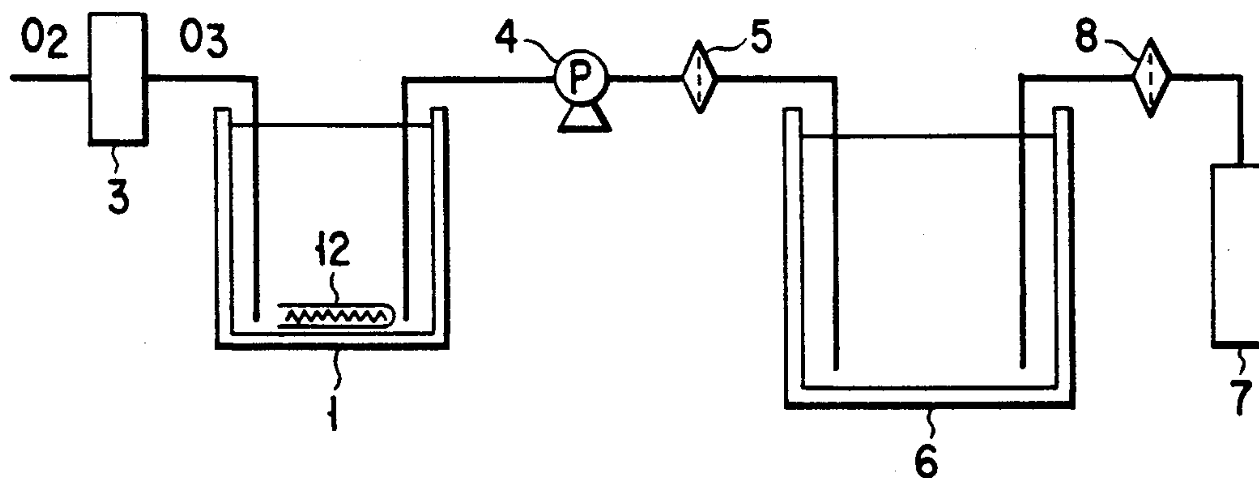
FIG. 6 (PRIOR ART)
