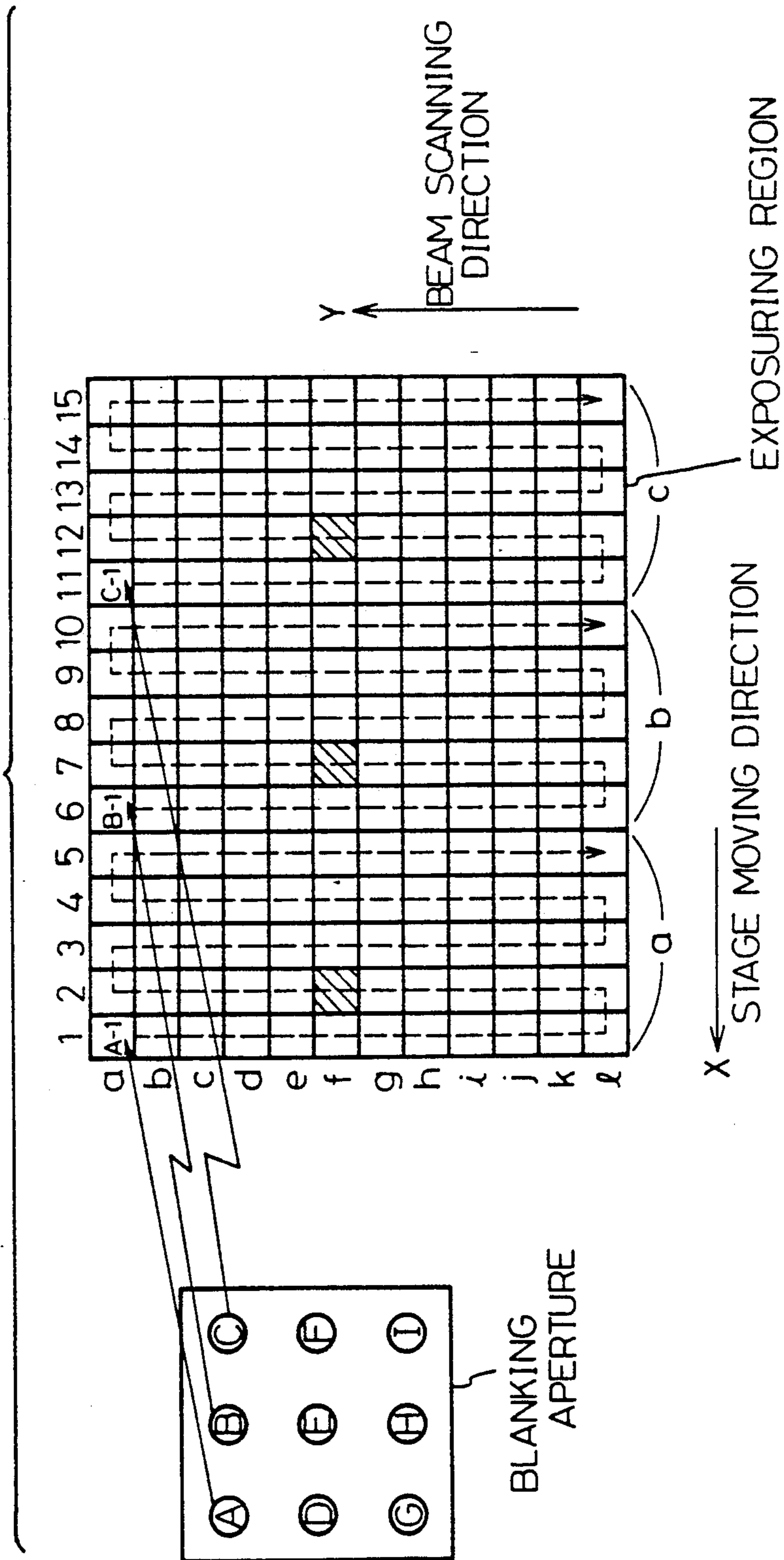
Fig. 20 PRIOR ART
