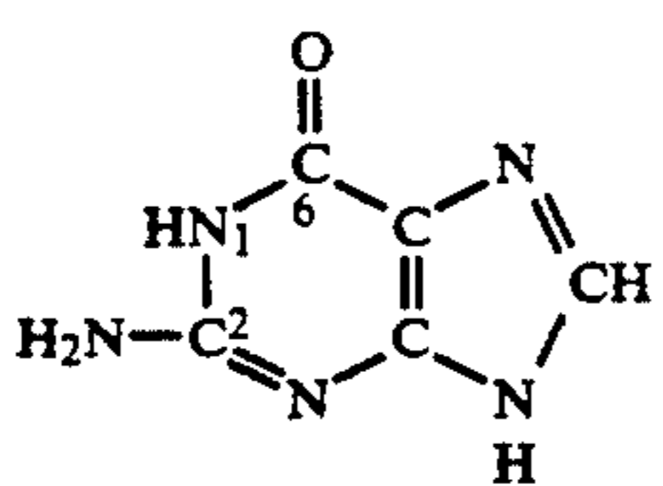
Guanine (2-amino-6-oxypurine)
