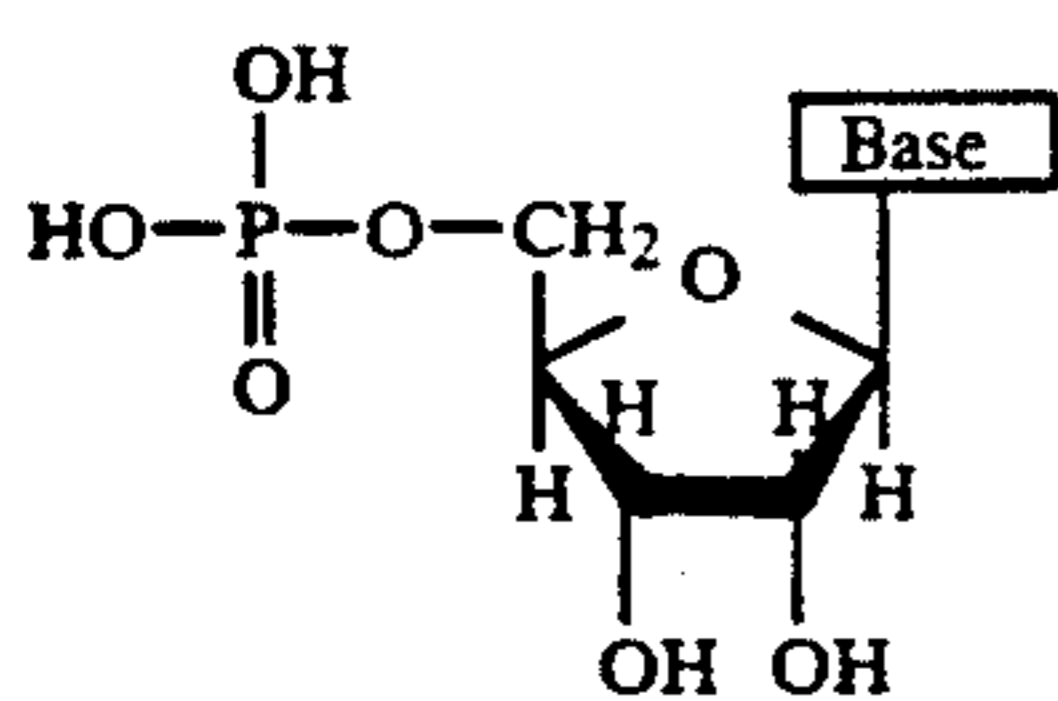
Ribonucleoside 5'-monophosphates
