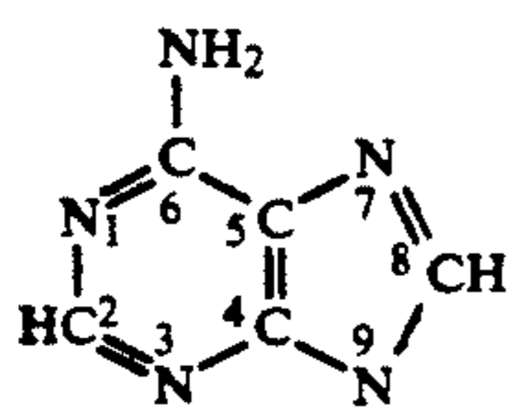
Adenine (6-aminopurine)
