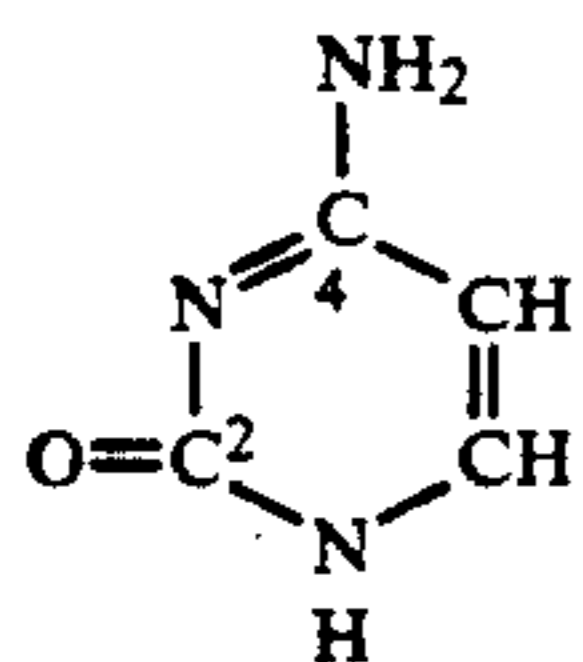
Cytosine (2-oxy-4-aminopyrimidine)
