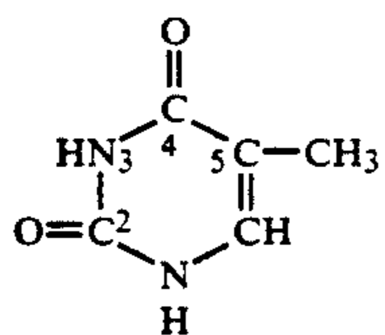
Thymine (5-methyl-2,4-dioxypyrimidine)
