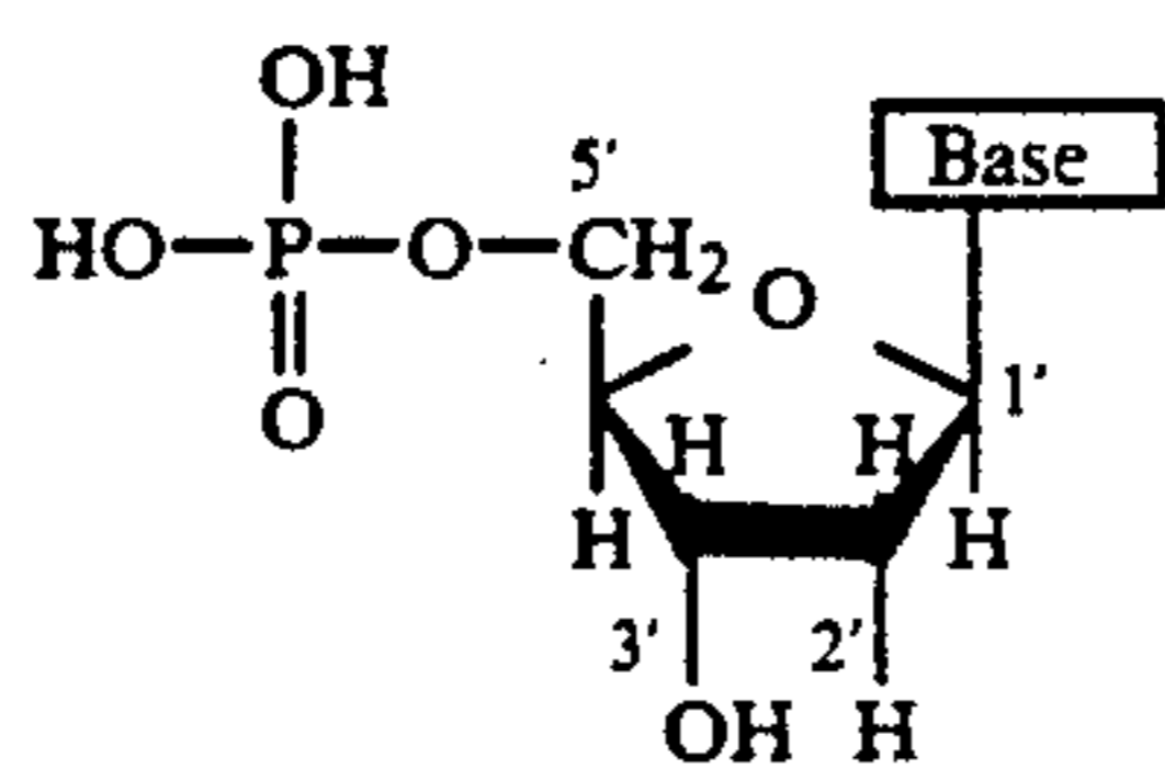
2'-Deoxyribonucleoside 5'-monophosphates
