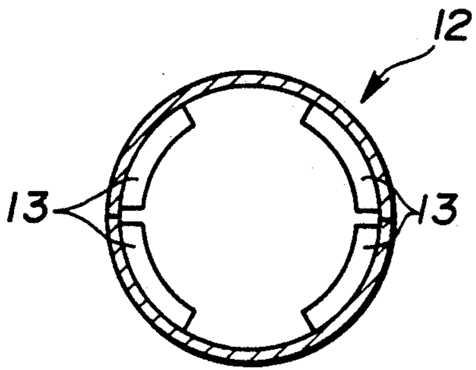
FIG. 7 PRIOR ART
