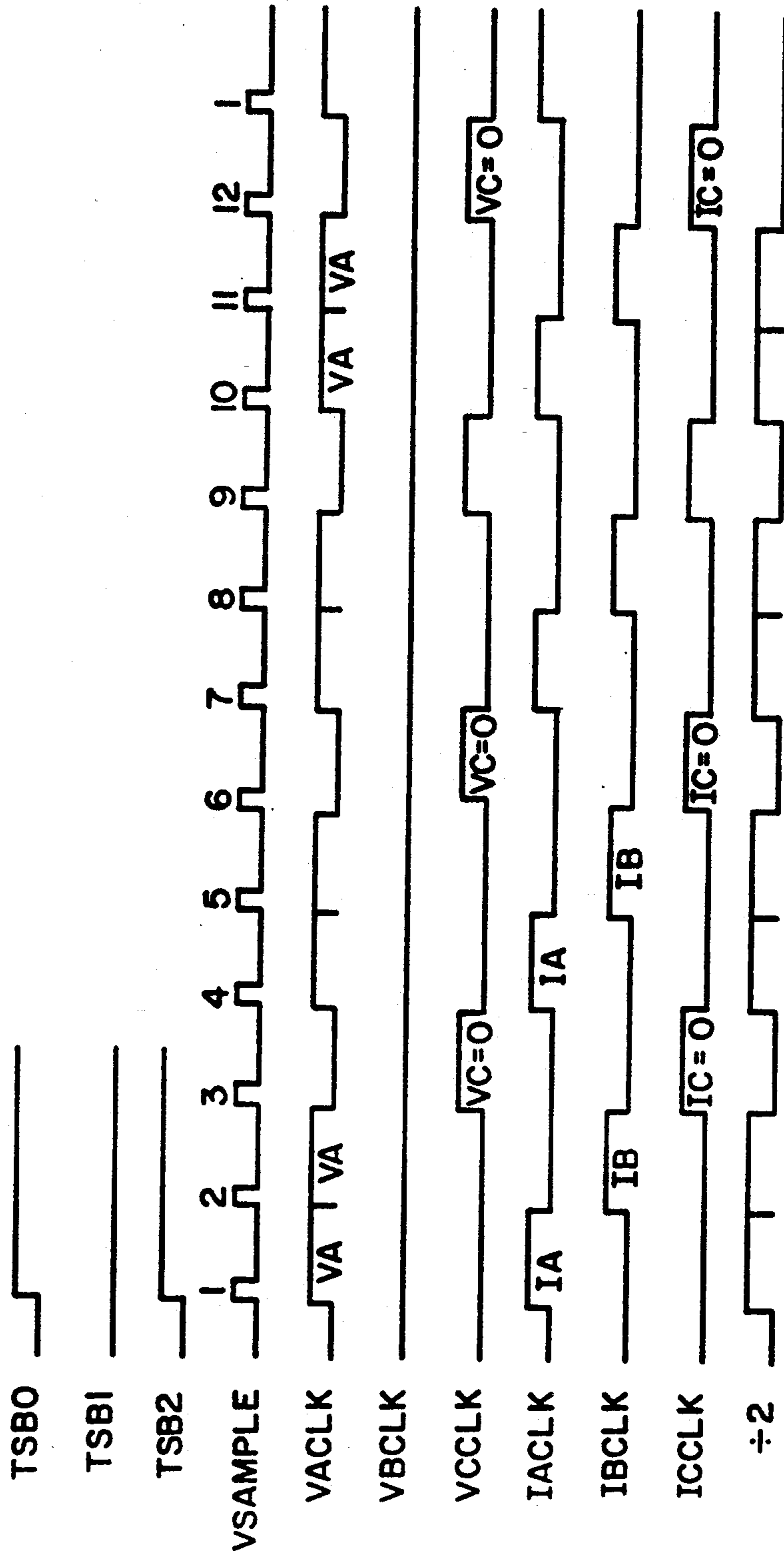
TIMING--TYPE 5 METER
