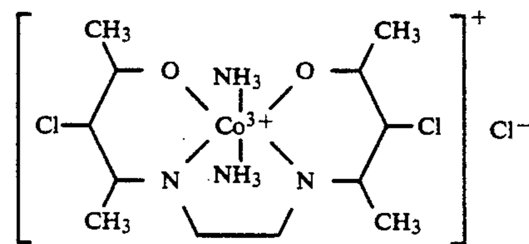
[\text{Co}(\text{L67})(\text{NH}_3)_2]\text{Cl}
