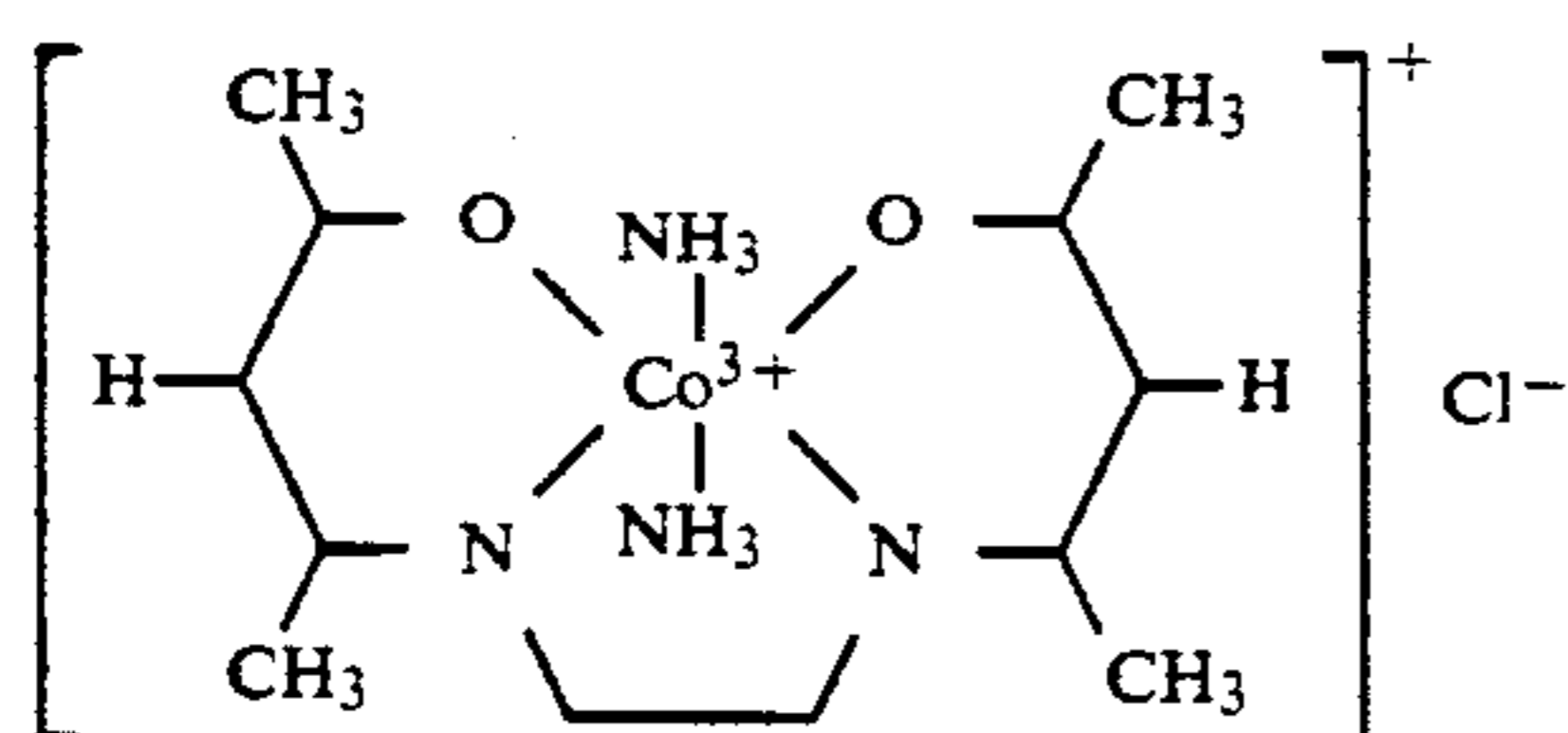
[\text{Co}(\text{L23})(\text{NH}_3)_2]\text{Cl}
