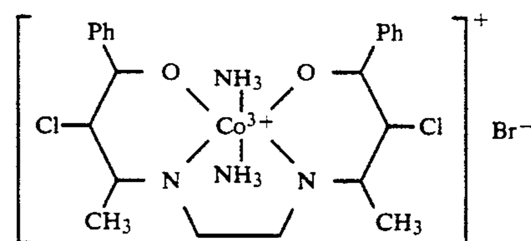
[\text{Co}(\text{L68})(\text{NH}_3)_2]\text{Br}
