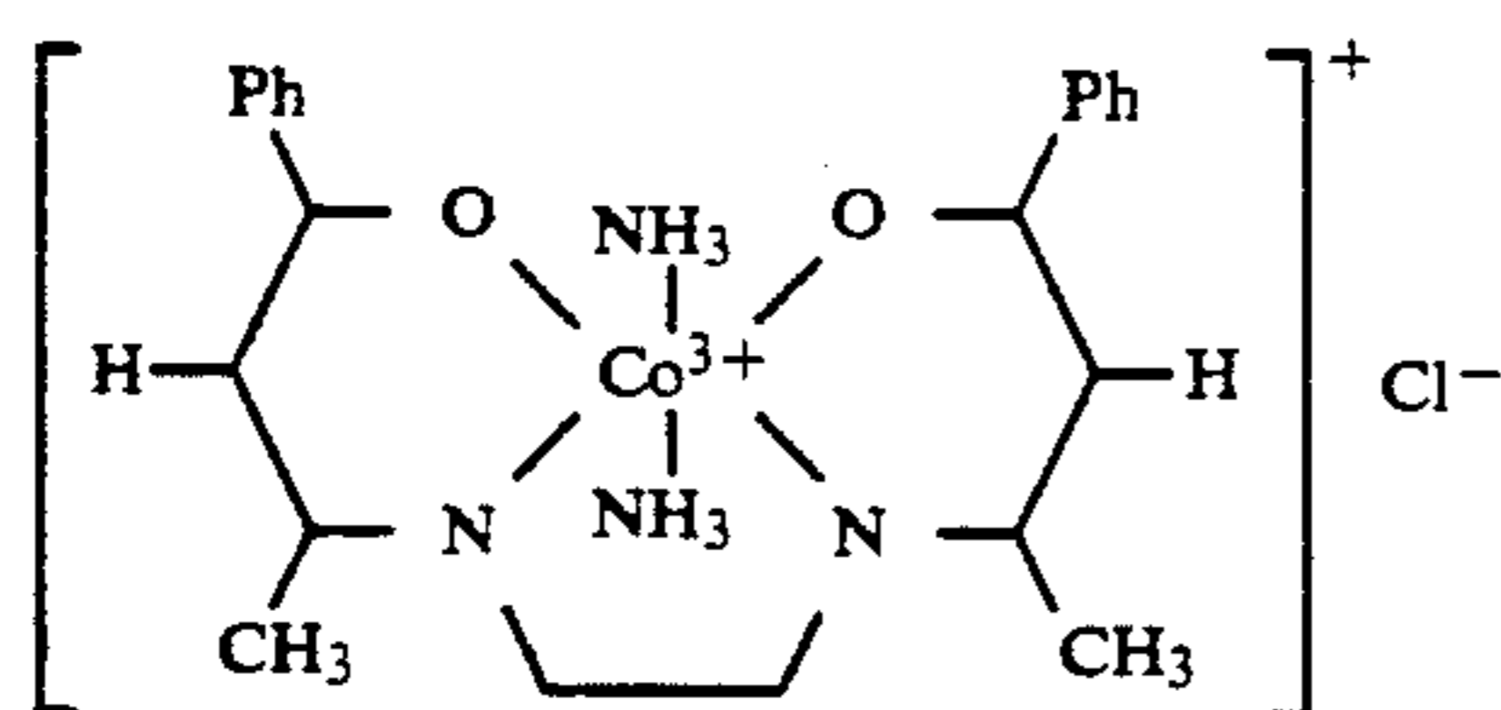
[\text{Co}(\text{L64})(\text{NH}_3)_2]\text{Cl}
