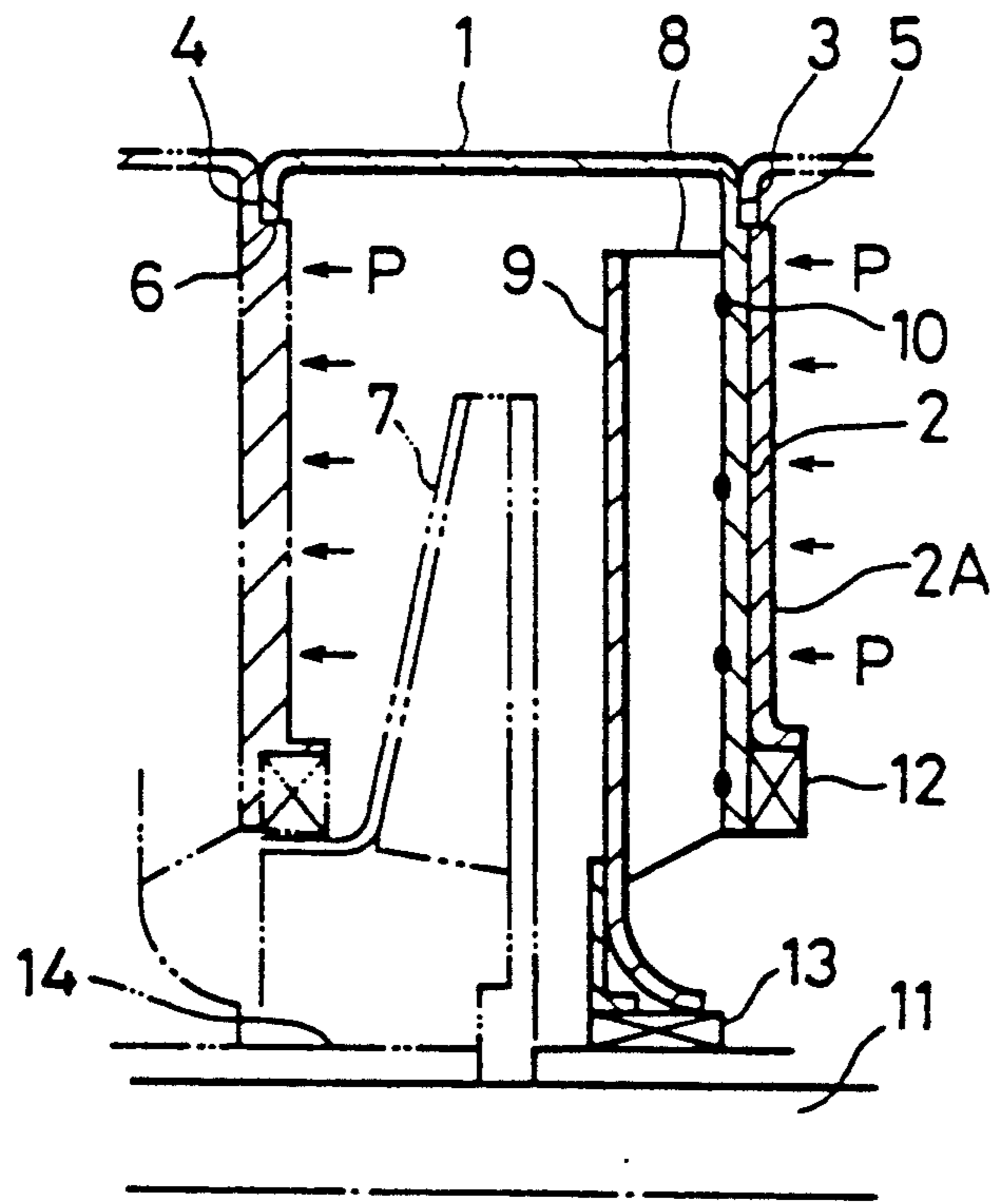
FIG. 2 - PRIOR ART
