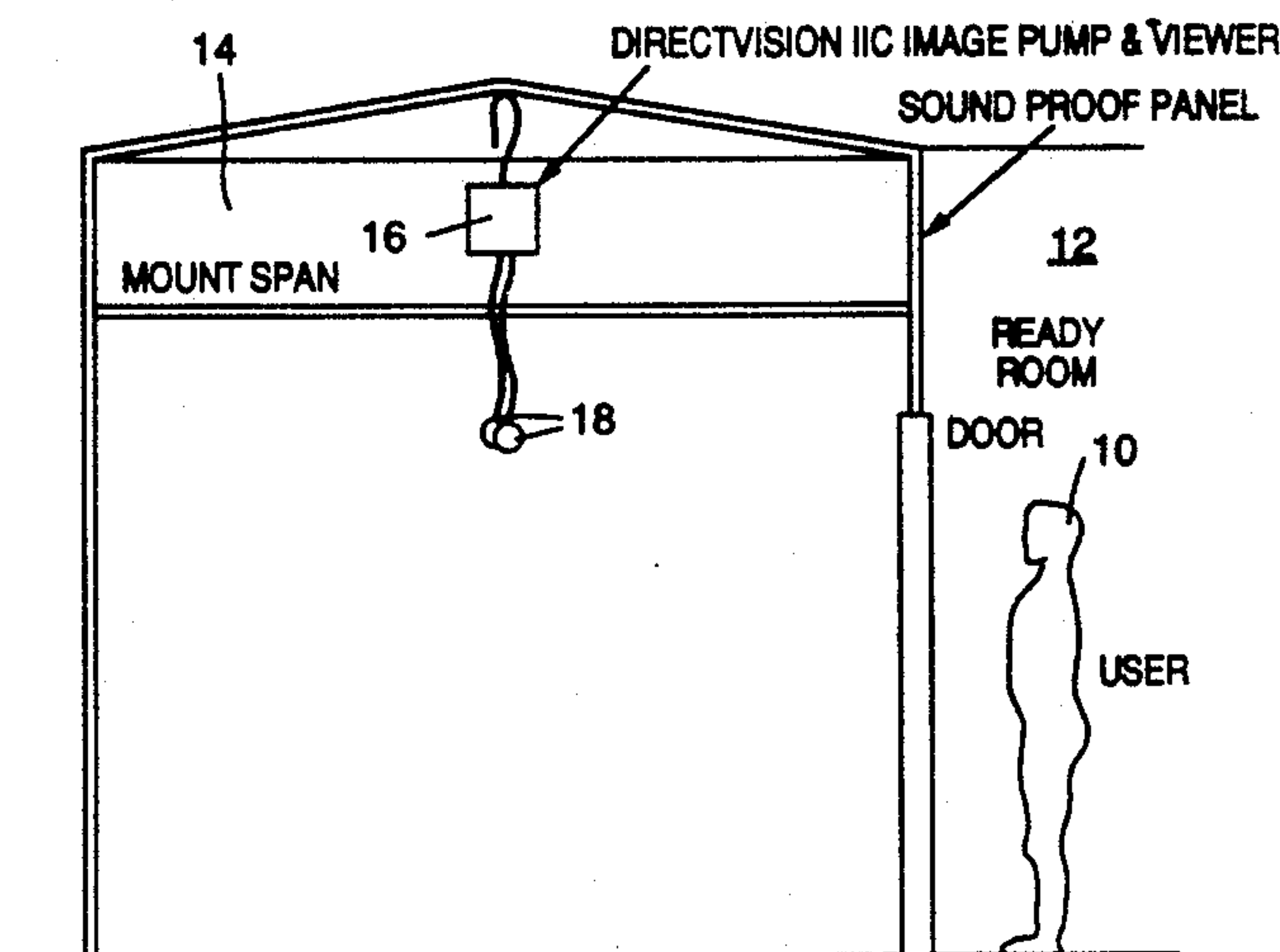
GENERAL LAYOUT, NOMINAL 10' X 10' VERITY CHAMBER
