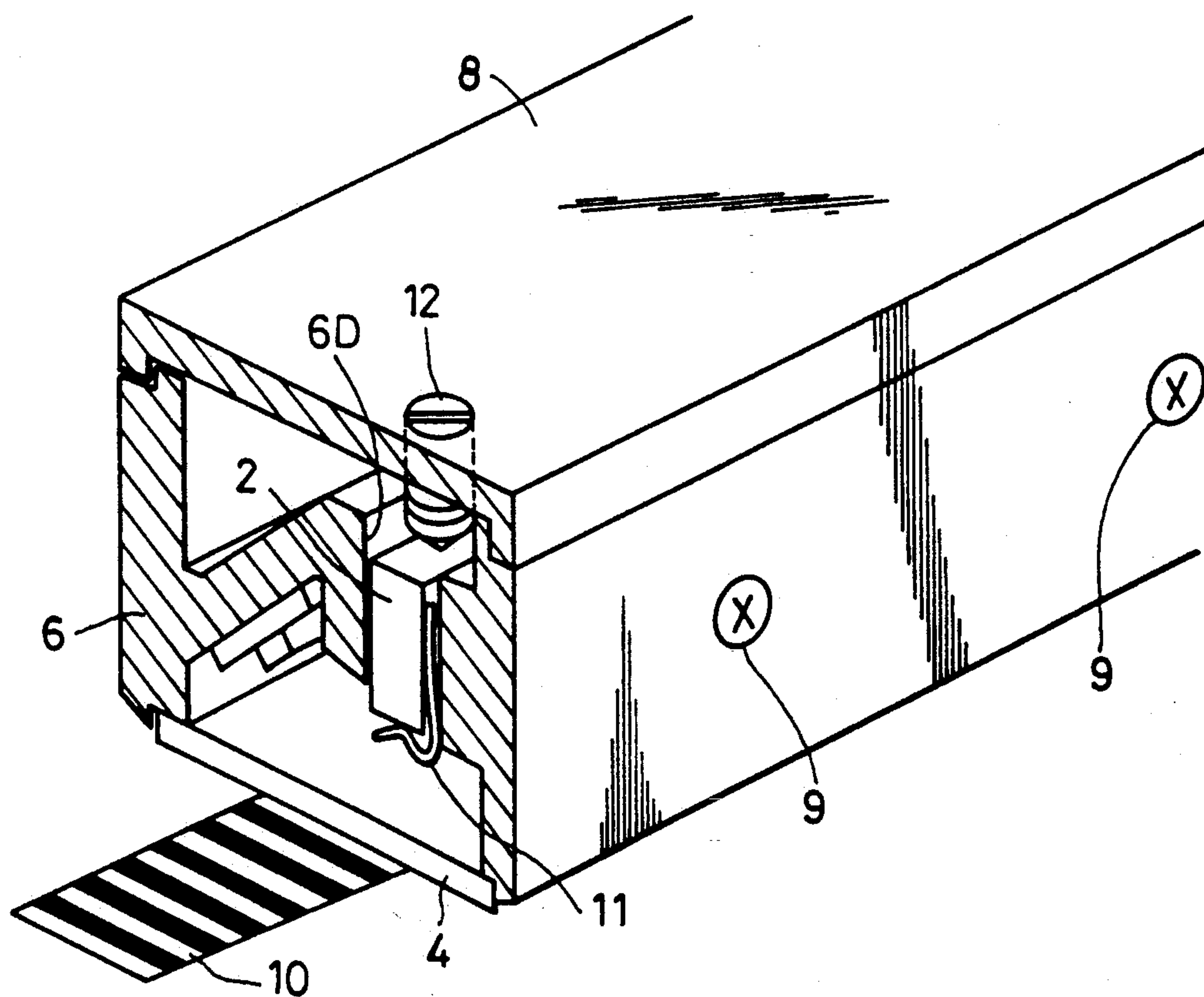
FIG. 2 PRIOR ART
