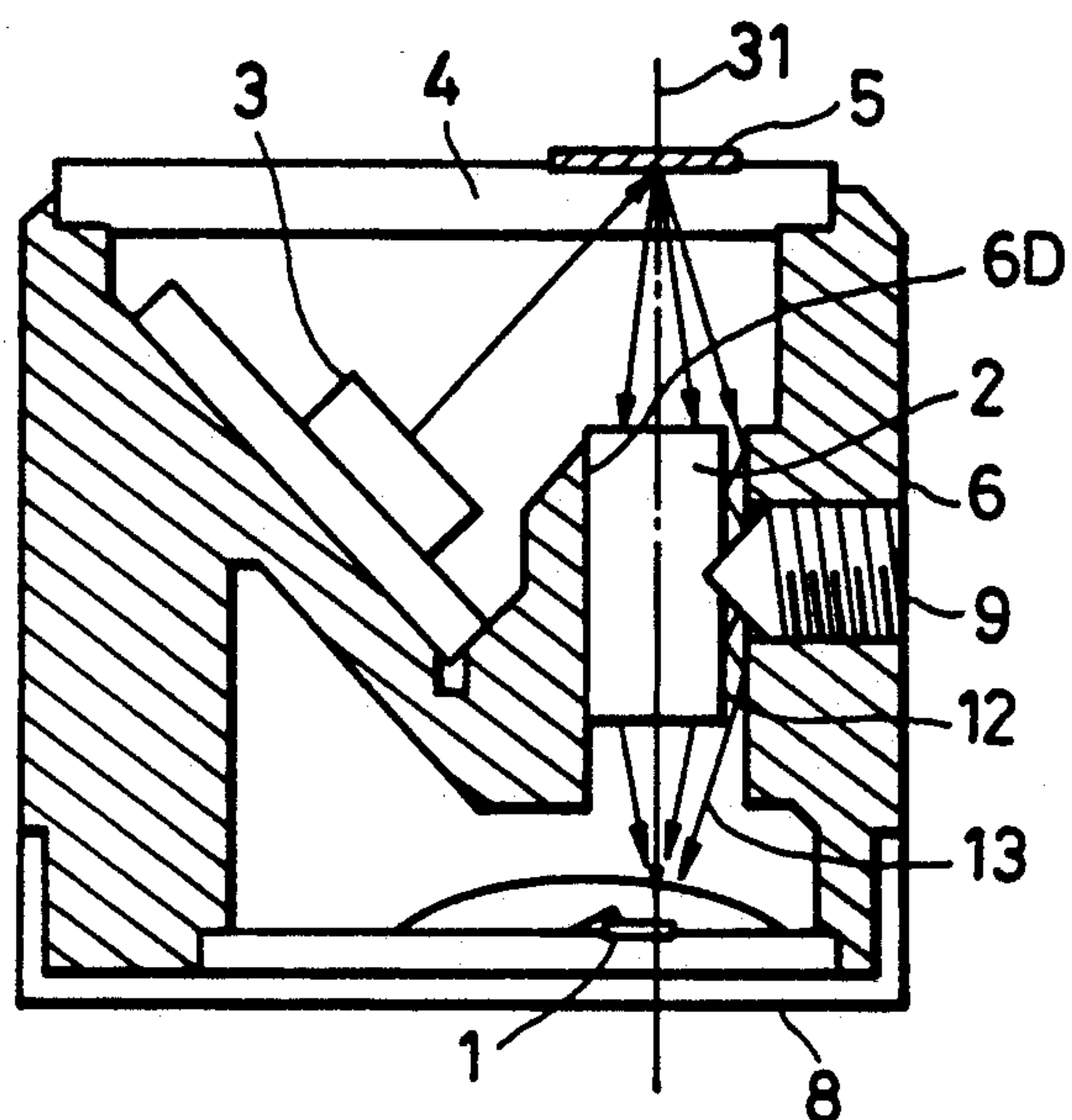
FIG. 1 PRIOR ART
