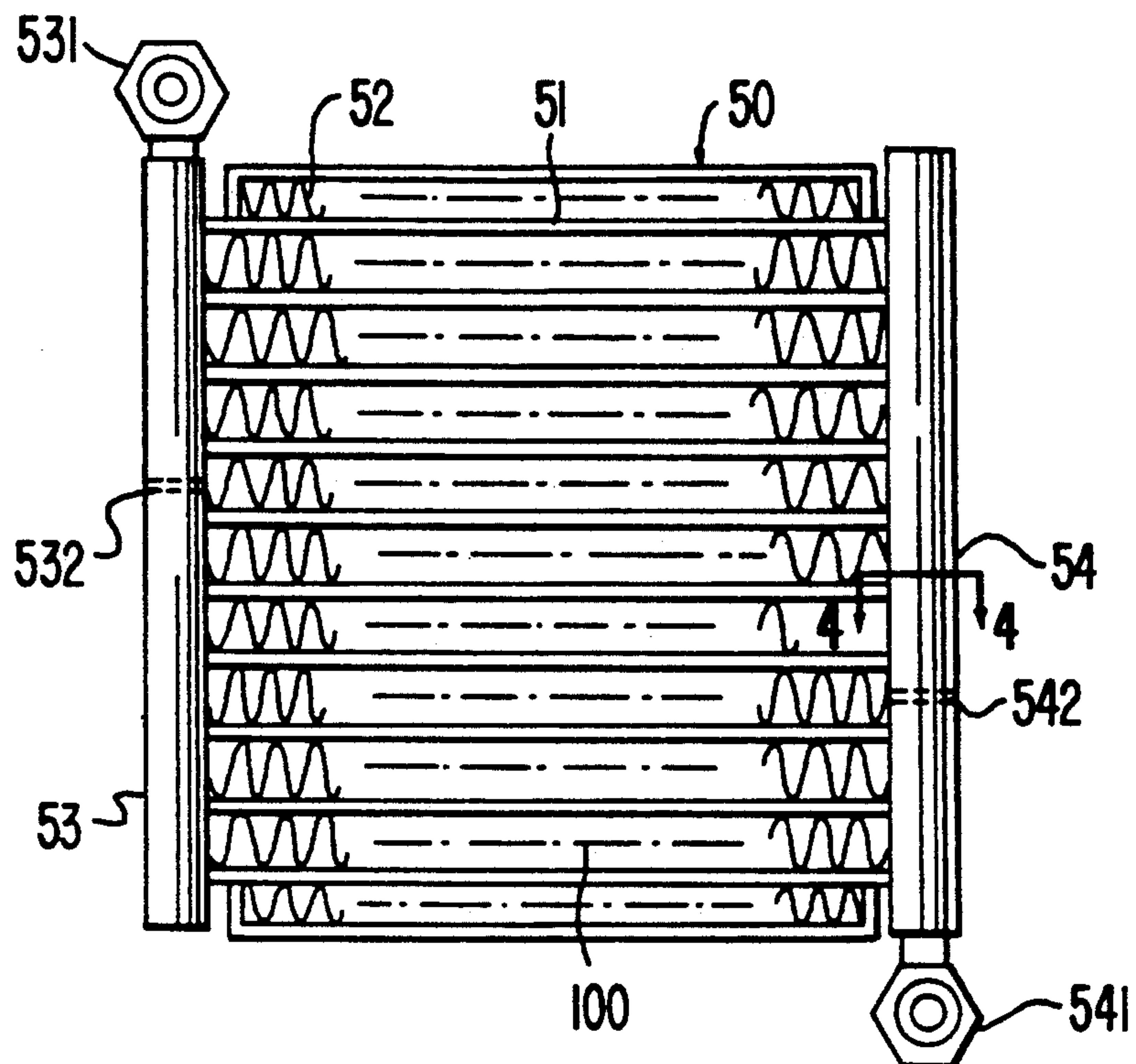
FIG. 2 (PRIOR ART)
