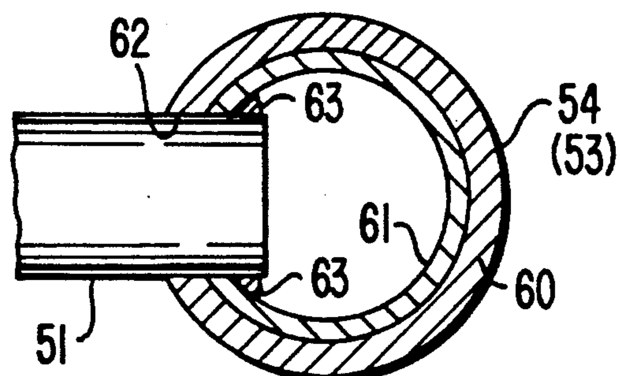
FIG. 3 (PRIOR ART)
