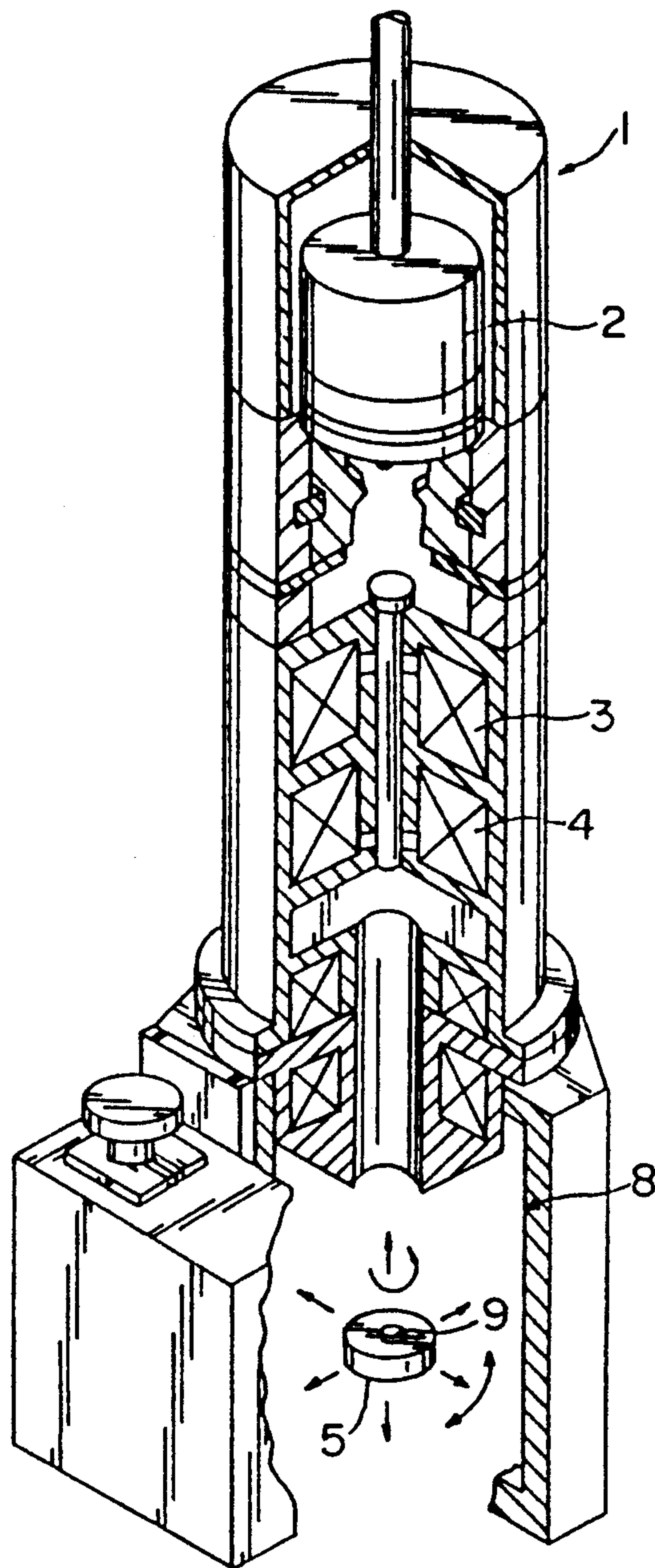
FIG. 1 PRIOR ART
