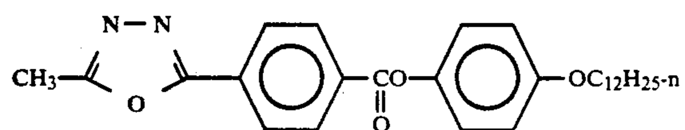
Formula (III-4)
