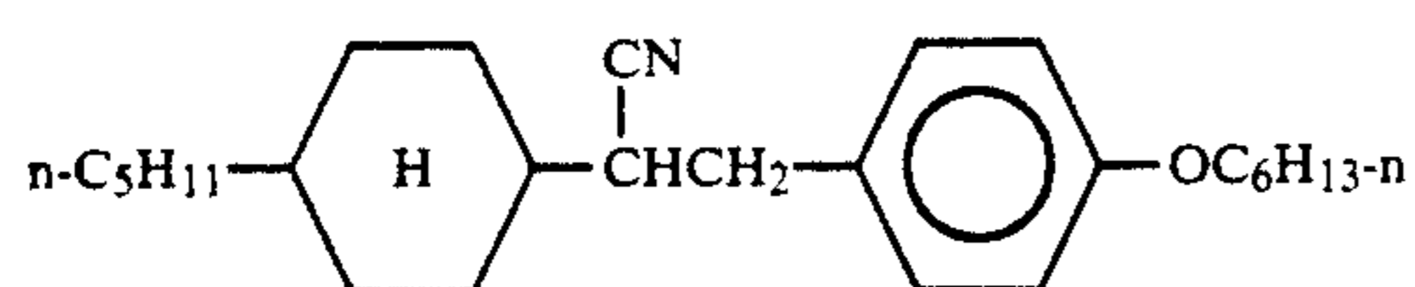
Formula (III-5)
