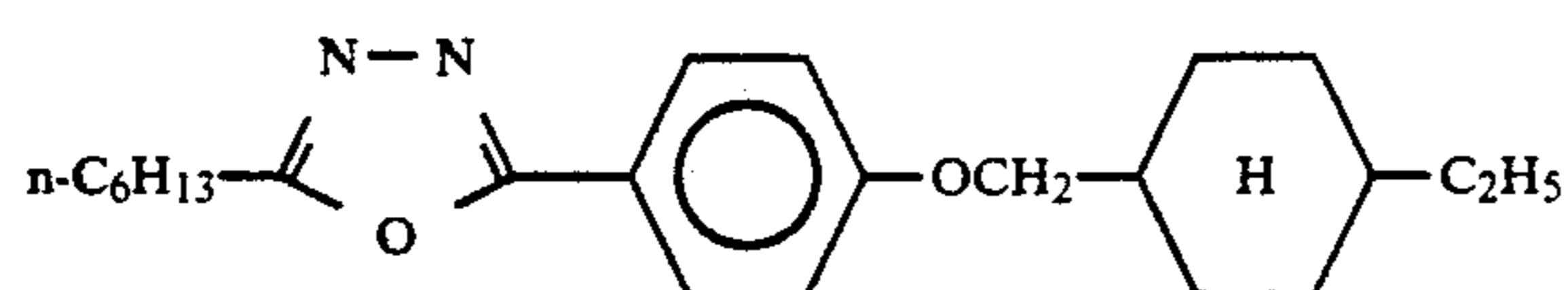
Formula (III-3)
